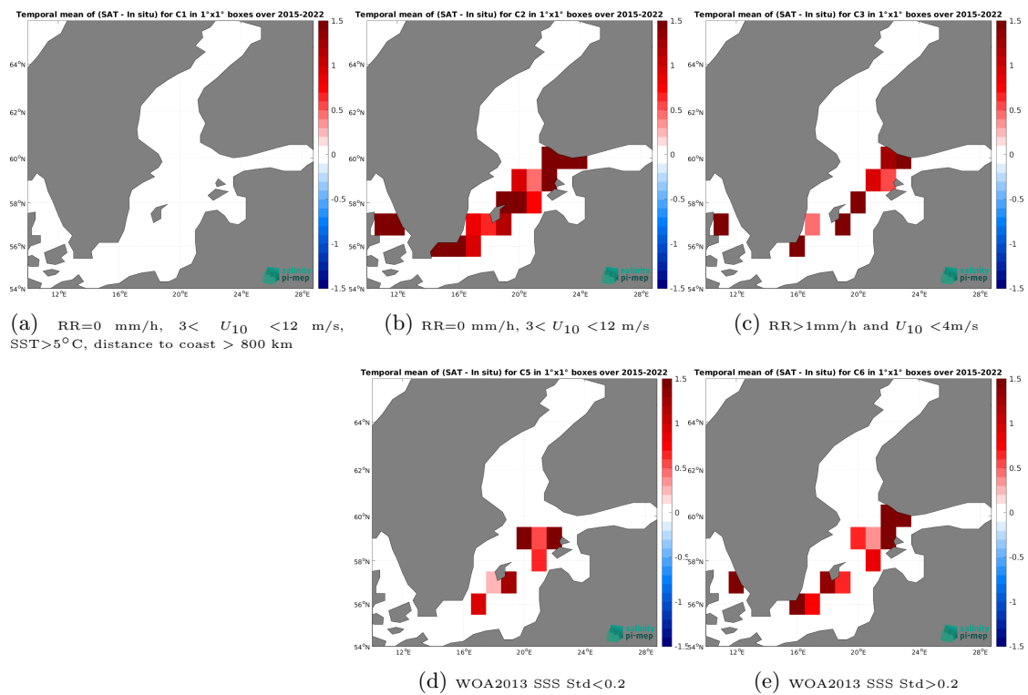
Figure 14: Temporal mean gridded over spatial boxes of size 1^\circ \times 1^\circ of \Delta SSS (SMAP SSS L3 v5.3 - 8-Day running (RSS) - TSG (LEGOS-DM)) for 5 different subdatasets corresponding to:RR=0 mm/h, 3 < U_{10} < 12 m/s, SST>5°C, distance to coast > 800 km (a), RR=0 mm/h, 3 < U_{10} < 12 m/s (b), RR>1mm/h and U_{10} < 4 m/s (c), WOA2013 SSS Std<0.2 (d), WOA2013 SSS Std>0.2 (e).
