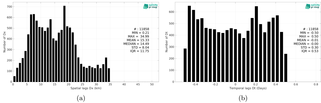
Figure 6: Histograms of the spatial (a) and temporal (b) lags between the location/time of the TSG (LEGOS-DM) measurement and the date of the corresponding SMAP SSS L3 v5.3 - 8-Day running (RSS) SSS pixel.
