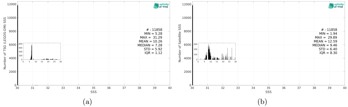
Figure 3: Histograms of SSS from TSG (LEGOS-DM) (a) and SMAP SSS L3 v5.3 - 8-Day running (RSS) (b) considering all match-up pairs per bins of 0.1 over the Baltic Sea Pi-MEP region and for the full satellite product period.
