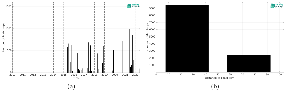
Figure 2: Number of match-ups between TSG (LEGOS-DM) and SMAP SSS L3 v5.3 - 8-Day running (RSS) SSS as a function of time (a) and as function of the distance to coast (b) over the Baltic Sea Pi-MEP region and for the full satellite product period.
