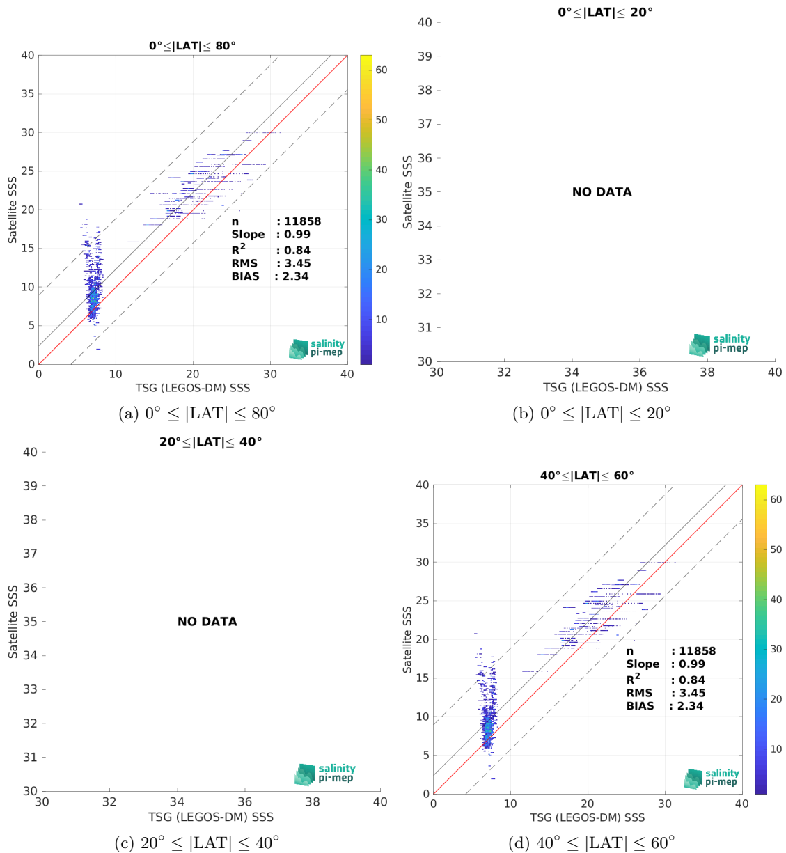
Figure 10: Contour maps of the concentration of SMAP SSS L3 v5.3 - 8-Day running (RSS) SSS (y-axis) versus TSG (LEGOS-DM) SSS (x-axis) at match-up pairs for different latitude bands. For each plot, the red line shows x=y . The black thin and dashed lines indicate a linear fit through the data cloud and the \pm 95\% confidence levels, respectively. The number match-up pairs n , the slope and R^2 coefficient of the linear fit, the root mean square (RMS) and the mean bias between satellite and in situ data are indicated for each latitude band in each plots.
