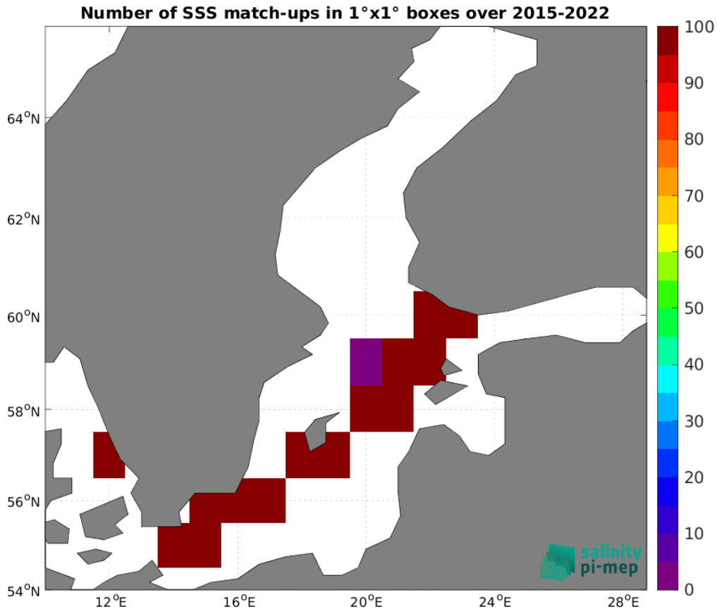
Figure 5: Number of SSS match-ups between TSG (LEGOS-DM) SSS and the SMAP SSS L3 v5.3 - Monthly (RSS) SSS product for the Baltic Sea Pi-MEP region over 1^\circ \times 1^\circ boxes and for the full satellite product period.
