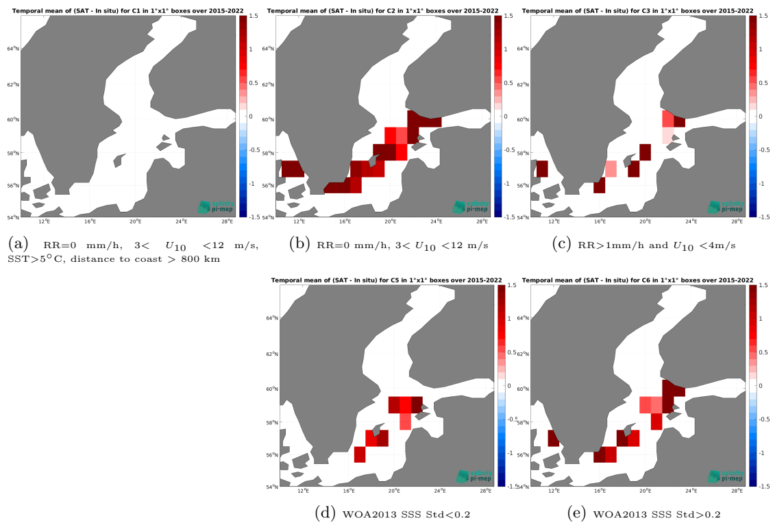
Figure 14: Temporal mean gridded over spatial boxes of size 1^\circ \times 1^\circ of \Delta\text{SSS} (SMAP SSS L3 v5.3 - Monthly (RSS) - TSG (LEGOS-DM)) for 5 different subdatasets corresponding to:RR=0 mm/h, 3 < U_{10} < 12 m/s, SST >5^\circ\text{C} , distance to coast > 800 km (a), RR=0 mm/h, 3 < U_{10} < 12 m/s (b), RR >1 mm/h and U_{10} < 4 m/s (c), WOA2013 SSS Std <0.2 (d), WOA2013 SSS Std >0.2 (e).
