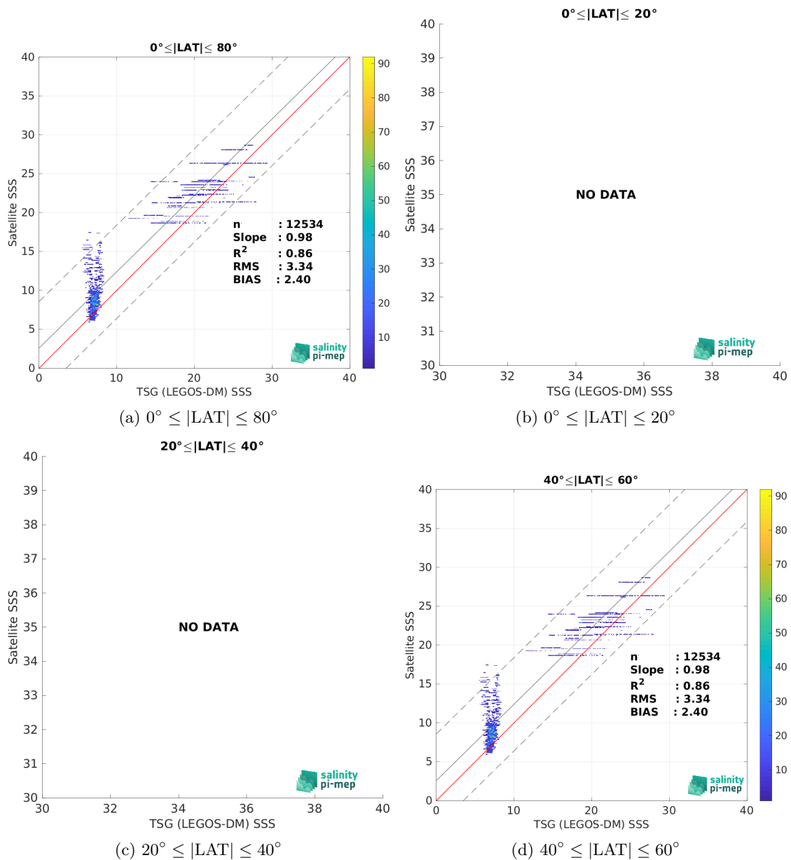
Figure 10: Contour maps of the concentration of SMAP SSS L3 v5.3 - Monthly (RSS) SSS (y-axis) versus TSG (LEGOS-DM) SSS (x-axis) at match-up pairs for different latitude bands. For each plot, the red line shows x=y . The black thin and dashed lines indicate a linear fit through the data cloud and the \pm 95\% confidence levels, respectively. The number match-up pairs n , the slope and R^2 coefficient of the linear fit, the root mean square (RMS) and the mean bias between satellite and in situ data are indicated for each latitude band in each plots.
