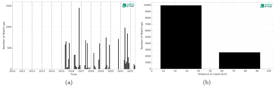
Figure 2: Number of match-ups between TSG (LEGOS-DM) and SMAP SSS L3 v5.3 - Monthly (RSS) SSS as a function of time (a) and as function of the distance to coast (b) over the Baltic Sea Pi-MEP region and for the full satellite product period.
