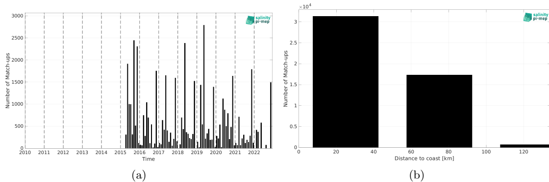
Figure 2: Number of match-ups between ICES and SMAP SSS L3 v5.3 - Monthly (RSS) SSS as a function of time (a) and as function of the distance to coast (b) over the Baltic Sea Pi-MEP region and for the full satellite product period.
