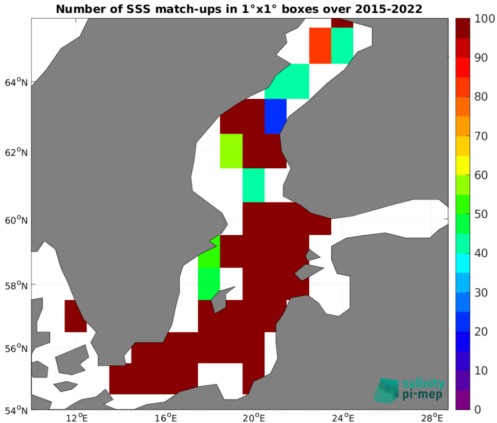
Figure 5: Number of SSS match-ups between ICES SSS and the SMAP SSS L3 v5.3 - Monthly (RSS) SSS product for the Baltic Sea Pi-MEP region over 1^\circ \times 1^\circ boxes and for the full satellite product period.
