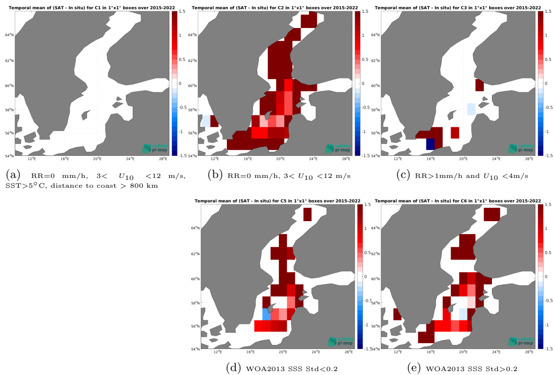
Figure 14: Temporal mean gridded over spatial boxes of size 1^\circ \times 1^\circ of \Delta SSS (SMAP SSS L3 v5.3 - Monthly (RSS) - ICES) for 5 different subdatasets corresponding to:RR=0 mm/h, 3 < U_{10} < 12 m/s, SST >5^\circ\text{C} , distance to coast > 800 km (a), RR=0 mm/h, 3 < U_{10} < 12 m/s (b), RR >1 mm/h and U_{10} < 4 m/s (c), WOA2013 SSS Std <0.2 (d), WOA2013 SSS Std >0.2 (e).
