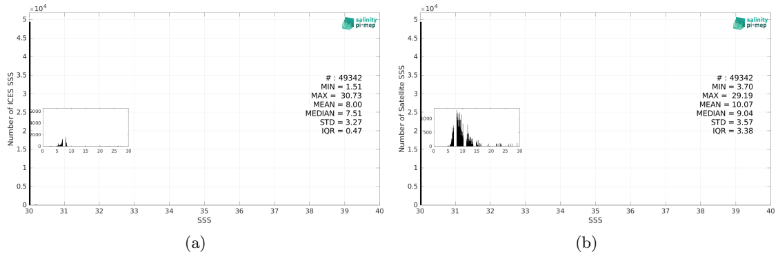
Figure 3: Histograms of SSS from ICES (a) and SMAP SSS L3 v5.3 - Monthly (RSS) (b) considering all match-up pairs per bins of 0.1 over the Baltic Sea Pi-MEP region and for the full satellite product period.
