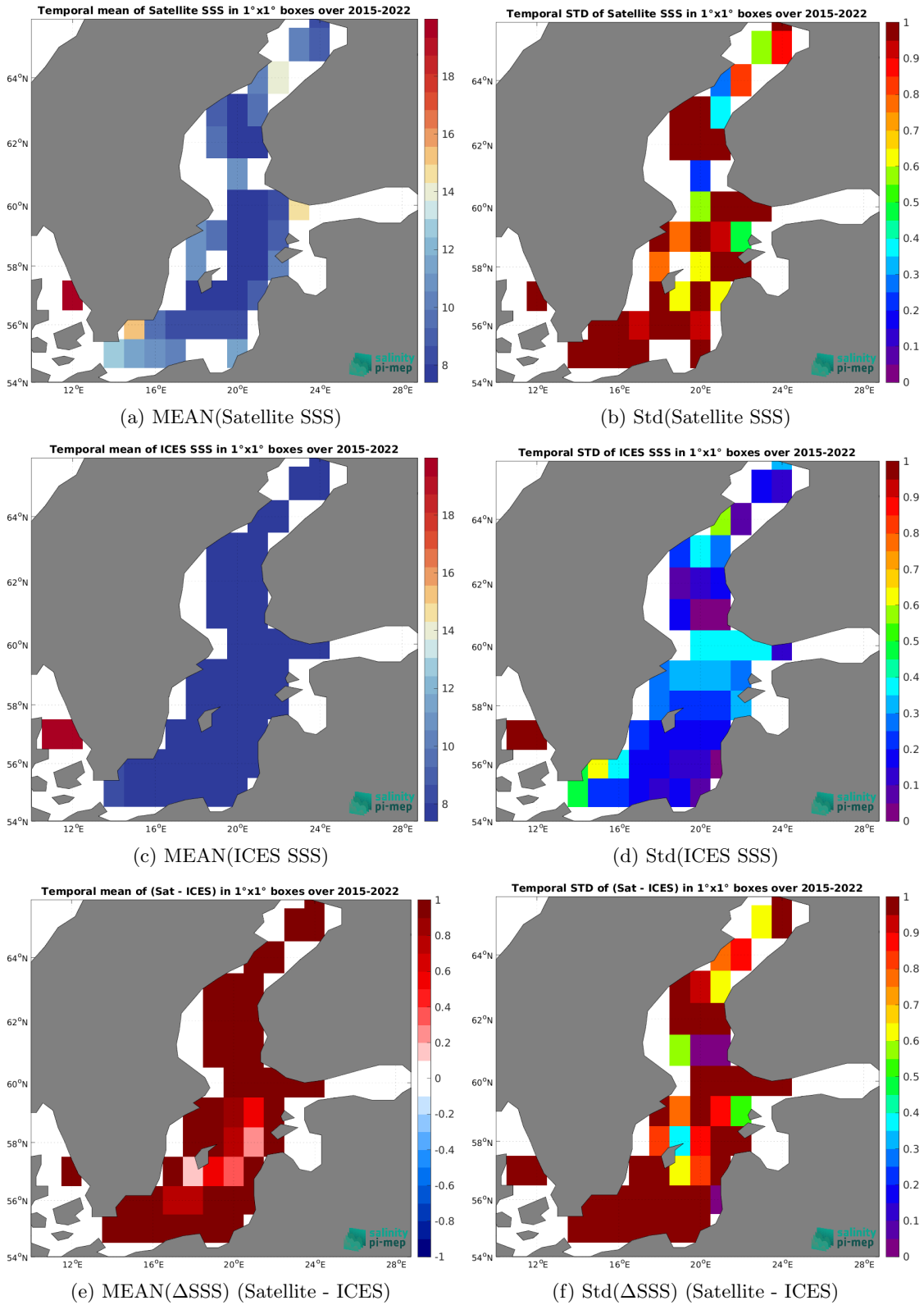
Figure 7: Temporal mean (left) and Std (right) of SSS from SMAP SSS L3 v5.3 - Monthly (RSS) (top), ICES (middle), and of \Delta SSS (Satellite - ICES). Only match-up pairs are used to generate these maps.
