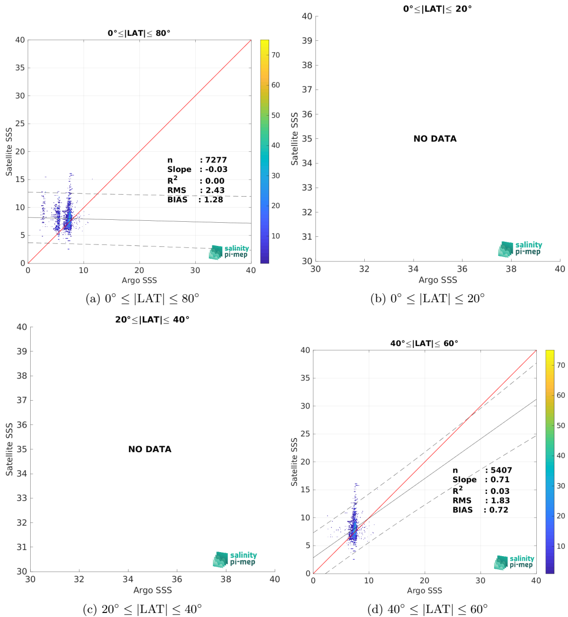
Figure 10: Contour maps of the concentration of SMAP SSS L3 v5.3 - Monthly (RSS) SSS (y-axis) versus Argo SSS (x-axis) at match-up pairs for different latitude bands. For each plot, the red line shows x=y . The black thin and dashed lines indicate a linear fit through the data cloud and the \pm 95\% confidence levels, respectively. The number match-up pairs n , the slope and R^2 coefficient of the linear fit, the root mean square (RMS) and the mean bias between satellite and in situ data are indicated for each latitude band in each plots.
