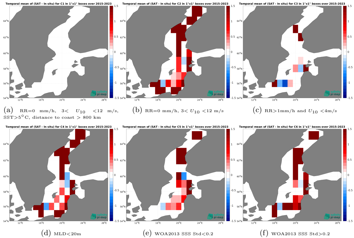
Figure 14: Temporal mean gridded over spatial boxes of size 1^\circ \times 1^\circ of \Delta SSS (SMAP SSS L3 v5.3 - Monthly (RSS) - Argo) for 6 different subdatasets corresponding to:RR=0 mm/h, 3 < U_{10} < 12 m/s, SST>5°C, distance to coast > 800 km (a), RR=0 mm/h, 3 < U_{10} < 12 m/s (b), RR>1mm/h and U_{10} < 4 m/s (c),MLD<20m (d),WOA2013 SSS Std<0.2 (e),WOA2013 SSS Std>0.2 (f).
