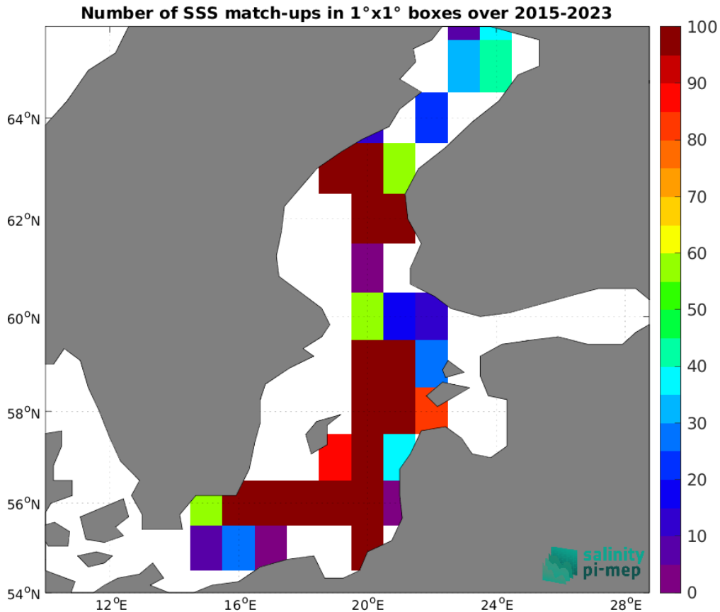
Figure 5: Number of SSS match-ups between Argo SSS and the SMAP SSS L3 v5.3 - Monthly (RSS) SSS product for the Baltic Sea Pi-MEP region over 1^\circ \times 1^\circ boxes and for the full satellite product period.
