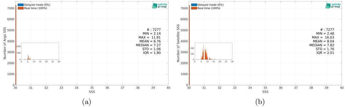
Figure 3: Histograms of SSS from Argo (a) and SMAP SSS L3 v5.3 - Monthly (RSS) (b) considering all match-up pairs per bins of 0.1 over the Baltic Sea Pi-MEP region and for the full satellite product period.
