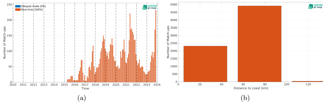
Figure 2: Number of match-ups between Argo and SMAP SSS L3 v5.3 - Monthly (RSS) SSS as a function of time (a) and as function of the distance to coast (b) over the Baltic Sea Pi-MEP region and for the full satellite product period.
