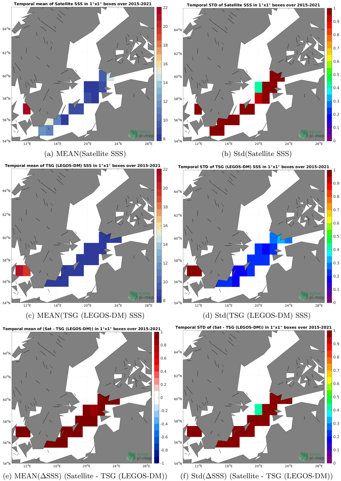
Figure 6: Temporal mean (left) and Std (right) of SSS from SMAP SSS L3 v5 - 8-Day running (RSS) (top), TSG (LEGOS-DM) (middle), and of \Delta SSS (Satellite - TSG (LEGOS-DM)). Only match-up pairs are used to generate these maps.
