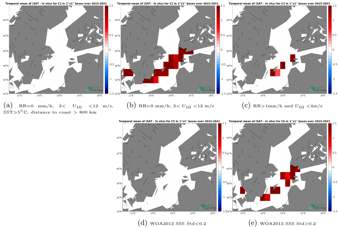
Figure 12: Temporal mean gridded over spatial boxes of size 1^{\circ}\times 1^{\circ} of \Delta\text{SSS} (SMAP SSS L3 v5 - 8-Day running (RSS) - TSG (LEGOS-DM)) for 5 different subdatasets corresponding to: \text{RR}=0 mm/h, 3 < U_{10} < 12 m/s, \text{SST} > 5^{\circ}\text{C} , distance to coast > 800 km (a), \text{RR}=0 mm/h, 3 < U_{10} < 12 m/s (b), \text{RR} > 1\text{mm/h} and U_{10} < 4\text{m/s} (c), WOA2013 SSS Std < 0.2 (d), WOA2013 SSS Std > 0.2 (e).
