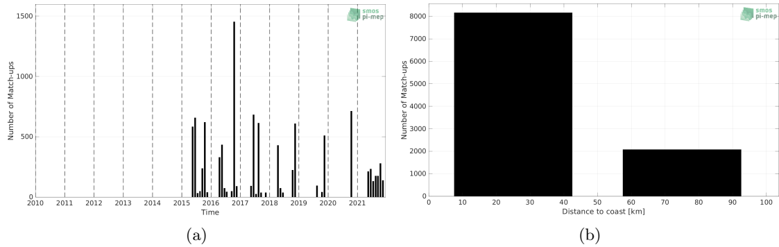
Figure 1: Number of match-ups between TSG (LEGOS-DM) and SMAP SSS L3 v5 - 8-Day running (RSS) SSS as a function of time (a) and as function of the distance to coast (b) over the Baltic Sea Pi-MEP region and for the full satellite product period.
