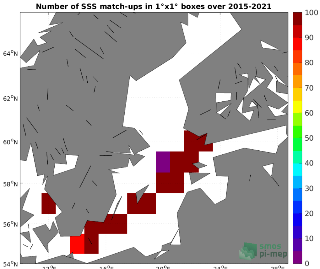
Figure 4: Number of SSS match-ups between TSG (LEGOS-DM) SSS and the SMAP SSS L3 v5 - 8-Day running (RSS) SSS product for the Baltic Sea Pi-MEP region over 1°×1° boxes and for the full satellite product period.
