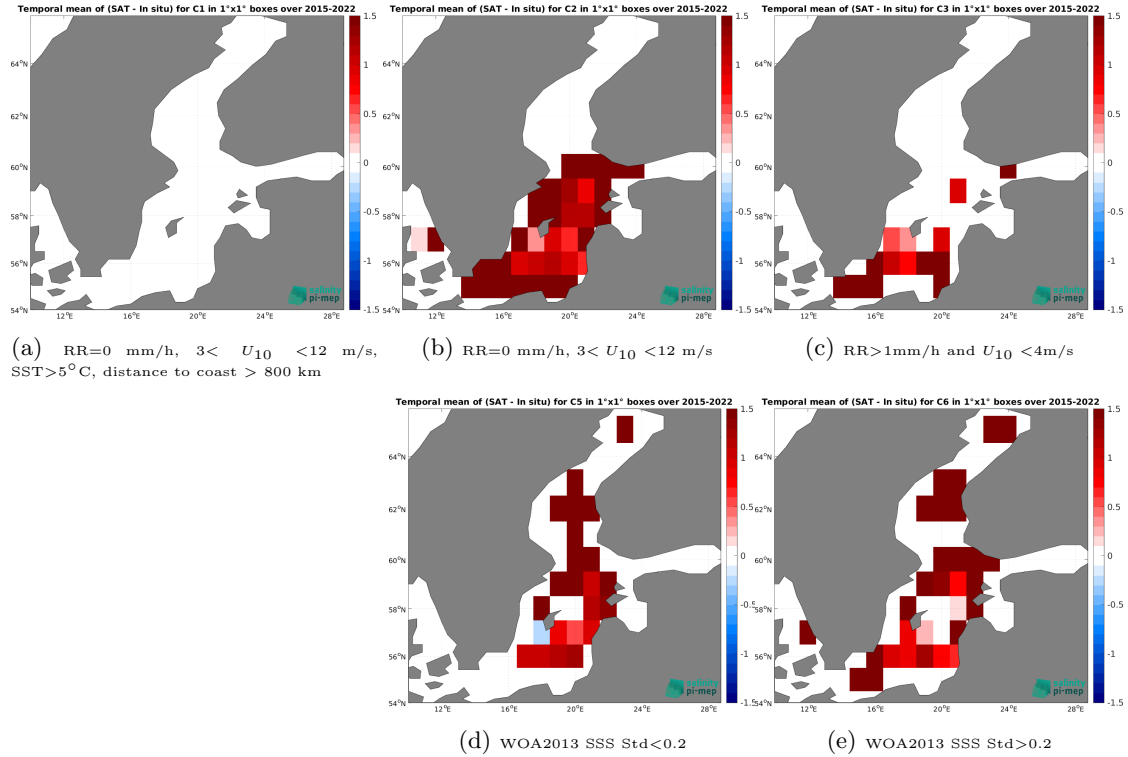
Figure 12: Temporal mean gridded over spatial boxes of size 1^{\circ}\times 1^{\circ} of \Delta\text{SSS} (SMAP SSS L3 v5 - 8-Day running (RSS) - ICES) for 5 different subdatasets corresponding to: \text{RR}=0 mm/h, 3 < U_{10} < 12 m/s, \text{SST} > 5^{\circ}\text{C} , distance to coast > 800 km (a), \text{RR}=0 mm/h, 3 < U_{10} < 12 m/s (b), \text{RR} > 1\text{mm/h} and U_{10} < 4\text{m/s} (c), WOA2013 SSS Std < 0.2 (d), WOA2013 SSS Std > 0.2 (e).
