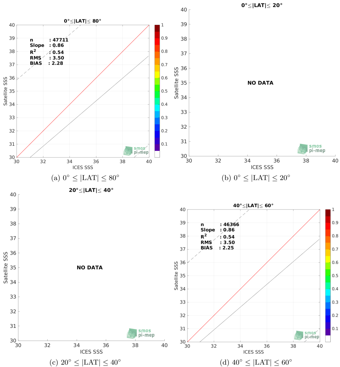
Figure 9: Contour maps of the concentration of SMAP SSS L3 v5 - 8-Day running (RSS) SSS (y-axis) versus ICES SSS (x-axis) at match-up pairs for different latitude bands. For each plot, the red line shows x=y . The black thin and dashed lines indicate a linear fit through the data cloud and the \pm 95\% confidence levels, respectively. The number match-up pairs n , the slope and R^2 coefficient of the linear fit, the root mean square (RMS) and the mean bias between satellite and in situ data are indicated for each latitude band in each plots.
