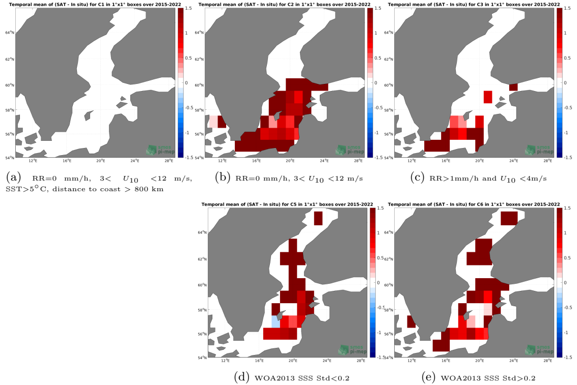
Figure 12: Temporal mean gridded over spatial boxes of size 1^{\circ}\times 1^{\circ} of \Delta\text{SSS} (SMAP SSS L3 v5 - 8-Day running (RSS) - ICES) for 5 different subdatasets corresponding to:RR=0 mm/h, 3 < U_{10} < 12 m/s, SST >5^{\circ}\text{C} , distance to coast > 800 km (a), RR=0 mm/h, 3 < U_{10} < 12 m/s (b), RR >1 mm/h and U_{10} < 4 m/s (c), WOA2013 SSS Std <0.2 (d), WOA2013 SSS Std >0.2 (e).
