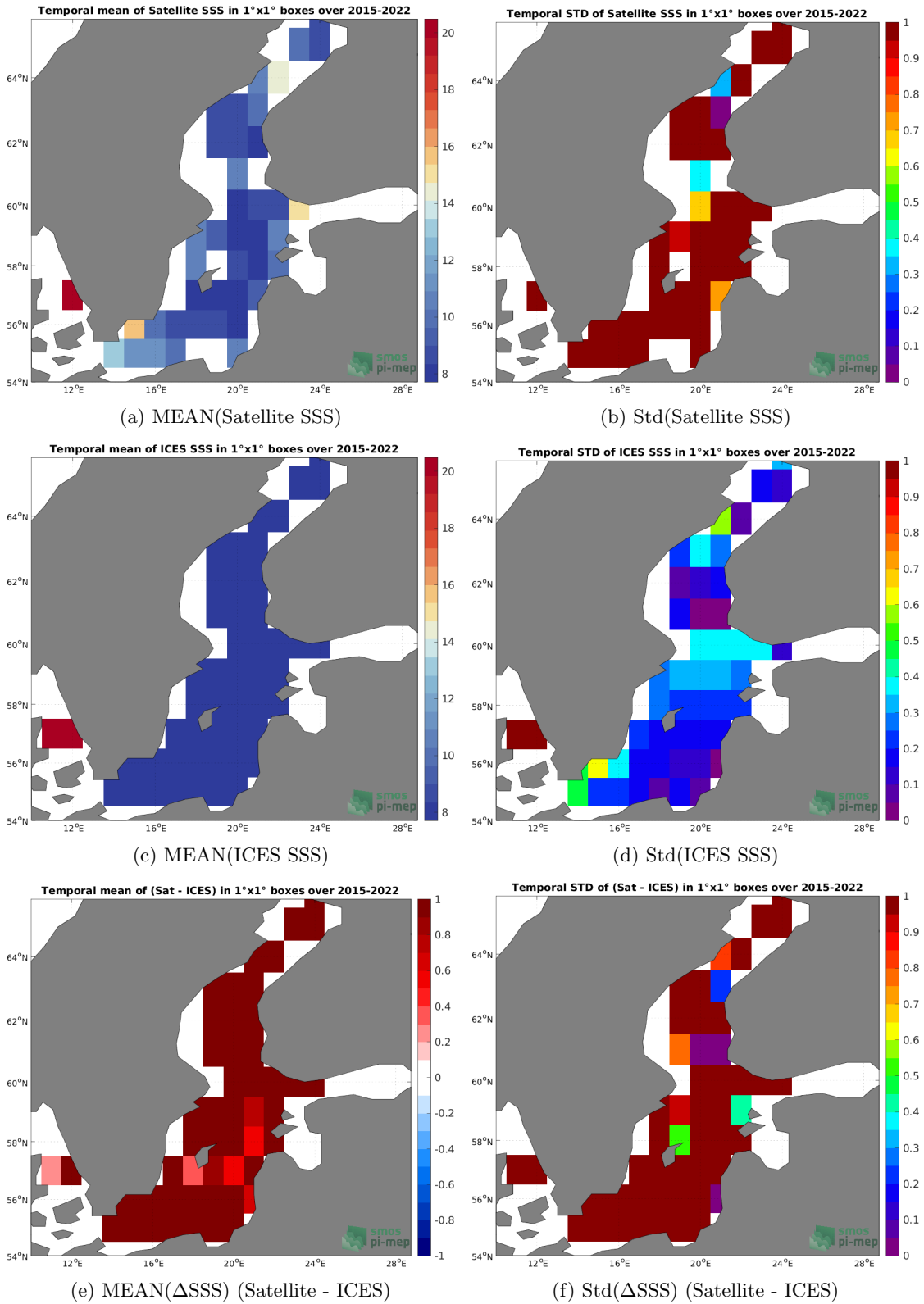
Figure 6: Temporal mean (left) and Std (right) of SSS from SMAP SSS L3 v5 - 8-Day running (RSS) (top), ICES (middle), and of \Delta SSS (Satellite - ICES). Only match-up pairs are used to generate these maps.
