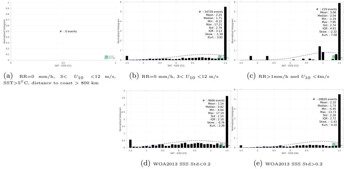
Figure 13: Normalized histogram of \Delta SSS (SMAP SSS L3 v5 - 8-Day running (RSS) - ICES) for 5 different subdatasets corresponding to: RR=0 mm/h, 3 < U_{10} < 12 m/s, SST > 5°C, distance to coast > 800 km (a), RR=0 mm/h, 3 < U_{10} < 12 m/s (b), RR > 1mm/h and U_{10} < 4 m/s (c), WOA2013 SSS Std < 0.2 (d), WOA2013 SSS Std > 0.2 (e).
