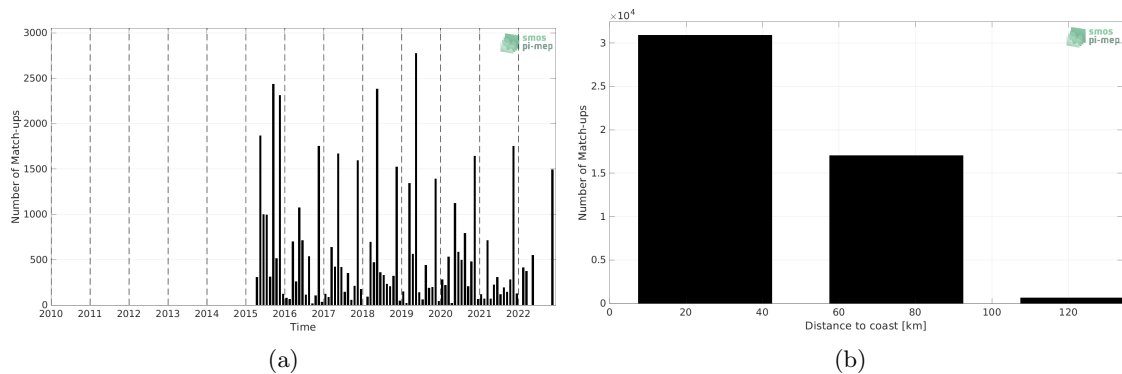
Figure 1: Number of match-ups between ICES and SMAP SSS L3 v5 - 8-Day running (RSS) SSS as a function of time (a) and as function of the distance to coast (b) over the Baltic Sea Pi-MEP region and for the full satellite product period.
