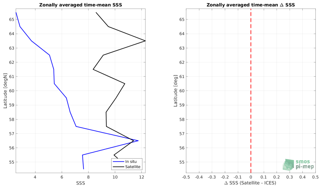
Figure 8: Left panel: Zonal mean SSS from SMAP SSS L3 v5 - 8-Day running (RSS) satellite product (black) and from ICES (blue). Right panel: Zonal mean of \Delta SSS (Satellite - ICES) for all the collected Pi-MEP match-up pairs estimated over the full satellite product period.
