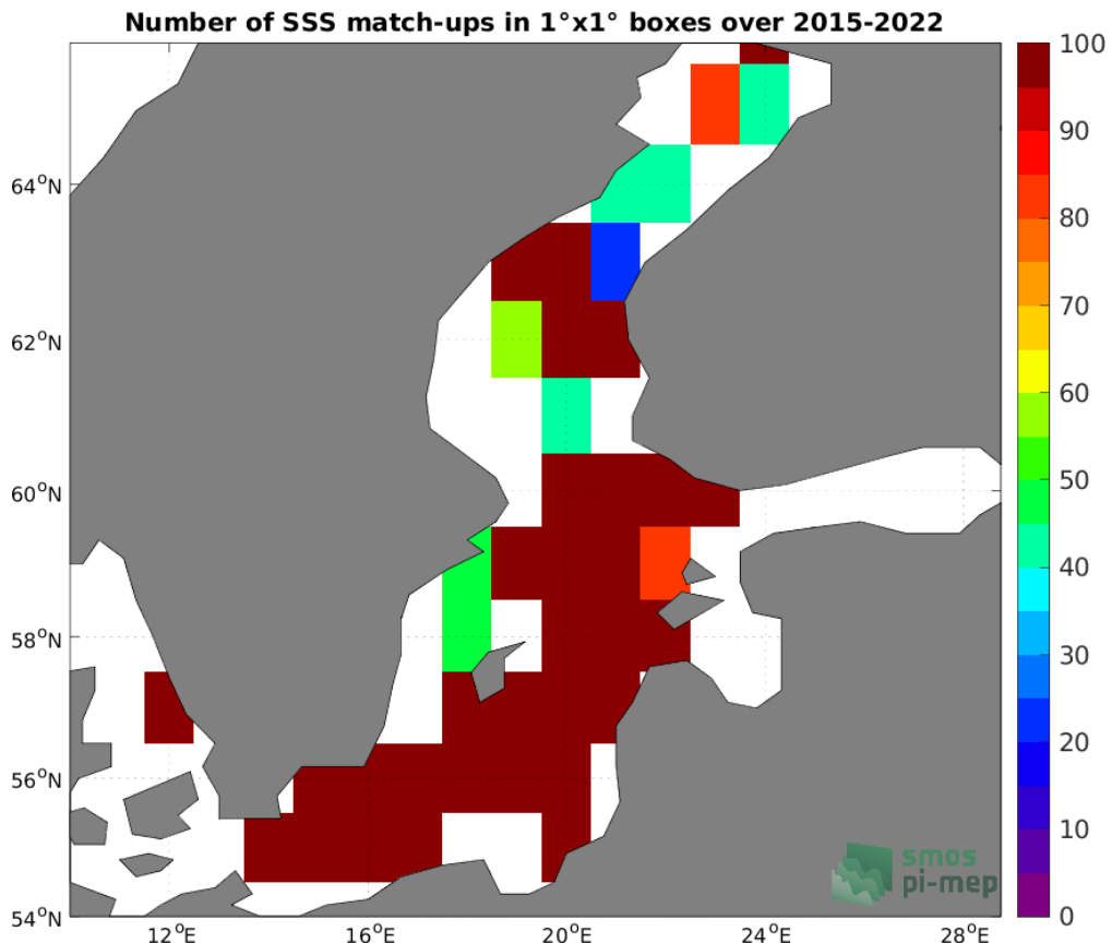
Figure 4: Number of SSS match-ups between ICES SSS and the SMAP SSS L3 v5 - 8-Day running (RSS) SSS product for the Baltic Sea Pi-MEP region over 1^\circ \times 1^\circ boxes and for the full satellite product period.
