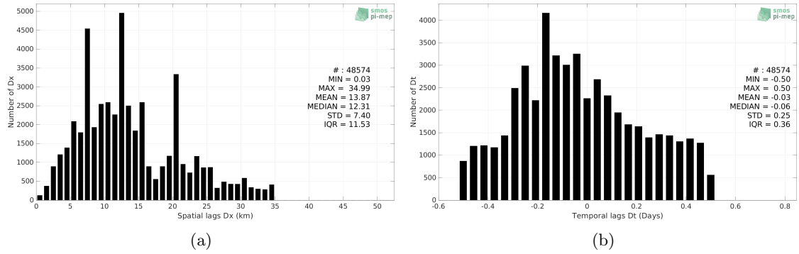
Figure 5: Histograms of the spatial (a) and temporal (b) lags between the location/time of the ICES measurement and the date of the corresponding SMAP SSS L3 v5 - 8-Day running (RSS) SSS pixel.
