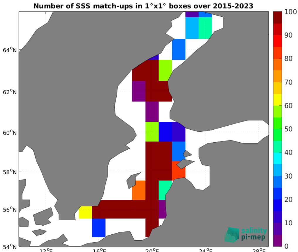
Figure 4: Number of SSS match-ups between Argo SSS and the SMAP SSS L3 v5 - 8-Day running (RSS) SSS product for the Baltic Sea Pi-MEP region over 1^\circ \times 1^\circ boxes and for the full satellite product period.
