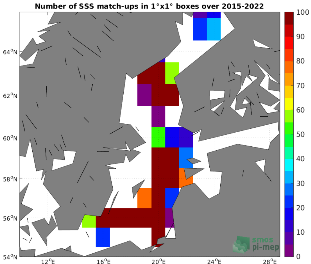
Figure 4: Number of SSS match-ups between Argo SSS and the SMAP SSS L3 v5 - 8-Day running (RSS) SSS product for the Baltic Sea Pi-MEP region over 1°×1° boxes and for the full satellite product period.
