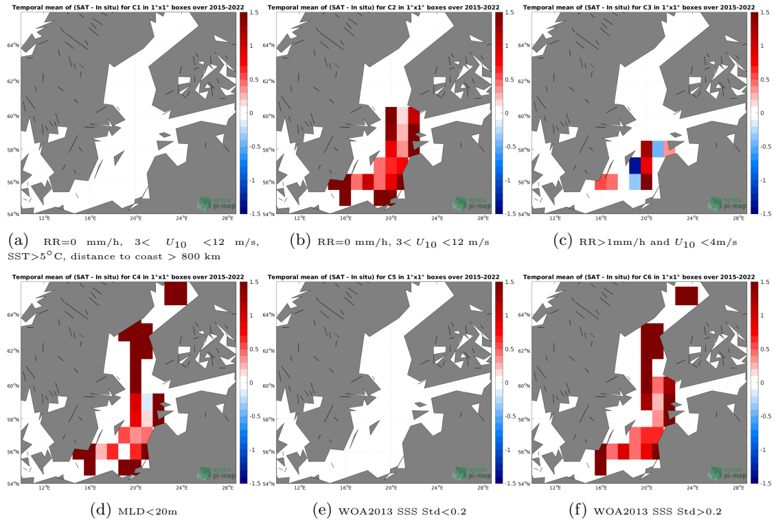
Figure 12: Temporal mean gridded over spatial boxes of size 1^{\circ}\times 1^{\circ} of \Delta\text{SSS} (SMAP SSS L3 v5 - 8-Day running (RSS) - Argo) for 6 different subdatasets corresponding to:RR=0 mm/h, 3 < U_{10} < 12 m/s, SST >5^{\circ}\text{C} , distance to coast > 800 km (a), RR=0 mm/h, 3 < U_{10} < 12 m/s (b), RR >1 mm/h and U_{10} < 4 m/s (c),MLD <20 m (d),WOA2013 SSS Std <0.2 (e),WOA2013 SSS Std >0.2 (f).
