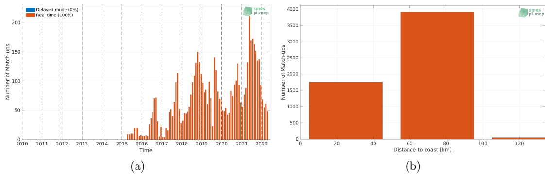
Figure 1: Number of match-ups between Argo and SMAP SSS L3 v5 - 8-Day running (RSS) SSS as a function of time (a) and as function of the distance to coast (b) over the Baltic Sea Pi-MEP region and for the full satellite product period.
