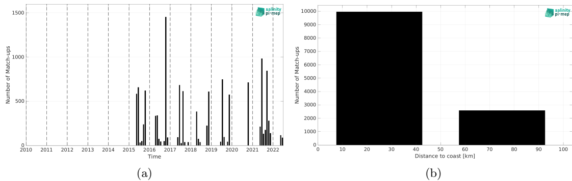
Figure 1: Number of match-ups between TSG (LEGOS-DM) and SMAP SSS L3 v5 - Monthly (RSS) SSS as a function of time (a) and as function of the distance to coast (b) over the Baltic Sea Pi-MEP region and for the full satellite product period.
