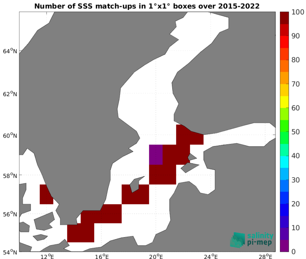
Figure 4: Number of SSS match-ups between TSG (LEGOS-DM) SSS and the SMAP SSS L3 v5 - Monthly (RSS) SSS product for the Baltic Sea Pi-MEP region over 1^\circ \times 1^\circ boxes and for the full satellite product period.
