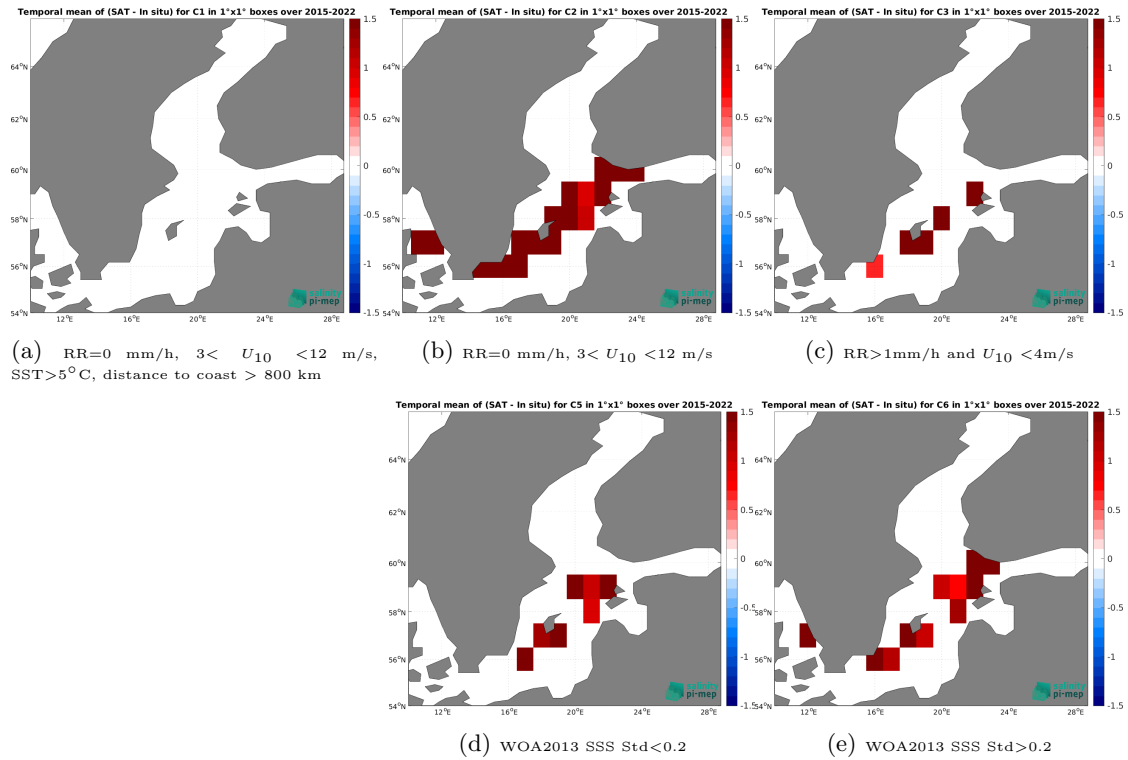
Figure 12: Temporal mean gridded over spatial boxes of size 1^{\circ}\times 1^{\circ} of \Delta\text{SSS} (SMAP SSS L3 v5 - Monthly (RSS) - TSG (LEGOS-DM)) for 5 different subdatasets corresponding to:RR=0 mm/h, 3 < U_{10} < 12 m/s, SST > 5^{\circ}\text{C} , distance to coast > 800 km (a), RR=0 mm/h, 3 < U_{10} < 12 m/s (b), RR > 1 mm/h and U_{10} < 4 m/s (c), WOA2013 SSS Std < 0.2 (d), WOA2013 SSS Std > 0.2 (e).
