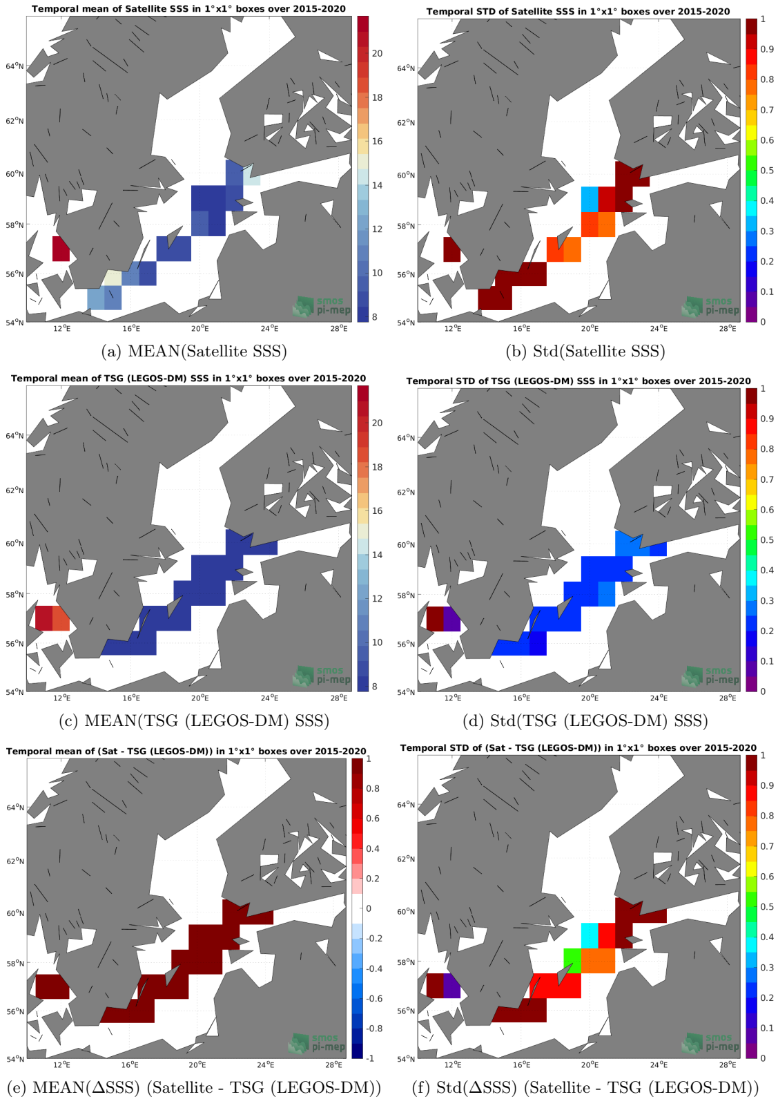
Figure 6: Temporal mean (left) and Std (right) of SSS from SMAP SSS L3 v5 - Monthly (RSS) (top), TSG (LEGOS-DM) (middle), and of \Delta SSS (Satellite - TSG (LEGOS-DM)). Only match-pairs are used to generate these maps.
