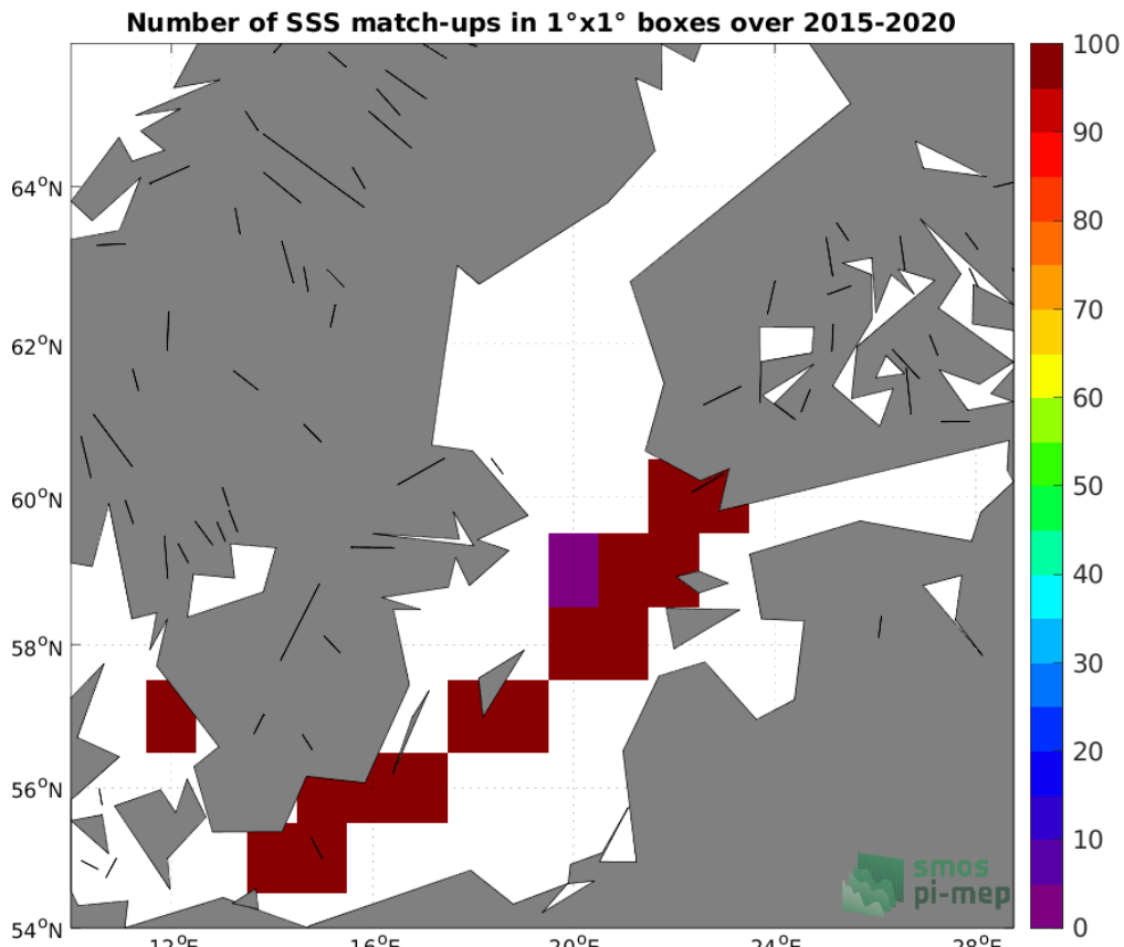
Figure 4: Number of SSS match-ups between TSG (LEGOS-DM) SSS and the SMAP SSS L3 v5 - Monthly (RSS) SSS product for the Baltic Sea Pi-MEP region over 1°×1° boxes and for the full satellite product period.
