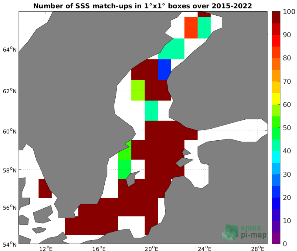
Figure 4: Number of SSS match-ups between ICES SSS and the SMAP SSS L3 v5 - Monthly (RSS) SSS product for the Baltic Sea Pi-MEP region over 1°×1° boxes and for the full satellite product period.
