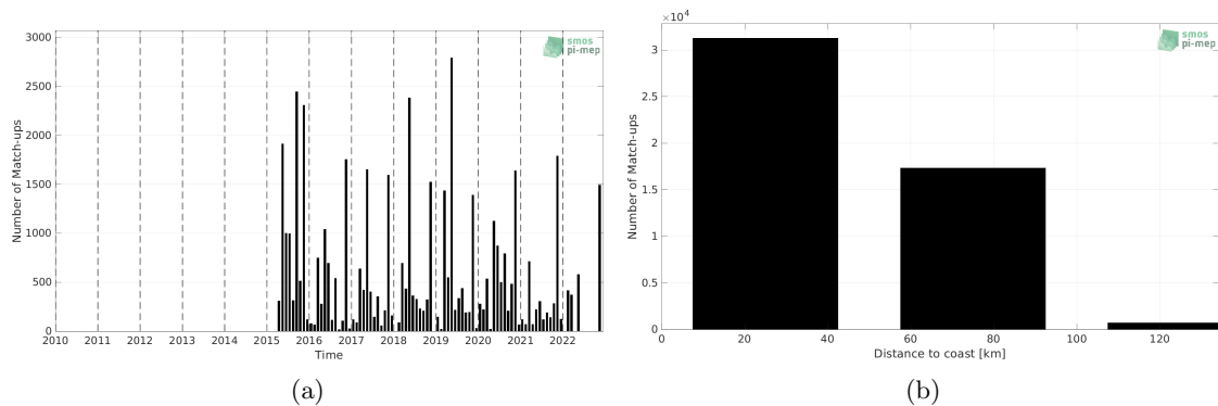
Figure 1: Number of match-ups between ICES and SMAP SSS L3 v5 - Monthly (RSS) SSS as a function of time (a) and as function of the distance to coast (b) over the Baltic Sea Pi-MEP region and for the full satellite product period.
