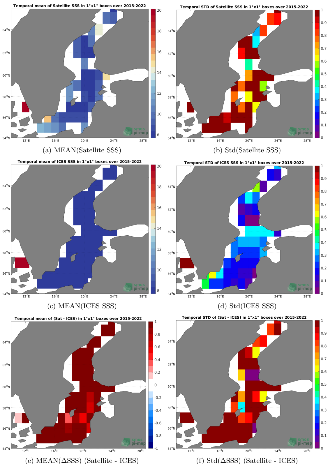
Figure 6: Temporal mean (left) and Std (right) of SSS from SMAP SSS L3 v5 - Monthly (RSS) (top), ICES (middle), and of \Delta SSS (Satellite - ICES). Only match-up pairs are used to generate these maps.
