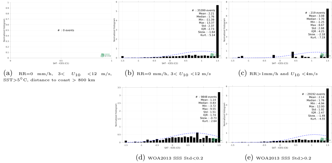
Figure 13: Normalized histogram of \Delta SSS (SMAP SSS L3 v5 - Monthly (RSS) - ICES) for 5 different subdatasets corresponding to: RR=0 mm/h, 3 < U_{10} < 12 m/s, SST>5°C, distance to coast > 800 km (a), RR=0 mm/h, 3 < U_{10} < 12 m/s (b), RR>1mm/h and U_{10} < 4 m/s (c), WOA2013 SSS Std<0.2 (d), WOA2013 SSS Std>0.2 (e).
