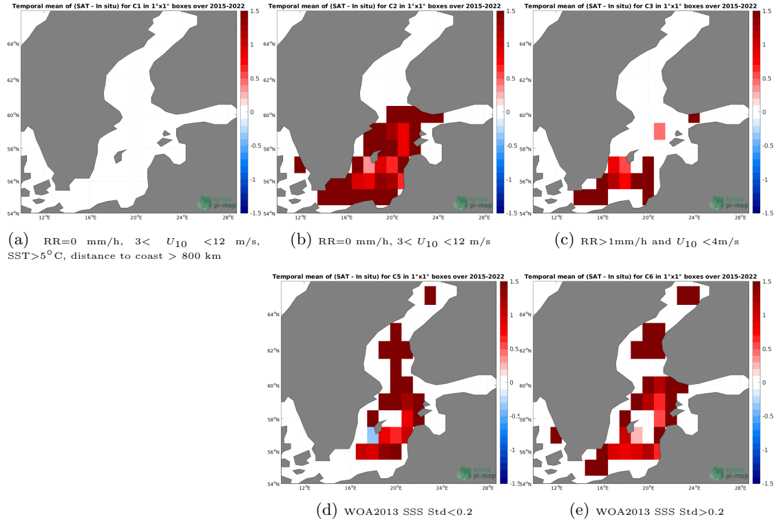
Figure 12: Temporal mean gridded over spatial boxes of size 1^{\circ}\times 1^{\circ} of \Delta\text{SSS} (SMAP SSS L3 v5 - Monthly (RSS) - ICES) for 5 different subdatasets corresponding to: \text{RR}=0 mm/h, 3 < U_{10} < 12 m/s, \text{SST} > 5^{\circ}\text{C} , distance to coast > 800 km (a), \text{RR}=0 mm/h, 3 < U_{10} < 12 m/s (b), \text{RR} > 1\text{mm/h} and U_{10} < 4\text{m/s} (c), WOA2013 SSS Std < 0.2 (d), WOA2013 SSS Std > 0.2 (e).
