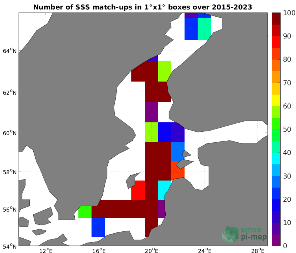
Figure 4: Number of SSS match-ups between Argo SSS and the SMAP SSS L3 v5 - Monthly (RSS) SSS product for the Baltic Sea Pi-MEP region over 1°×1° boxes and for the full satellite product period.
