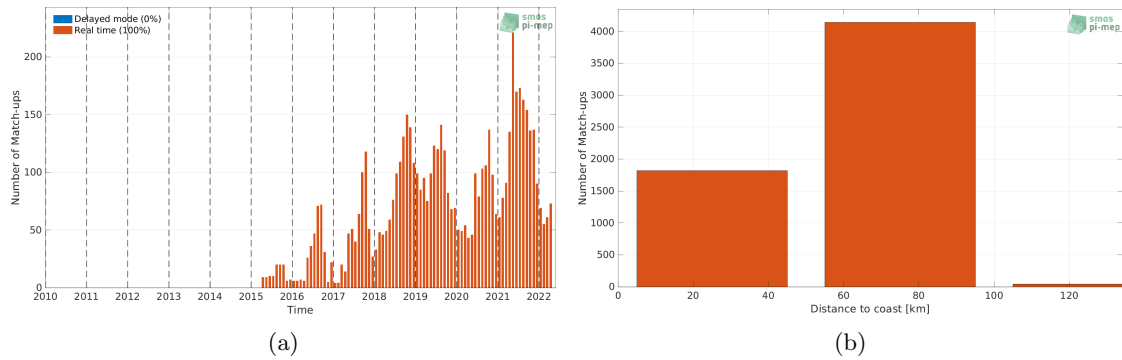
Figure 1: Number of match-ups between Argo and SMAP SSS L3 v5 - Monthly (RSS) SSS as a function of time (a) and as function of the distance to coast (b) over the Baltic Sea Pi-MEP region and for the full satellite product period.
