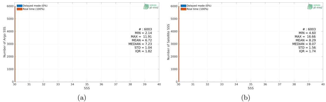
Figure 2: Histograms of SSS from Argo (a) and SMAP SSS L3 v5 - Monthly (RSS) (b) considering all match-up pairs per bins of 0.1 over the Baltic Sea Pi-MEP region and for the full satellite product period.
