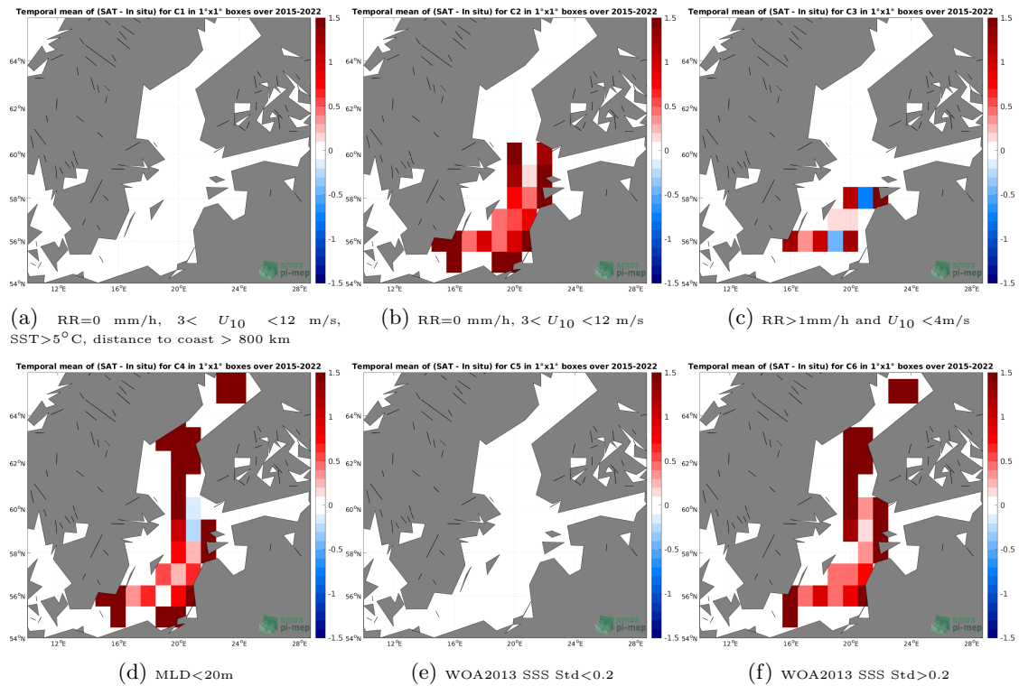
Figure 12: Temporal mean gridded over spatial boxes of size 1^{\circ}\times 1^{\circ} of \Delta\text{SSS} (SMAP SSS L3 v5 - Monthly (RSS) - Argo) for 6 different subdatasets corresponding to:RR=0 mm/h, 3 < U_{10} < 12 m/s, SST >5^{\circ}\text{C} , distance to coast > 800 km (a), RR=0 mm/h, 3 < U_{10} < 12 m/s (b), RR >1 mm/h and U_{10} < 4 m/s (c),MLD <20 m (d),WOA2013 SSS Std <0.2 (e),WOA2013 SSS Std >0.2 (f).
