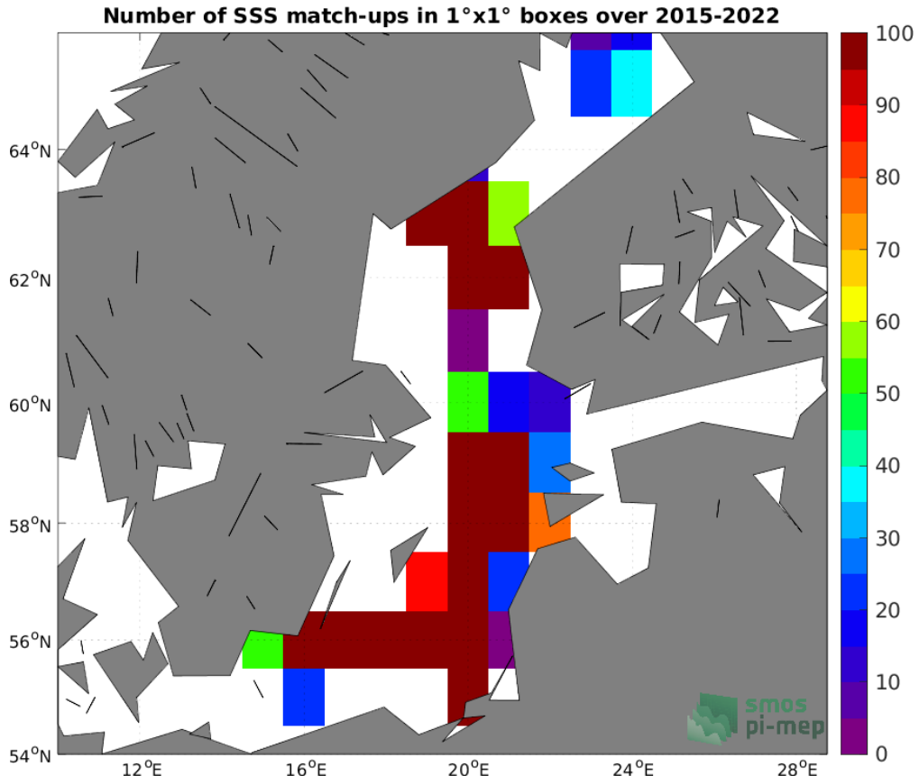
Figure 4: Number of SSS match-ups between Argo SSS and the SMAP SSS L3 v5 - Monthly (RSS) SSS product for the Baltic Sea Pi-MEP region over 1^{\circ} \times 1^{\circ} boxes and for the full satellite product period.
