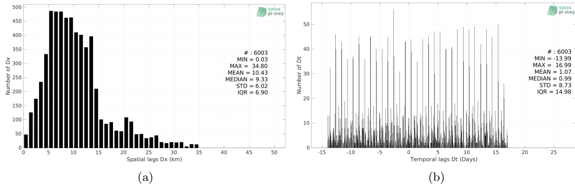
Figure 5: Histograms of the spatial (a) and temporal (b) lags between the location/time of the Argo measurement and the date of the corresponding SMAP SSS L3 v5 - Monthly (RSS) SSS pixel.
