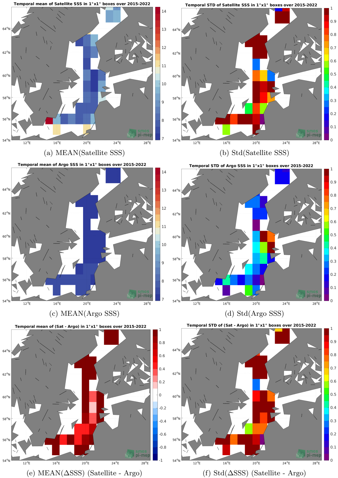
Figure 6: Temporal mean (left) and Std (right) of SSS from SMAP SSS L3 v5 - Monthly (RSS) (top), Argo (middle), and of \Delta SSS (Satellite - Argo). Only match-up pairs are used to generate these maps.
