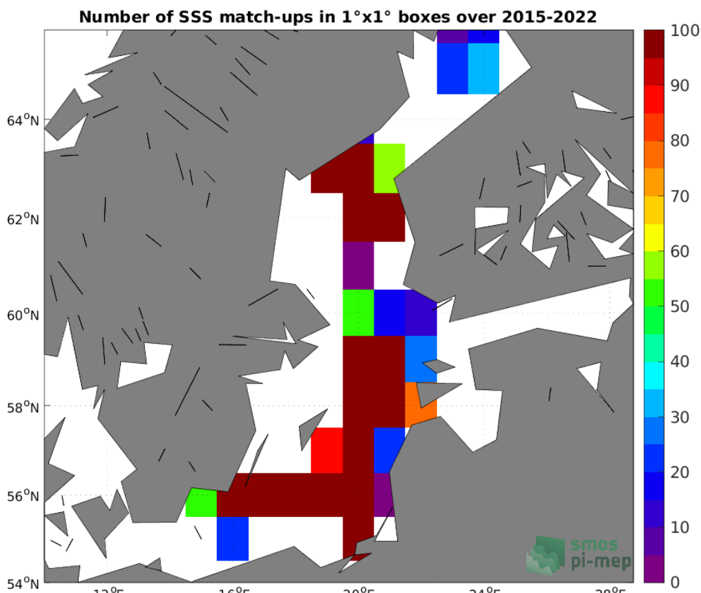
Figure 4: Number of SSS match-ups between Argo SSS and the SMAP SSS L3 v5 - Monthly (RSS) SSS product for the Baltic Sea Pi-MEP region over 1^\circ \times 1^\circ boxes and for the full satellite product period.
