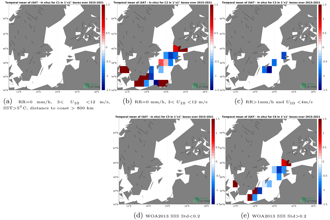
Figure 12: Temporal mean gridded over spatial boxes of size 1^{\circ}\times 1^{\circ} of \Delta\text{SSS} (SMAP SSS L3 v4 - 8-Day running (RSS) - TSG (LEGOS-DM)) for 5 different subdatasets corresponding to:RR=0 mm/h, 3 < U_{10} < 12 m/s, SST >5^{\circ}\text{C} , distance to coast > 800 km (a), RR=0 mm/h, 3 < U_{10} < 12 m/s (b), RR >1 mm/h and U_{10} < 4 m/s (c), WOA2013 SSS Std <0.2 (d), WOA2013 SSS Std >0.2 (e).
