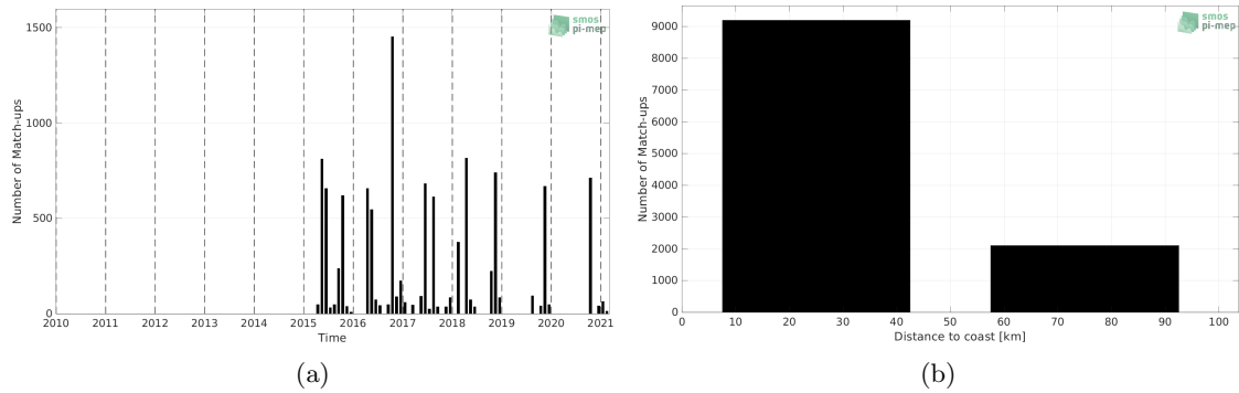
Figure 1: Number of match-ups between TSG (LEGOS-DM) and SMAP SSS L3 v4 - 8-Day running (RSS) SSS as a function of time (a) and as function of the distance to coast (b) over the Baltic Sea Pi-MEP region and for the full satellite product period.
