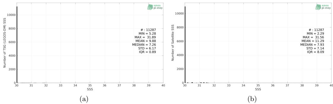
Figure 2: Histograms of SSS from TSG (LEGOS-DM) (a) and SMAP SSS L3 v4 - 8-Day running (RSS) (b) considering all match-up pairs per bins of 0.1 over the Baltic Sea Pi-MEP region and for the full satellite product period.
