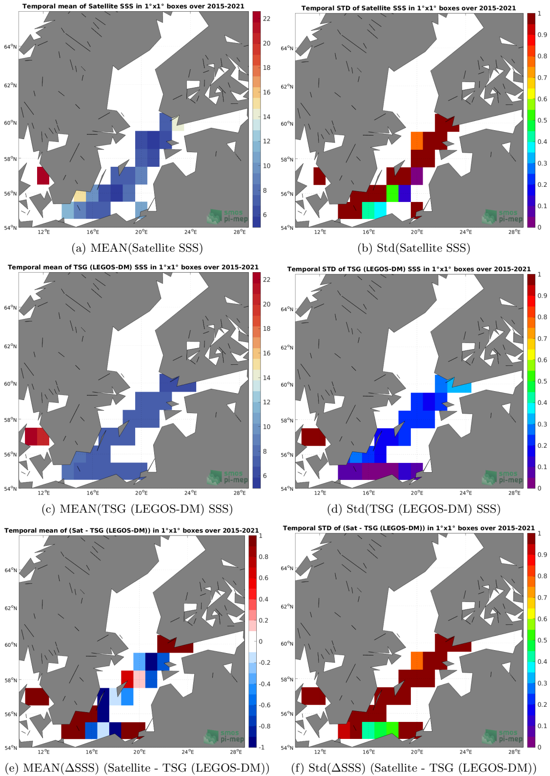
Figure 6: Temporal mean (left) and Std (right) of SSS from SMAP SSS L3 v4 - 8-Day running (RSS) (top), TSG (LEGOS-DM) (middle), and of \Delta SSS (Satellite - TSG (LEGOS-DM)). Only match-up pairs are used to generate these maps.
