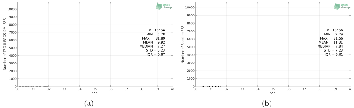
Figure 2: Histograms of SSS from TSG (LEGOS-DM) (a) and SMAP SSS L3 v4 - 8-Day running (RSS) (b) considering all match-up pairs per bins of 0.1 over the Baltic Sea Pi-MEP region and for the full satellite product period.
