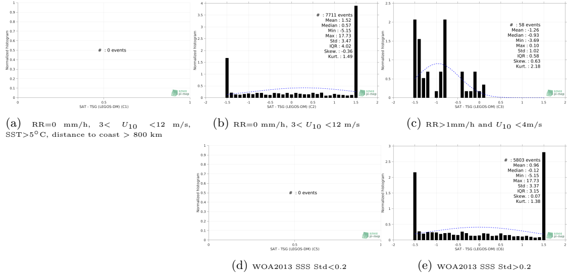
Figure 13: Normalized histogram of \Delta\text{SSS} (SMAP SSS L3 v4 - 8-Day running (RSS) - TSG (LEGOS-DM)) for 5 different subdatasets corresponding to: RR=0 mm/h, 3 < U_{10} < 12 m/s, SST > 5^\circ\text{C} , distance to coast > 800 km (a), RR=0 mm/h, 3 < U_{10} < 12 m/s (b), RR > 1 mm/h and U_{10} < 4 m/s (c), WOA2013 SSS Std < 0.2 (d), WOA2013 SSS Std > 0.2 (e).
