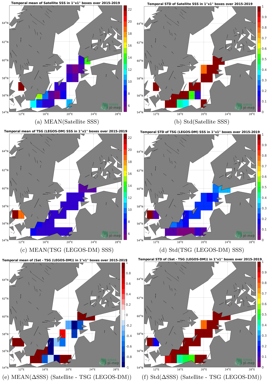
Figure 6: Temporal mean (left) and Std (right) of SSS from SMAP SSS L3 v4 - 8-Day running (RSS) (top), TSG (LEGOS-DM) (middle), and \Delta SSS (Satellite - TSG (LEGOS-DM)). Only match-up pairs are used to generate these maps.
