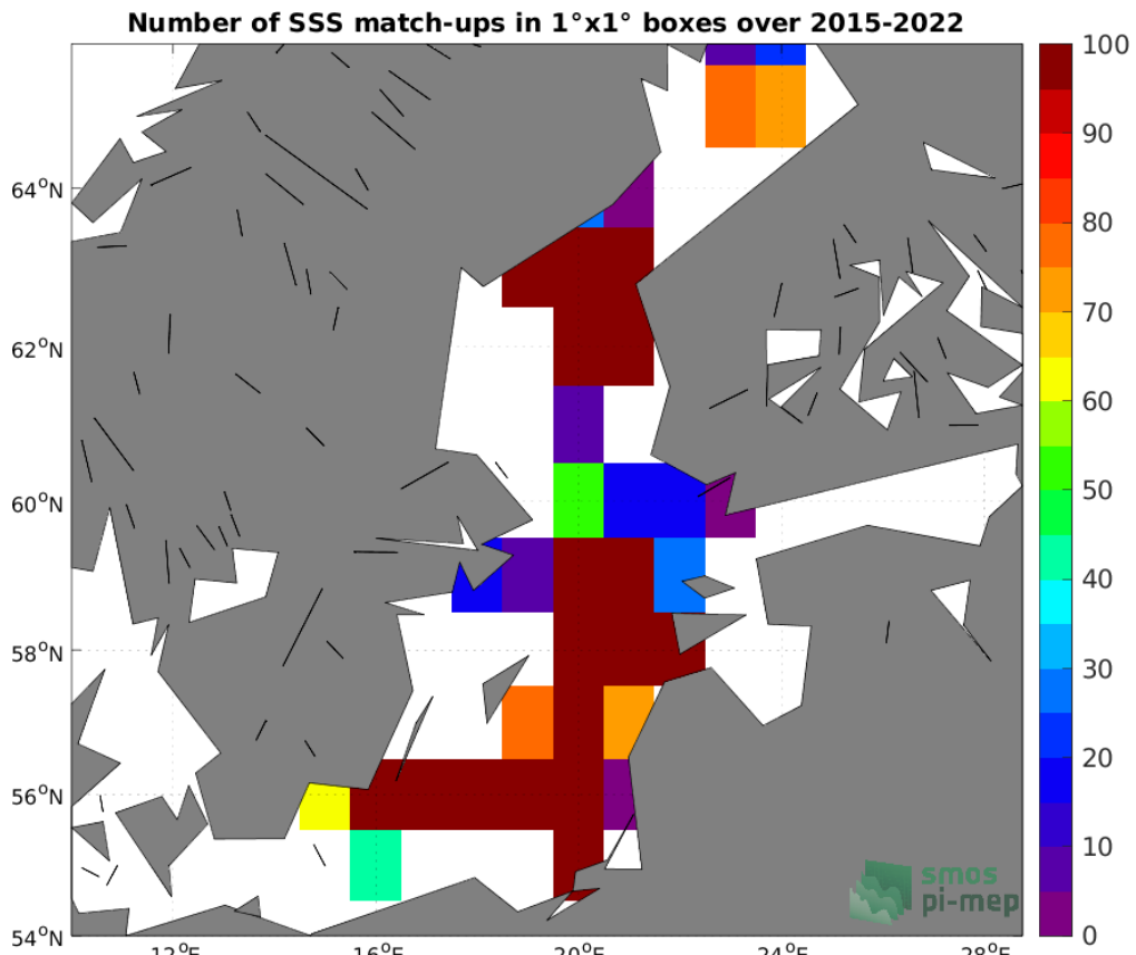
Figure 4: Number of SSS match-ups between Argo SSS and the SMAP SSS L3 v4 - 8-Day running (RSS) SSS product for the Baltic Sea Pi-MEP region over 1°×1° boxes and for the full satellite product period.
