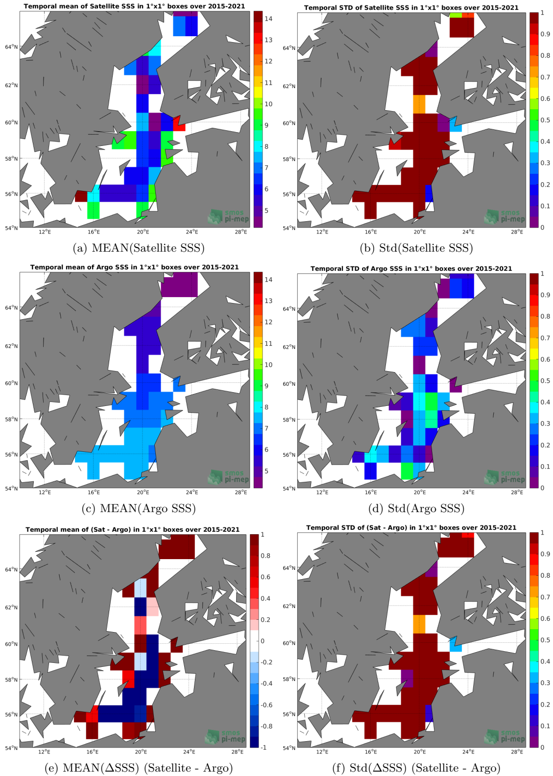
Figure 6: Temporal mean (left) and Std (right) of SSS from SMAP SSS L3 v4 - 8-Day running (RSS) (top), Argo (middle), and of \Delta SSS (Satellite - Argo). Only match-up pairs are used to generate these maps.
