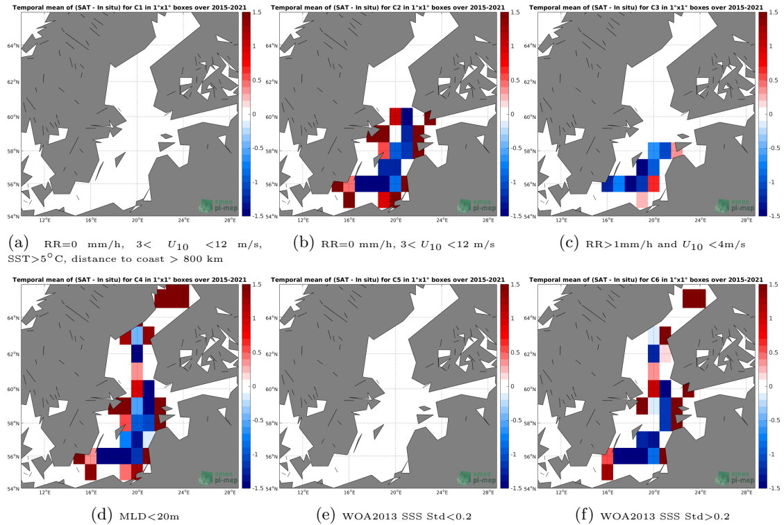
Figure 12: Temporal mean gridded over spatial boxes of size 1^{\circ}\times 1^{\circ} of \Delta\text{SSS} (SMAP SSS L3 v4 - 8-Day running (RSS) - Argo) for 6 different subdatasets corresponding to:RR=0 mm/h, 3 < U_{10} < 12 m/s, SST > 5^{\circ}\text{C} , distance to coast > 800 km (a), RR=0 mm/h, 3 < U_{10} < 12 m/s (b), RR > 1\text{mm/h} and U_{10} < 4\text{m/s} (c),MLD < 20\text{m} (d),WOA2013 SSS Std < 0.2 (e),WOA2013 SSS Std > 0.2 (f).
