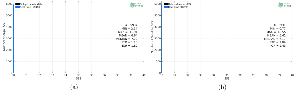
Figure 2: Histograms of SSS from Argo (a) and SMAP SSS L3 v4 - 8-Day running (RSS) (b) considering all match-up pairs per bins of 0.1 over the Baltic Sea Pi-MEP region and for the full satellite product period.
