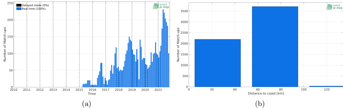
Figure 1: Number of match-ups between Argo and SMAP SSS L3 v4 - 8-Day running (RSS) SSS as a function of time (a) and as function of the distance to coast (b) over the Baltic Sea Pi-MEP region and for the full satellite product period.
