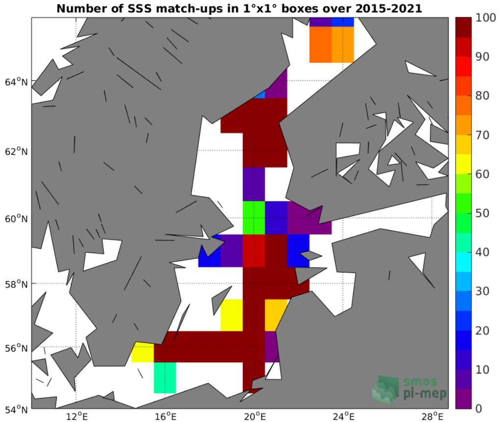
Figure 4: Number of SSS match-ups between Argo SSS and the SMAP SSS L3 v4 - 8-Day running (RSS) SSS product for the Baltic Sea Pi-MEP region over 1^\circ \times 1^\circ boxes and for the full satellite product period.
