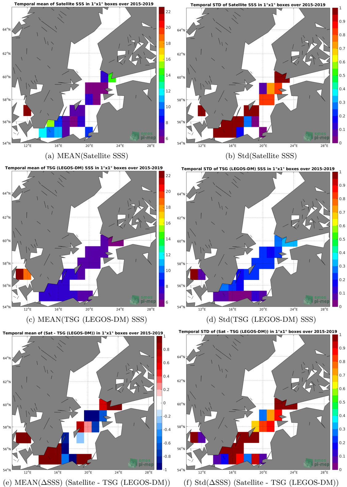
Figure 6: Temporal mean (left) and Std (right) of SSS from SMAP SSS L3 v4 - Monthly (RSS) (top), TSG (LEGOS-DM) (middle), and of \Delta SSS (Satellite - TSG (LEGOS-DM)). Only match-pairs are used to generate these maps.
