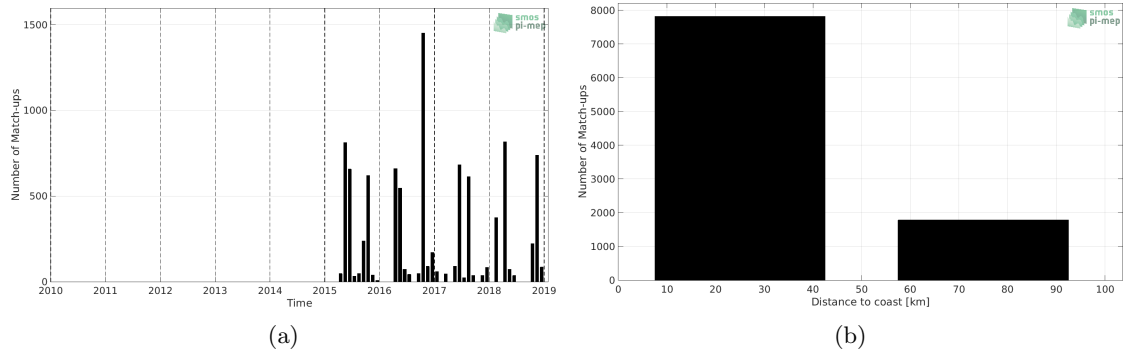
Figure 1: Number of match-ups between TSG (LEGOS-DM) and SMAP SSS L3 v4 - Monthly (RSS) SSS as a function of time (a) and as function of the distance to coast (b) over the Baltic Sea Pi-MEP region and for the full satellite product period.
