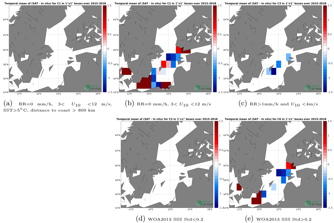
Figure 12: Temporal mean gridded over spatial boxes of size 1^{\circ}\times 1^{\circ} of \Delta\text{SSS} (SMAP SSS L3 v4 - Monthly (RSS) - TSG (LEGOS-DM)) for 5 different subdatasets corresponding to:RR=0 mm/h, 3 < U_{10} < 12 m/s, SST >5^{\circ}\text{C} , distance to coast > 800 km (a), RR=0 mm/h, 3 < U_{10} < 12 m/s (b), RR >1 mm/h and U_{10} < 4 m/s (c), WOA2013 SSS Std <0.2 (d), WOA2013 SSS Std >0.2 (e).
