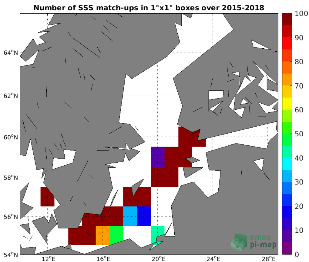
Figure 4: Number of SSS match-ups between TSG (LEGOS-DM) SSS and the SMAP SSS L3 v4 - Monthly (RSS) SSS product for the Baltic Sea Pi-MEP region over 1°x1° boxes and for the full satellite product period.
