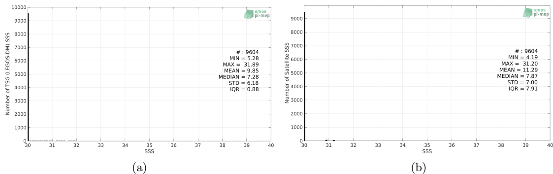
Figure 2: Histograms of SSS from TSG (LEGOS-DM) (a) and SMAP SSS L3 v4 - Monthly (RSS) (b) considering all match-up pairs per bins of 0.1 over the Baltic Sea Pi-MEP region and for the full satellite product period.
