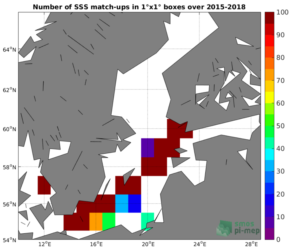
Figure 4: Number of SSS match-ups between TSG-LEGOS-DM SSS and the SMAP-L3-RSS-V4-MONTHLY SSS product for the Baltic Sea Pi-MEP region over 1°x1° boxes and for the full satellite product period.
