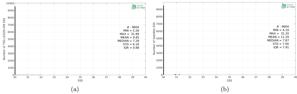
Figure 2: Histograms of SSS from TSG-LEGOS-DM (a) and SMAP-L3-RSS-V4-MONTHLY (b) considering all match-up pairs per bins of 0.1 over the Baltic Sea Pi-MEP region and for the full satellite product period.
