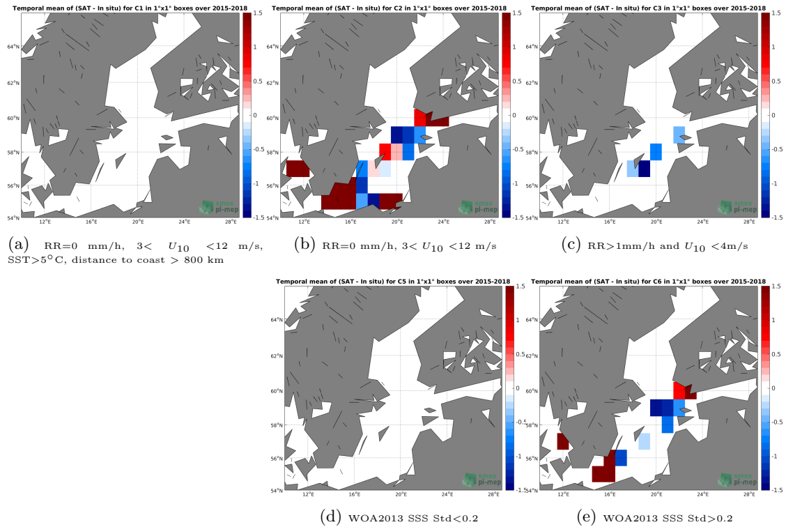
Figure 12: Temporal mean gridded over spatial boxes of size 1^{\circ}\times 1^{\circ} of \Delta\text{SSS} (SMAP-L3-RSS-V4-MONTHLY - TSG-LEGOS-DM) for 5 different subdatasets corresponding to:RR=0 mm/h, 3 < U_{10} < 12 m/s, SST >5^{\circ}\text{C} , distance to coast > 800 km (a), RR=0 mm/h, 3 < U_{10} < 12 m/s (b), RR >1 mm/h and U_{10} < 4 m/s (c), WOA2013 SSS Std <0.2 (d), WOA2013 SSS Std >0.2 (e).
