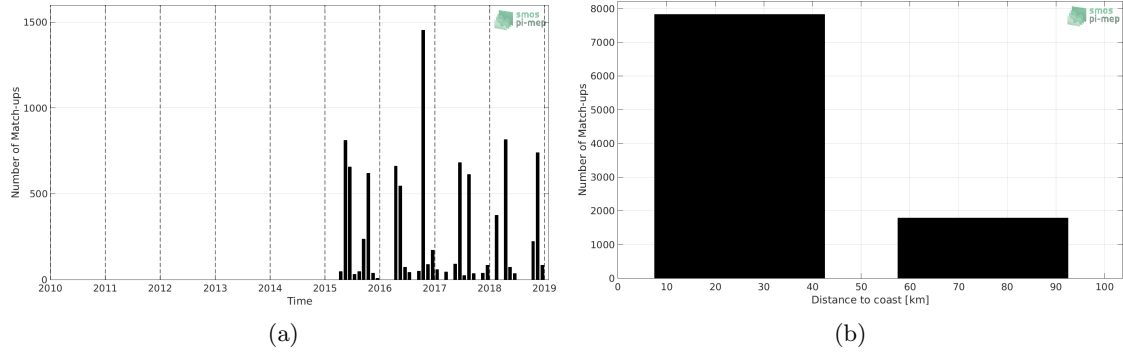
Figure 1: Number of match-ups between TSG-LEGOS-DM and SMAP-L3-RSS-V4-MONTHLY SSS as a function of time (a) and as function of the distance to coast (b) over the Baltic Sea Pi-MEP region and for the full satellite product period.
