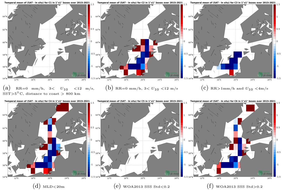
Figure 12: Temporal mean gridded over spatial boxes of size 1^{\circ}\times 1^{\circ} of \Delta\text{SSS} (SMAP SSS L3 v4 - Monthly (RSS) - Argo) for 6 different subdatasets corresponding to:RR=0 mm/h, 3 < U_{10} < 12 m/s, SST >5^{\circ}\text{C} , distance to coast > 800 km (a), RR=0 mm/h, 3 < U_{10} < 12 m/s (b), RR >1\text{mm/h} and U_{10} < 4\text{m/s} (c),MLD <20\text{m} (d),WOA2013 SSS Std <0.2 (e),WOA2013 SSS Std >0.2 (f).
