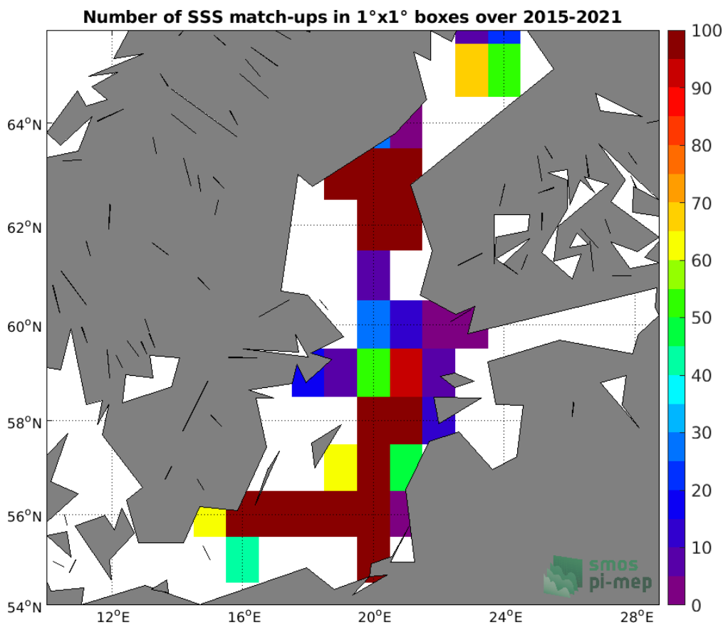
Figure 4: Number of SSS match-ups between Argo SSS and the SMAP SSS L3 v4 - Monthly (RSS) SSS product for the Baltic Sea Pi-MEP region over 1°x1° boxes and for the full satellite product period.
