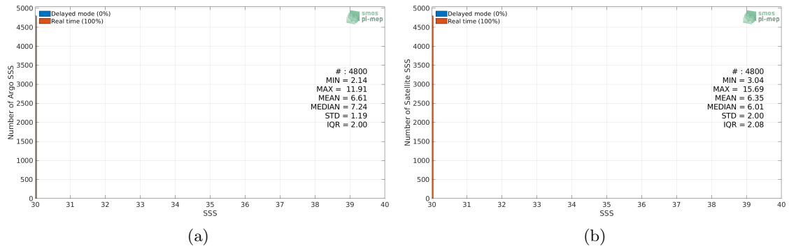
Figure 2: Histograms of SSS from Argo (a) and SMAP SSS L3 v4 - Monthly (RSS) (b) considering all match-up pairs per bins of 0.1 over the Baltic Sea Pi-MEP region and for the full satellite product period.
