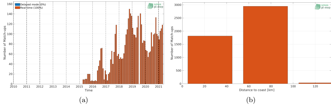
Figure 1: Number of match-ups between Argo and SMAP SSS L3 v4 - Monthly (RSS) SSS as a function of time (a) and as function of the distance to coast (b) over the Baltic Sea Pi-MEP region and for the full satellite product period.
