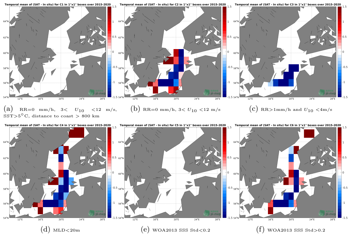
Figure 12: Temporal mean gridded over spatial boxes of size 1^{\circ}\times 1^{\circ} of \Delta\text{SSS} (SMAP SSS L3 v4 - Monthly (RSS) - Argo) for 6 different subdatasets corresponding to: \text{RR}=0 mm/h, 3 < U_{10} < 12 m/s, \text{SST} > 5^{\circ}\text{C} , distance to coast > 800 km (a), \text{RR}=0 mm/h, 3 < U_{10} < 12 m/s (b), \text{RR} > 1\text{mm/h} and U_{10} < 4\text{m/s} (c), \text{MLD} < 20\text{m} (d), \text{WOA2013 SSS Std} < 0.2 (e), \text{WOA2013 SSS Std} > 0.2 (f).
