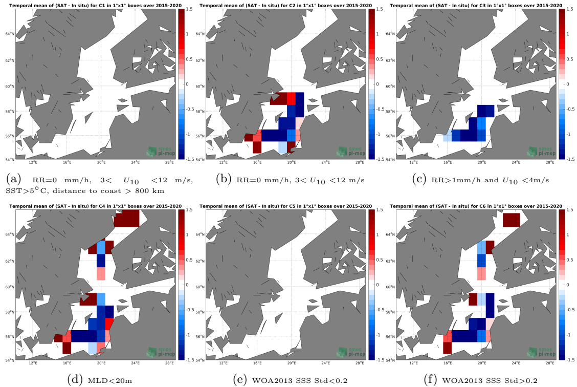
Figure 12: Temporal mean gridded over spatial boxes of size 1^{\circ}\times 1^{\circ} of \Delta\text{SSS} (SMAP-L3-RSS-V4-MONTHLY - Argo) for 6 different subdatasets corresponding to:RR=0 mm/h, 3 < U_{10} < 12 m/s, SST >5^{\circ}\text{C} , distance to coast > 800 km (a), RR=0 mm/h, 3 < U_{10} < 12 m/s (b), RR >1 mm/h and U_{10} < 4 m/s (c),MLD <20 m (d),WOA2013 SSS Std <0.2 (e),WOA2013 SSS Std >0.2 (f).
