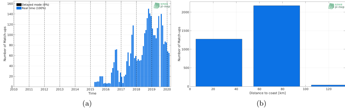
Figure 1: Number of match-ups between Argo and SMAP-L3-RSS-V4-MONTHLY SSS as a function of time (a) and as function of the distance to coast (b) over the Baltic Sea Pi-MEP region and for the full satellite product period.
