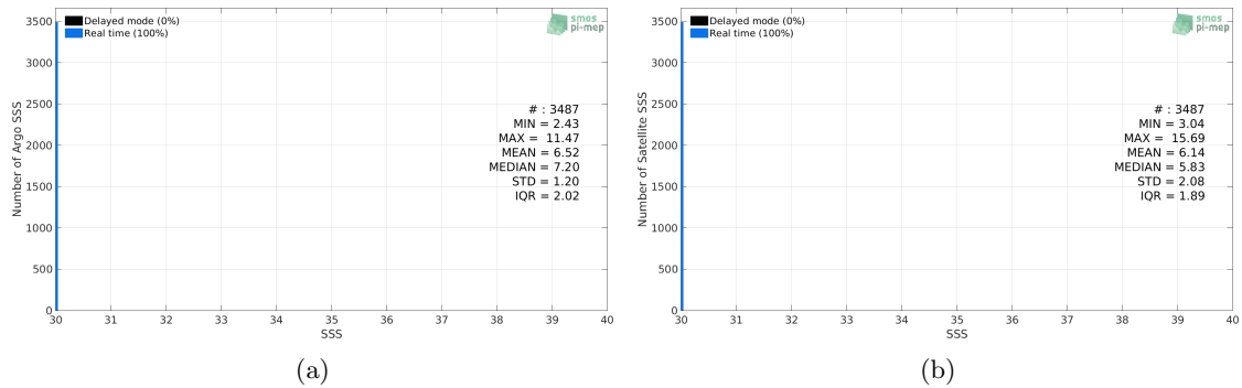
Figure 2: Histograms of SSS from Argo (a) and SMAP-L3-RSS-V4-MONTHLY (b) considering all match-up pairs per bins of 0.1 over the Baltic Sea Pi-MEP region and for the full satellite product period.
