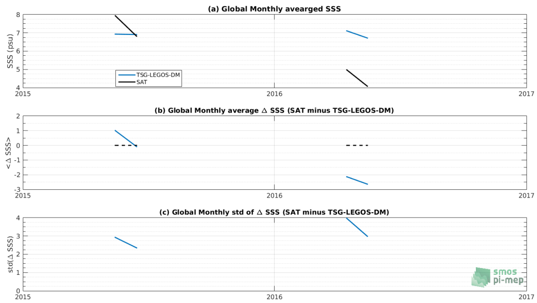
Figure 7: Time series of the monthly averaged mean SSS (top), mean \Delta SSS (Satellite - TSG-LEGOS-DM) and Std of \Delta SSS (Satellite - TSG-LEGOS-DM) over the Baltic Sea Pi-MEP region considering all match-ups collected by the Pi-MEP platform.
