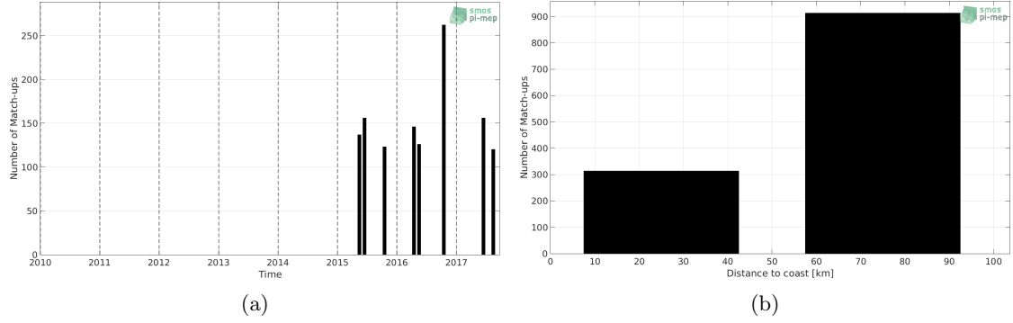
Figure 1: Number of match-ups between TSG-LEGOS-DM and SMAP-L3-RSS-V3-8DAY-RUNNING-40KM SSS as a function of time (a) and as function of the distance to coast (b) over the Baltic Sea Pi-MEP region and for the full satellite product period.
