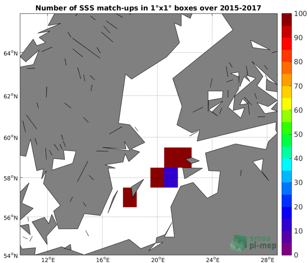
Figure 4: Number of SSS match-ups between TSG-LEGOS-DM SSS and the SMAP-L3-RSS-V3-8DAY-RUNNING-40KM SSS product for the Baltic Sea Pi-MEP region over 1°x1° boxes and for the full satellite product period.
