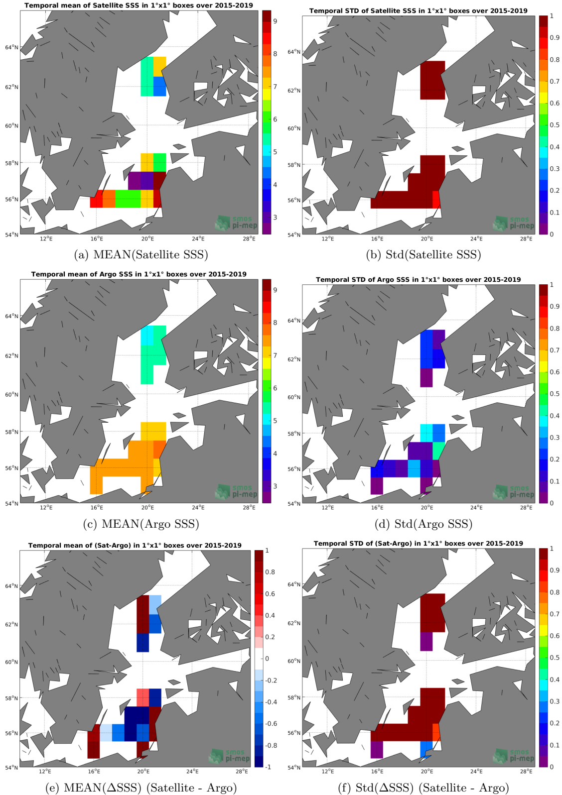
Figure 6: Temporal mean (left) and Std (right) of SSS from SMAP-L3-RSS-V3-8DAY-RUNNING-40KM (top), Argo (middle), and \Delta SSS (Satellite - Argo). Only match-up pairs are used to generate these maps.
