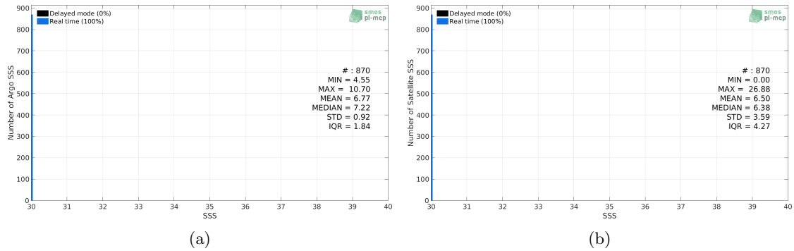
Figure 2: Histograms of SSS from Argo (a) and SMAP-L3-RSS-V3-8DAY-RUNNING-40KM (b) considering all match-up pairs per bins of 0.1 over the Baltic Sea Pi-MEP region and for the full satellite product period.
