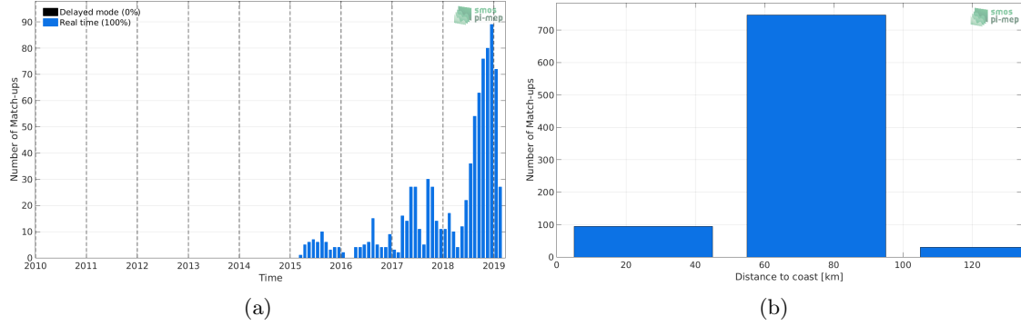
Figure 1: Number of match-ups between Argo and SMAP-L3-RSS-V3-8DAY-RUNNING-40KM SSS as a function of time (a) and as function of the distance to coast (b) over the Baltic Sea Pi-MEP region and for the full satellite product period.
