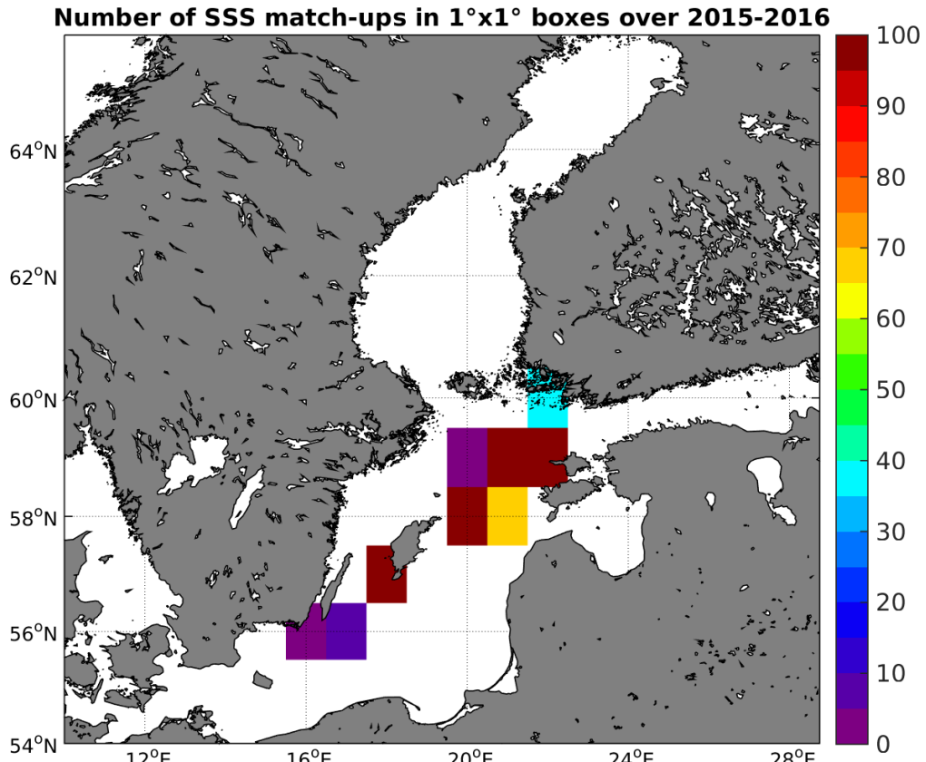
Figure 4: Number of SSS match-ups between TSG-LEGOS-DM SSS and the SMAP-L3-RSS-V2-8DAY-RUNNING-40KM SSS product for the Baltic Sea Pi-MEP region over 1°x1° boxes and for the full satellite product period.
