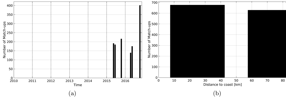
Figure 1: Number of match-ups between TSG-LEGOS-DM and SMAP-L3-RSS-V2-8DAY-RUNNING-40KM SSS as a function of time (a) and as function of the distance to coast (b) over the Baltic Sea Pi-MEP region and for the full satellite product period.
