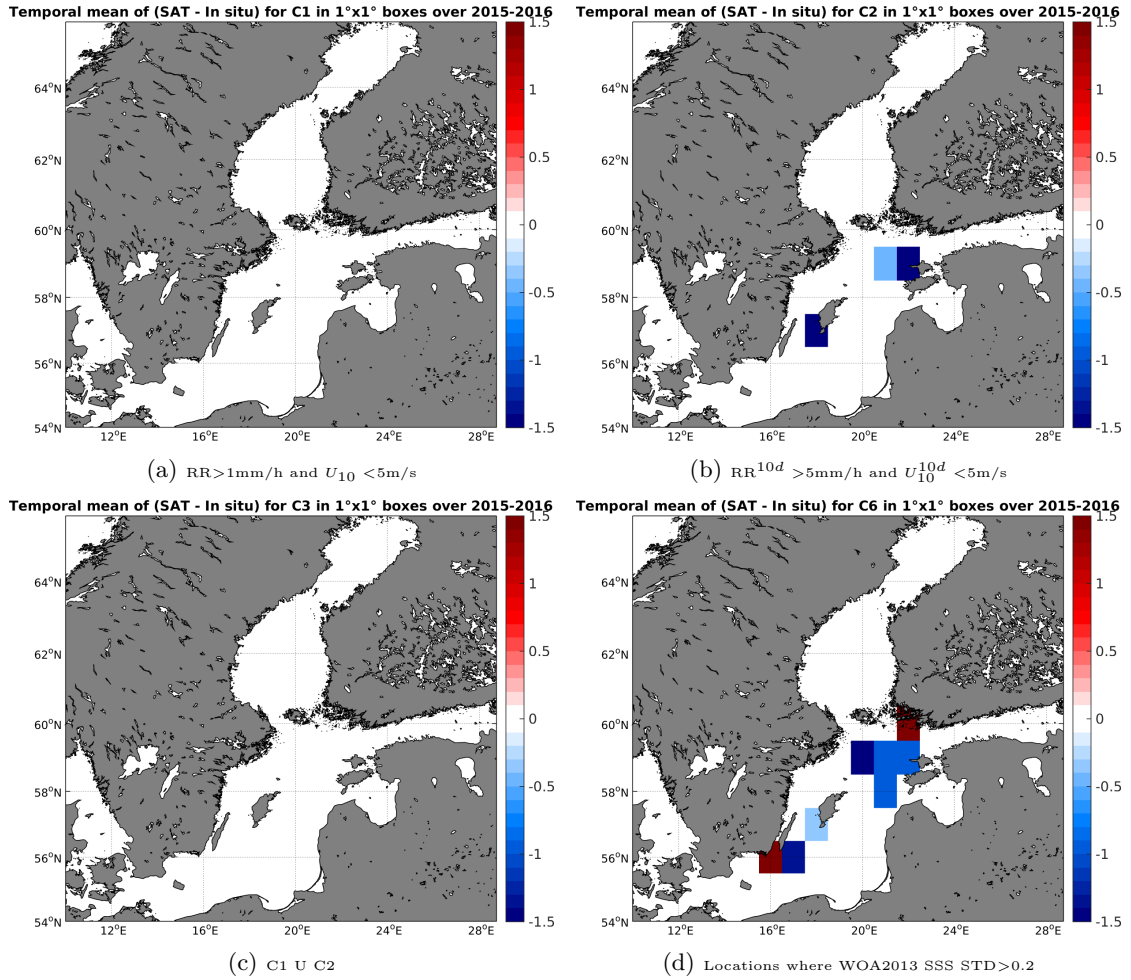
Figure 12: Temporal mean gridded over spatial boxes of size 1°x1° of \Delta SSS (SMAP-L3-RSS-V2-8DAY-RUNNING-40KM - TSG-LEGOS-DM) for 4 different subdatasets corresponding to: RR > 1\text{mm/h} and U_{10} < 5\text{m/s} (a), RR^{10d} > 5\text{mm/h} and U_{10}^{10d} < 5\text{m/s} (b), C1 U C2 (c), Locations where WOA2013 SSS STD > 0.2 (d).
