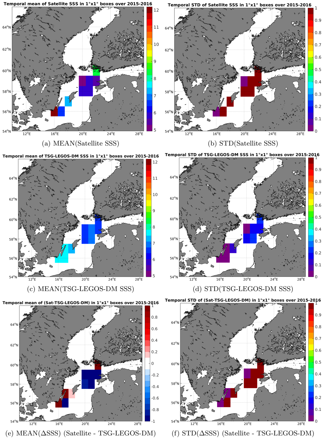
Figure 6: Temporal mean (left) and STD (right) of SSS from SMAP-L3-RSS-V2-8DAY-RUNNING-40KM (top), TSG-LEGOS-DM (middle), and of \Delta SSS (Satellite - TSG-LEGOS-DM). Only match-up pairs are used to generate these maps.
