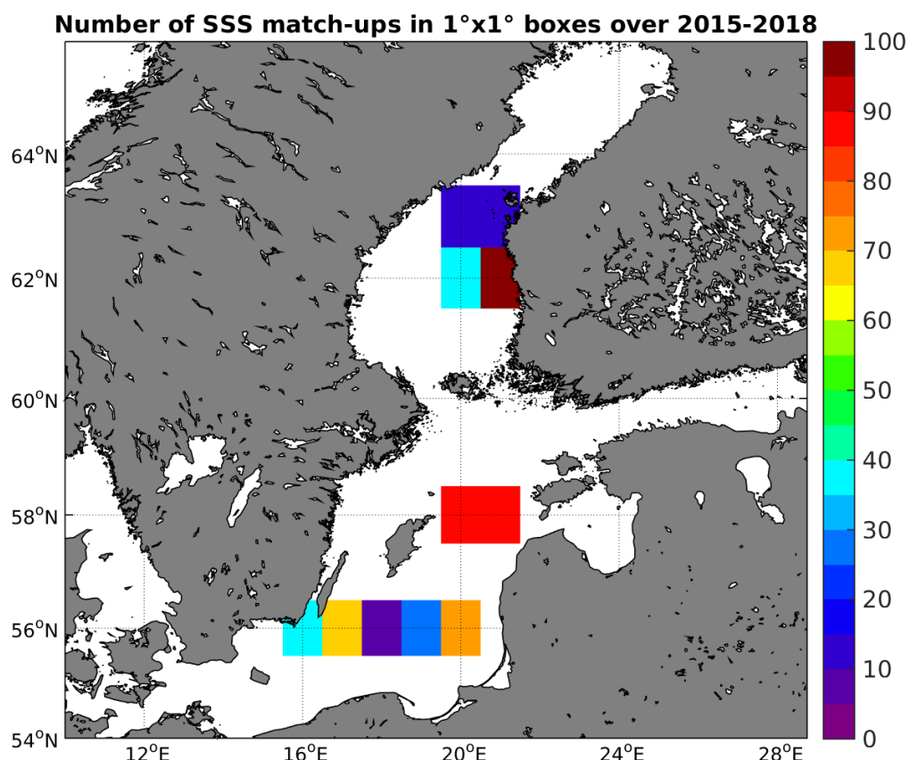
Figure 4: Number of SSS match-ups between Argo SSS and the SMAP-L3-RSS-V2-8DAY-RUNNING-40KM SSS product for the Baltic Sea Pi-MEP region over 1°x1° boxes and for the full satellite product period.
