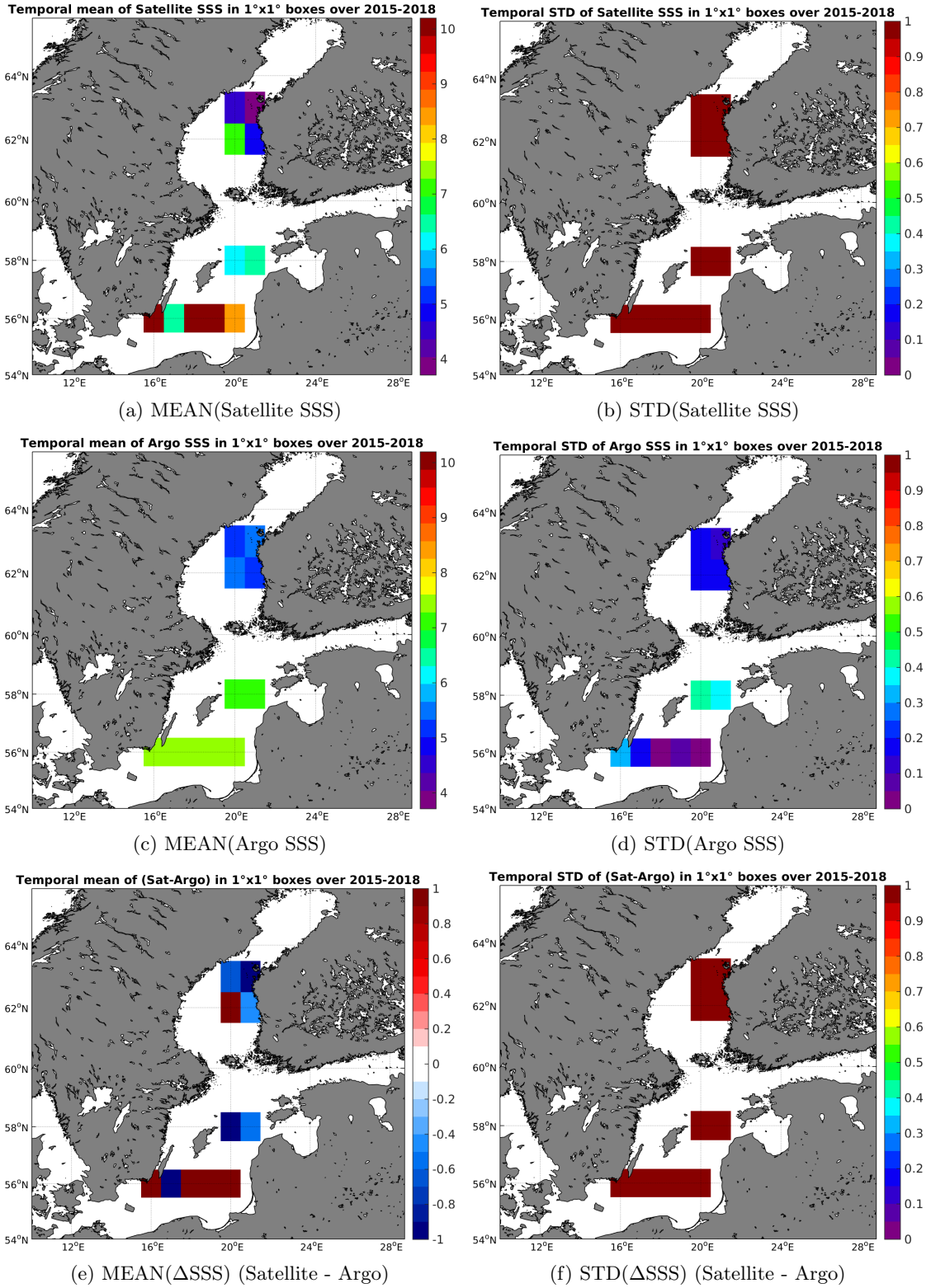
Figure 6: Temporal mean (left) and STD (right) of SSS from SMAP-L3-RSS-V2-8DAY-RUNNING-40KM (top), Argo (middle), and of \Delta SSS (Satellite - Argo). Only match-up pairs are used to generate these maps.
