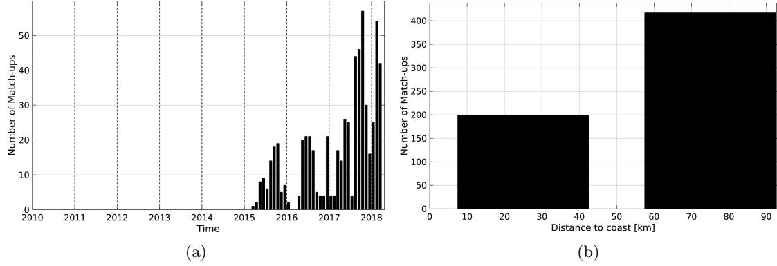
Figure 1: Number of match-ups between Argo and SMAP-L3-RSS-V2-8DAY-RUNNING-40KM SSS as a function of time (a) and as function of the distance to coast (b) over the Baltic Sea Pi-MEP region and for the full satellite product period.
