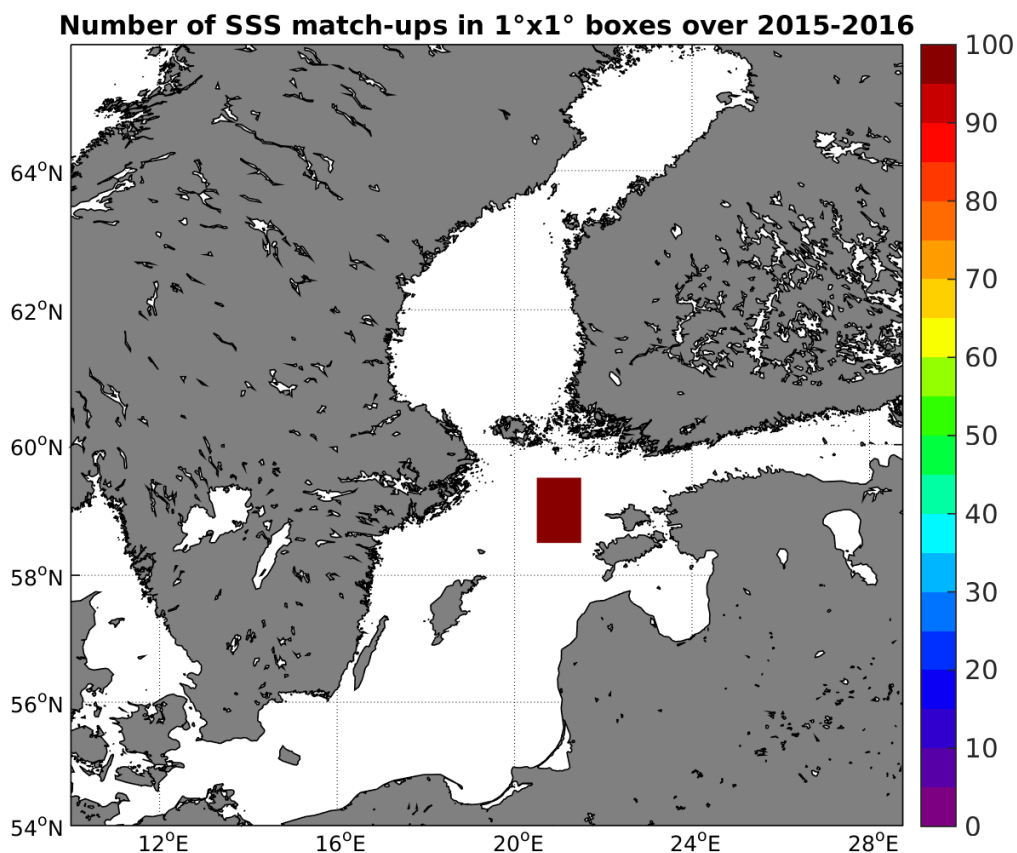
Figure 4: Number of SSS match-ups between TSG-LEGOS-DM SSS and the SMAP-L3-RSS-V2-8DAY-RUNNING-70KM SSS product for the Baltic Sea Pi-MEP region over 1°x1° boxes and for the full satellite product period.
