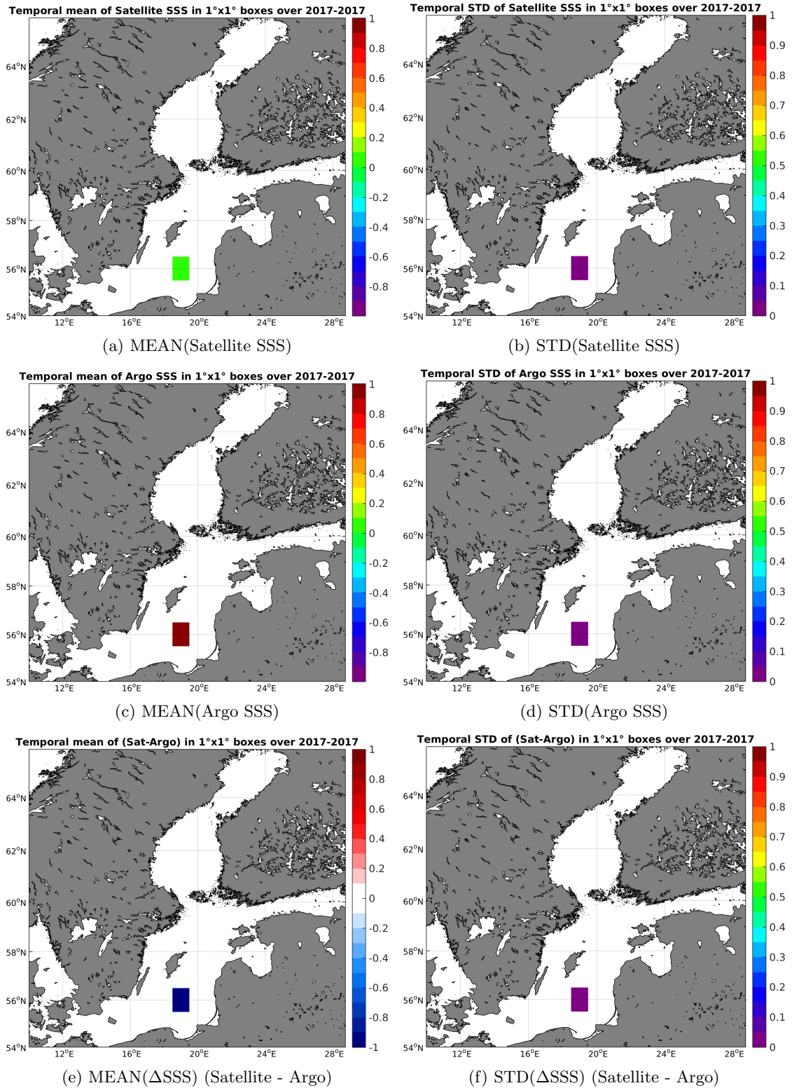
Figure 6: Temporal mean (left) and STD (right) of SSS from SMAP-L3-RSS-V2-8DAY-RUNNING-70KM (top), Argo (middle), and of \Delta SSS (Satellite - Argo). Only match-up pairs are used to generate these maps.
