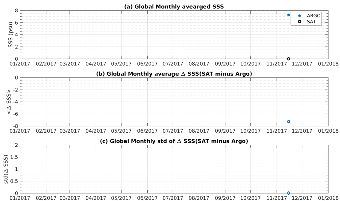
Figure 7: Time series of the monthly averaged mean SSS (top), mean \Delta SSS (Satellite - Argo) and STD of \Delta SSS (Satellite - Argo) over the Baltic Sea Pi-MEP region considering all match-ups collected by the Pi-MEP platform.
