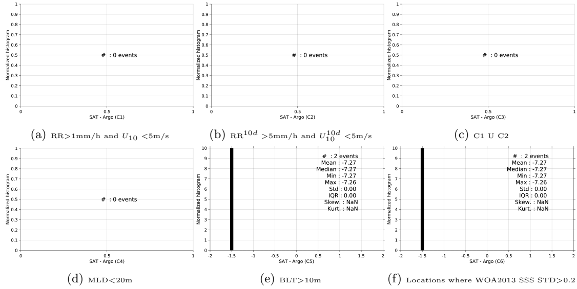
Figure 13: Normalized histogram of \Delta\text{SSS} (SMAP-L3-RSS-V2-8DAY-RUNNING-70KM - Argo) for 6 different subdatasets corresponding to: RR > 1\text{mm/h} and U_{10} < 5\text{m/s} (a), RR^{10d} > 5\text{mm/h} and U_{10}^{10d} < 5\text{m/s} (b), C1 U C2 (c), MLD < 20\text{m} (d), BLT > 10\text{m} (e), Locations where WOA2013 SSS STD > 0.2 (f).
