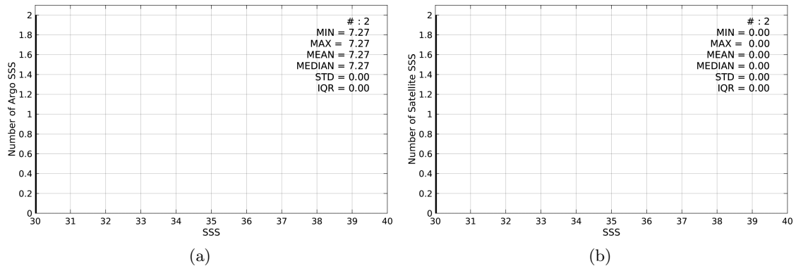
Figure 2: Histograms of SSS from Argo (a) and SMAP-L3-RSS-V2-8DAY-RUNNING-70KM (b) considering all match-up pairs per bins of 0.1 over the Baltic Sea Pi-MEP region and for the full satellite product period.
