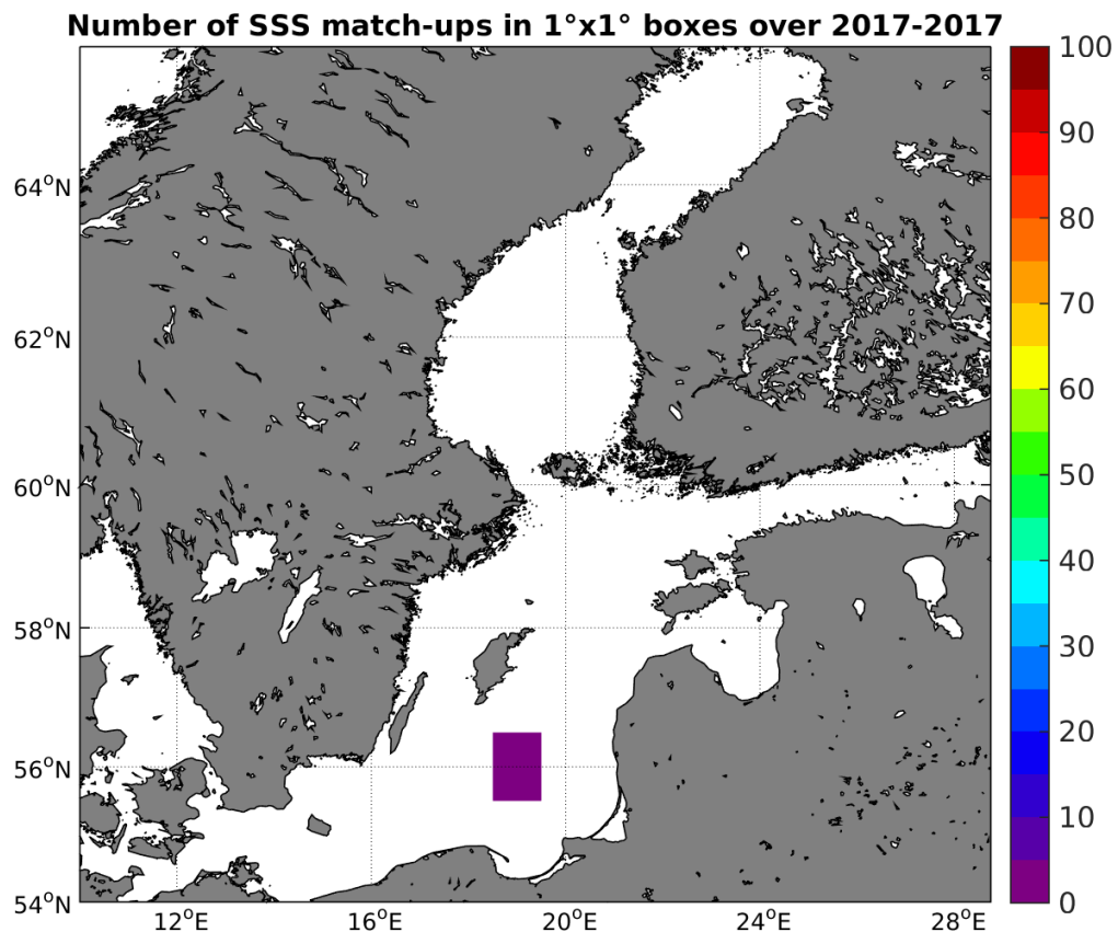
Figure 4: Number of SSS match-ups between Argo SSS and the SMAP-L3-RSS-V2-8DAY-RUNNING-70KM SSS product for the Baltic Sea Pi-MEP region over 1°x1° boxes and for the full satellite product period.
