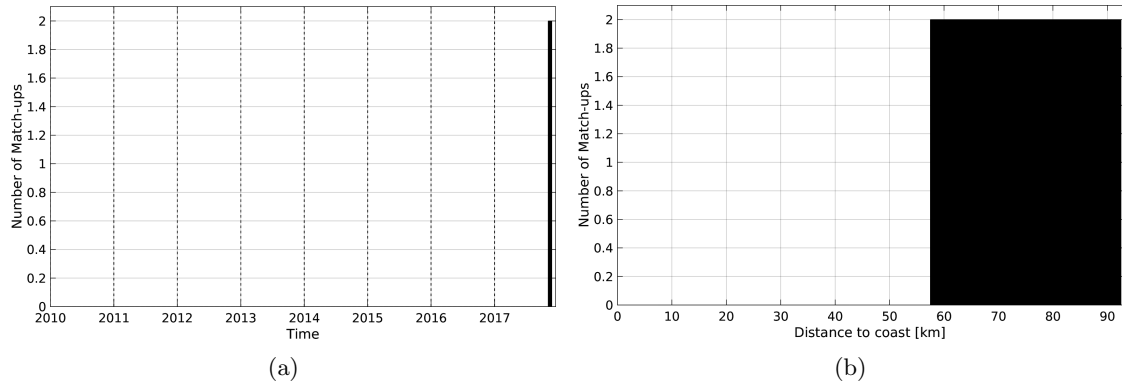
Figure 1: Number of match-ups between Argo and SMAP-L3-RSS-V2-8DAY-RUNNING-70KM SSS as a function of time (a) and as function of the distance to coast (b) over the Baltic Sea Pi-MEP region and for the full satellite product period.
