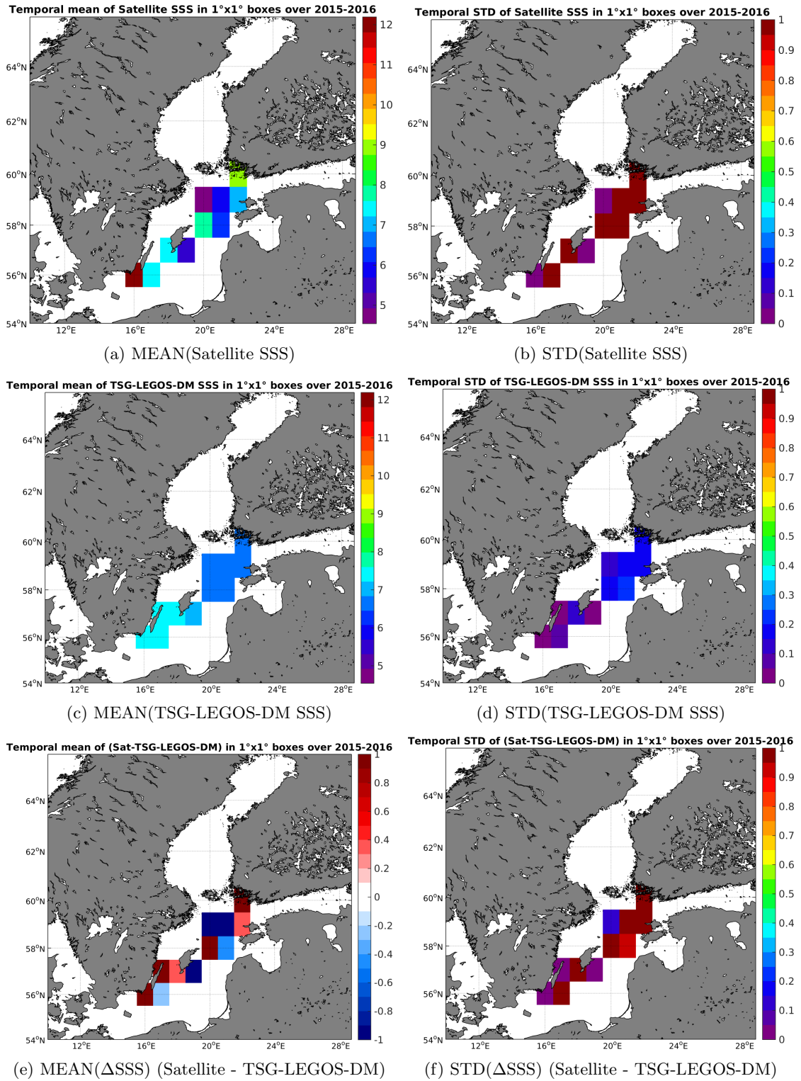
Figure 6: Temporal mean (left) and STD (right) of SSS from SMAP-L3-RSS-V2-MONTHLY-0.25DEG-40KM (top), TSG-LEGOS-DM (middle), and of \Delta SSS (Satellite - TSG-LEGOS-DM). Only match-up pairs are used to generate these maps.
