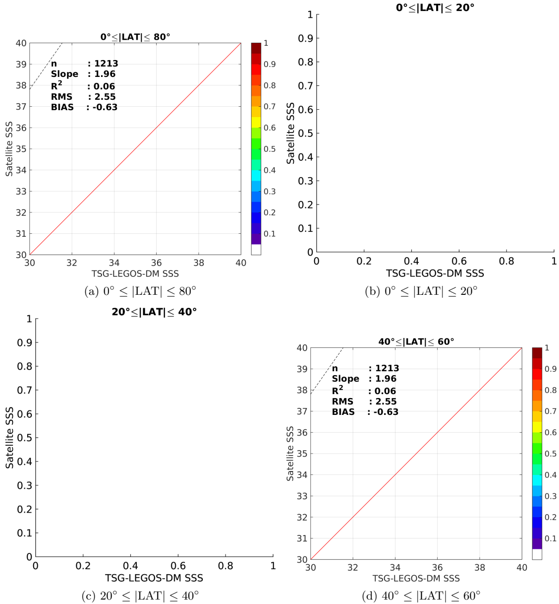
Figure 9: Contour maps of the concentration of SMAP-L3-RSS-V2-MONTHLY-0.25DEG-40KM SSS (y-axis) versus TSG-LEGOS-DM SSS (x-axis) at match-up pairs for different latitude bands. For each plot, the red line shows x=y . The black thin and dashed lines indicate a linear fit through the data cloud and the \pm 95\% confidence levels, respectively. The number match-up pairs n , the slope and R^2 coefficient of the linear fit, the root mean square (RMS) and the mean bias between satellite and in situ data are indicated for each latitude band in each plots.
