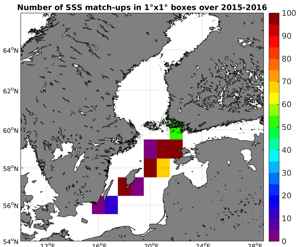
Figure 4: Number of SSS match-ups between TSG-LEGOS-DM SSS and the SMAP-L3-RSS-V2-MONTHLY-0.25DEG-40KM SSS product for the Baltic Sea Pi-MEP region over 1°x1° boxes and for the full satellite product period.
