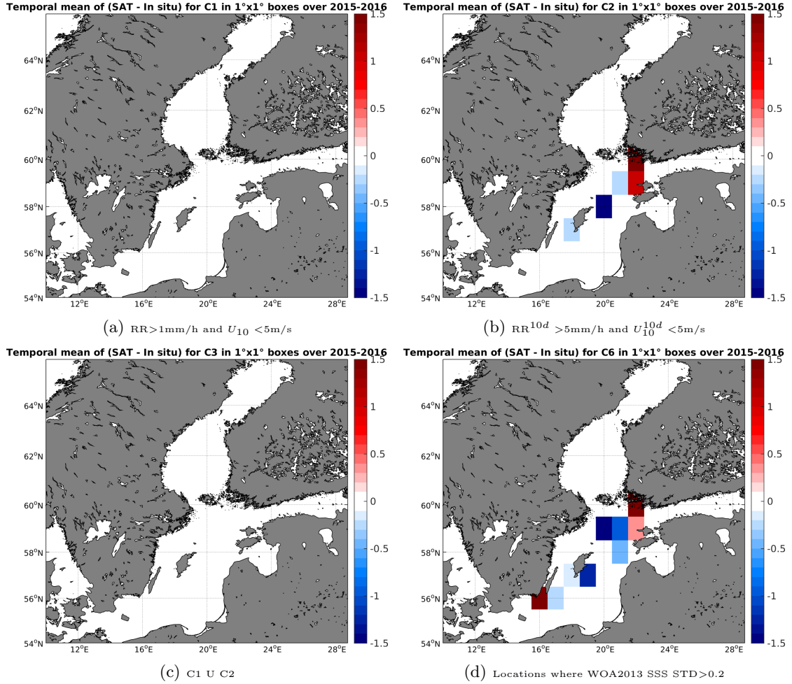
Figure 12: Temporal mean gridded over spatial boxes of size 1°x1° of \Delta SSS (SMAP-L3-RSS-V2-MONTHLY-0.25DEG-40KM - TSG-LEGOS-DM) for 4 different subdatasets corresponding to: RR > 1\text{mm/h} and U_{10} < 5\text{m/s} (a), RR^{10d} > 5\text{mm/h} and U_{10}^{10d} < 5\text{m/s} (b), C1 U C2 (c), Locations where WOA2013 SSS STD > 0.2 (d).
