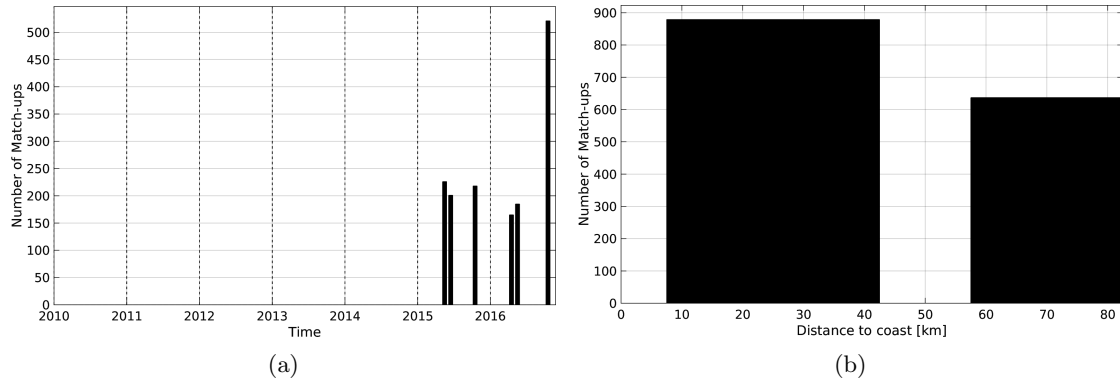
Figure 1: Number of match-ups between TSG-LEGOS-DM and SMAP-L3-RSS-V2-MONTHLY-0.25DEG-40KM SSS as a function of time (a) and as function of the distance to coast (b) over the Baltic Sea Pi-MEP region and for the full satellite product period.
