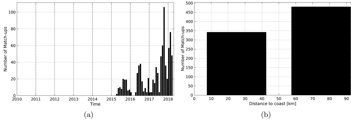
Figure 1: Number of match-ups between Argo and SMAP-L3-RSS-V2-MONTHLY-0.25DEG-40KM SSS as a function of time (a) and as function of the distance to coast (b) over the Baltic Sea Pi-MEP region and for the full satellite product period.
