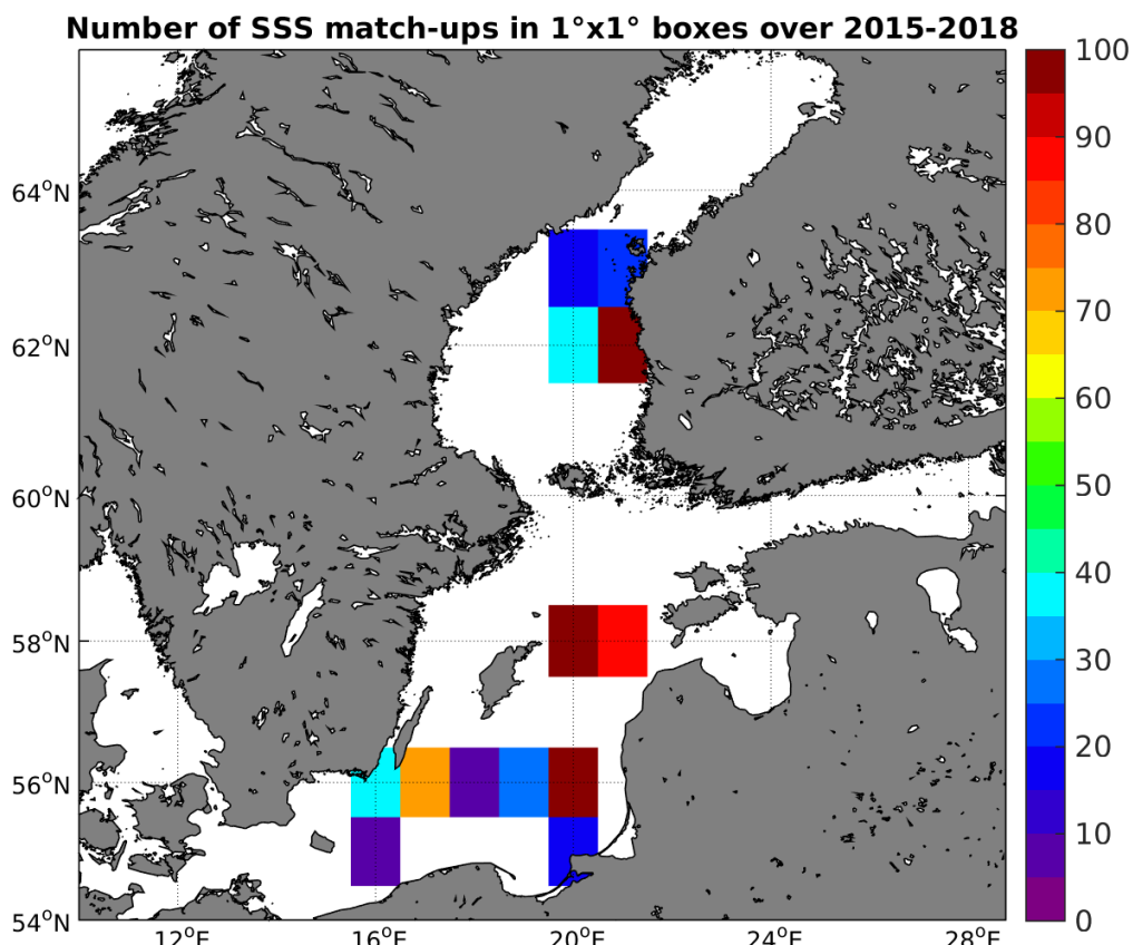
Figure 4: Number of SSS match-ups between Argo SSS and the SMAP-L3-RSS-V2-MONTHLY-0.25DEG-40KM SSS product for the Baltic Sea Pi-MEP region over 1°x1° boxes and for the full satellite product period.
