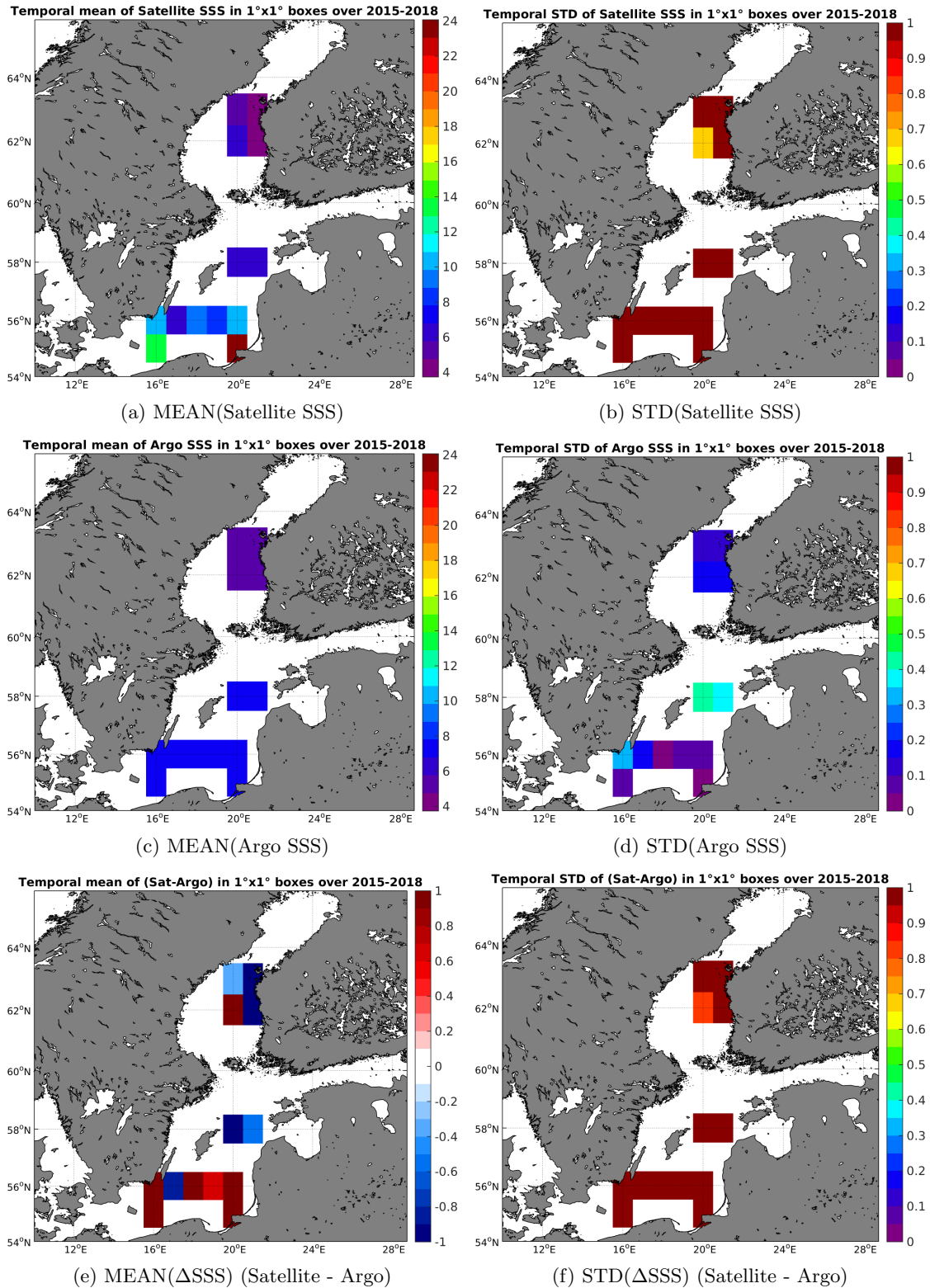
Figure 6: Temporal mean (left) and STD (right) of SSS from SMAP-L3-RSS-V2-MONTHLY-0.25DEG-40KM (top), Argo (middle), and of \Delta SSS (Satellite - Argo). Only match-up pairs are used to generate these maps.
