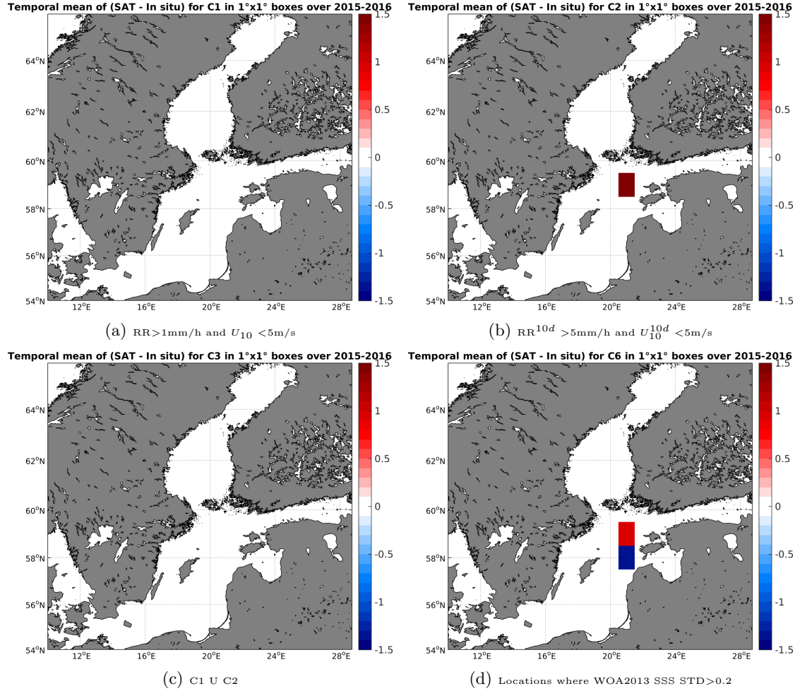
Figure 12: Temporal mean gridded over spatial boxes of size 1^\circ \times 1^\circ of \Delta SSS (SMAP-L3-RSS-V2-MONTHLY-70KM - TSG-LEGOS-DM) for 4 different subdatasets corresponding to: RR > 1mm/h and U_{10} < 5 m/s (a), RR^{10d} > 5 mm/h and U_{10}^{10d} < 5 m/s (b), C1 U C2 (c), Locations where WOA2013 SSS STD > 0.2 (d).
