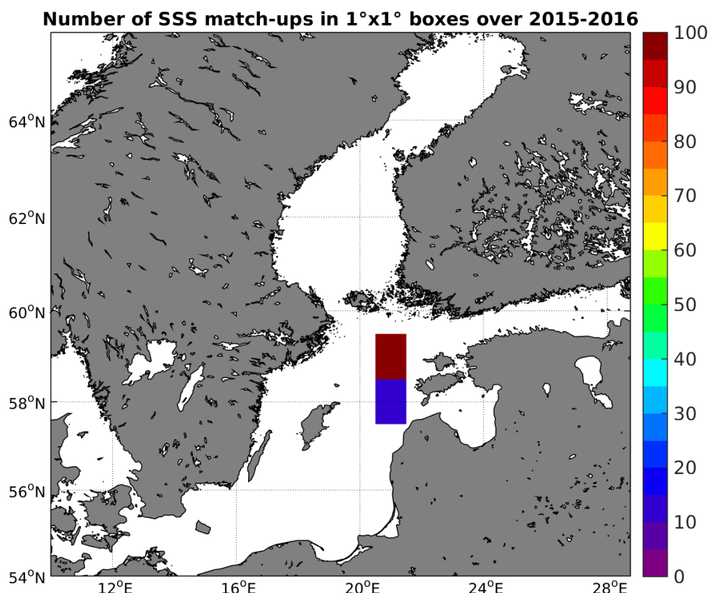
Figure 4: Number of SSS match-ups between TSG-LEGOS-DM SSS and the SMAP-L3-RSS-V2-MONTHLY-70KM SSS product for the Baltic Sea Pi-MEP region over 1°x1° boxes and for the full satellite product period.
