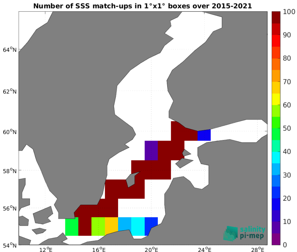
Figure 5: Number of SSS match-ups between TSG (LEGOS-DM) SSS and the SMAP SSS L3 v5.0 - 8-Day running (JPL) SSS product for the Baltic Sea Pi-MEP region over 1^\circ \times 1^\circ boxes and for the full satellite product period.
