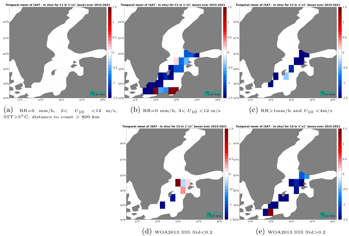
Figure 14: Temporal mean gridded over spatial boxes of size 1^\circ \times 1^\circ of \Delta\text{SSS} (SMAP SSS L3 v5.0 - 8-Day running (JPL) - TSG (LEGOS-DM)) for 5 different subdatasets corresponding to:RR=0 mm/h, 3 < U_{10} < 12 m/s, SST > 5°C, distance to coast > 800 km (a), RR=0 mm/h, 3 < U_{10} < 12 m/s (b), RR > 1mm/h and U_{10} < 4 m/s (c), WOA2013 SSS Std < 0.2 (d), WOA2013 SSS Std > 0.2 (e).
