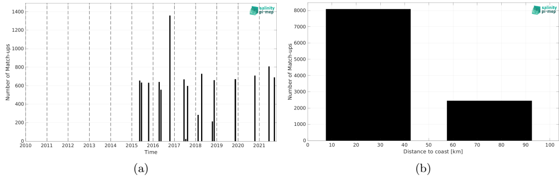
Figure 2: Number of match-ups between TSG (LEGOS-DM) and SMAP SSS L3 v5.0 - 8-Day running (JPL) SSS as a function of time (a) and as function of the distance to coast (b) over the Baltic Sea Pi-MEP region and for the full satellite product period.
