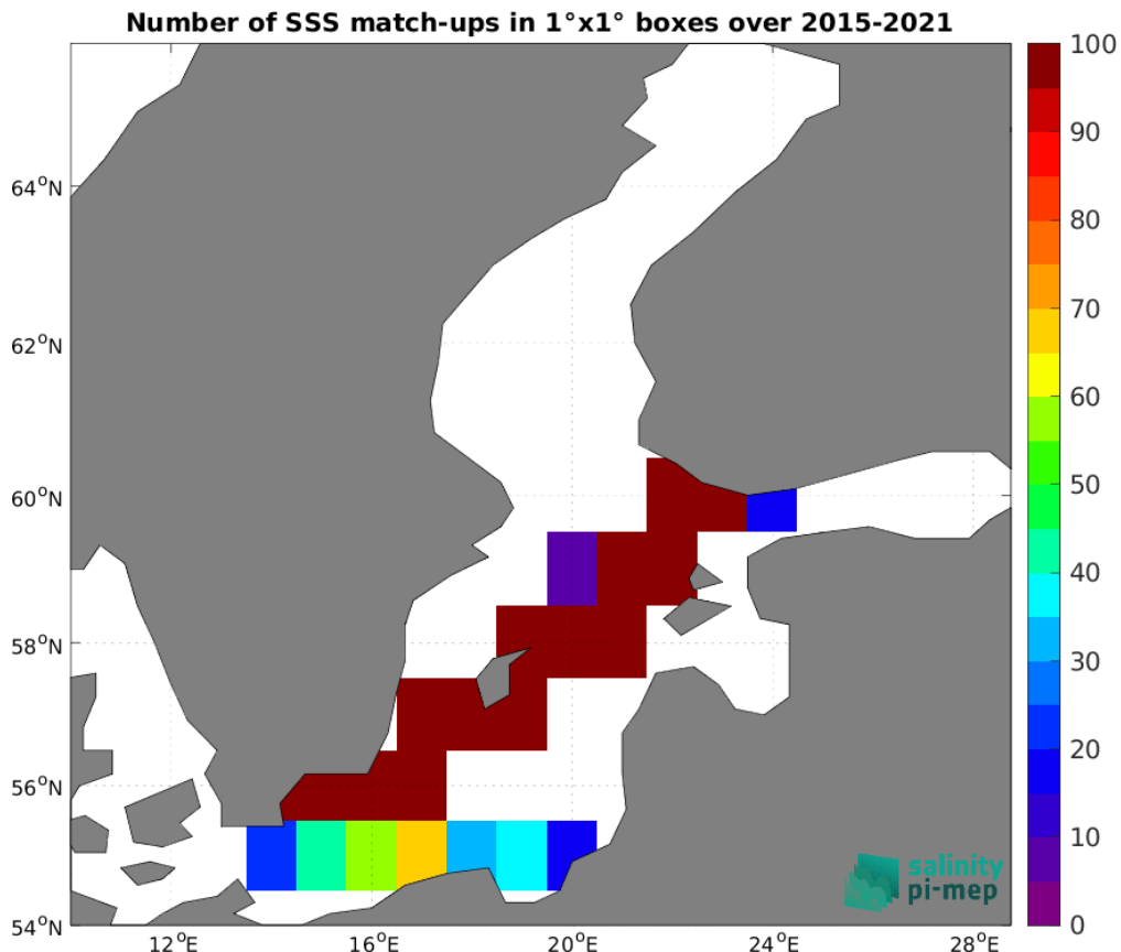
Figure 4: Number of SSS match-ups between TSG (LEGOS-DM) SSS and the SMAP SSS L3 v5.0 - 8-Day running (JPL) SSS product for the Baltic Sea Pi-MEP region over 1^\circ \times 1^\circ boxes and for the full satellite product period.
