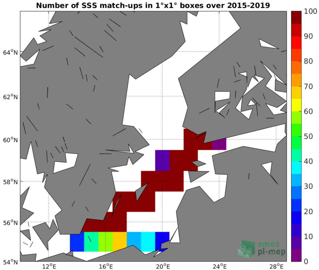
Figure 4: Number of SSS match-ups between TSG (LEGOS-DM) SSS and the SMAP SSS L3 v5.0 - 8-Day running (JPL) SSS product for the Baltic Sea Pi-MEP region over 1^{\circ} \times 1^{\circ} boxes and for the full satellite product period.
