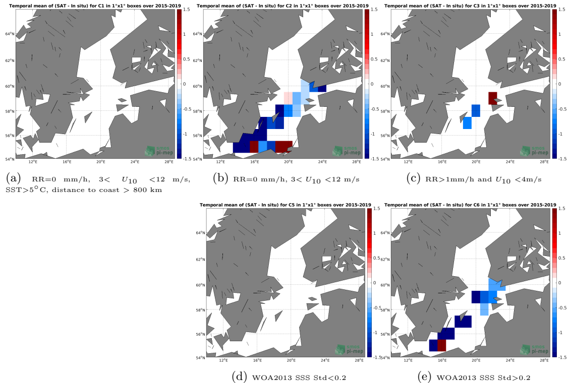
Figure 12: Temporal mean gridded over spatial boxes of size 1^{\circ}\times 1^{\circ} of \Delta\text{SSS} (SMAP SSS L3 v5.0 - 8-Day running (JPL) - TSG (LEGOS-DM)) for 5 different subdatasets corresponding to:RR=0 mm/h, 3 < U_{10} < 12 m/s, SST >5^{\circ}\text{C} , distance to coast > 800 km (a), RR=0 mm/h, 3 < U_{10} < 12 m/s (b), RR >1 mm/h and U_{10} < 4 m/s (c), WOA2013 SSS Std <0.2 (d), WOA2013 SSS Std >0.2 (e).
