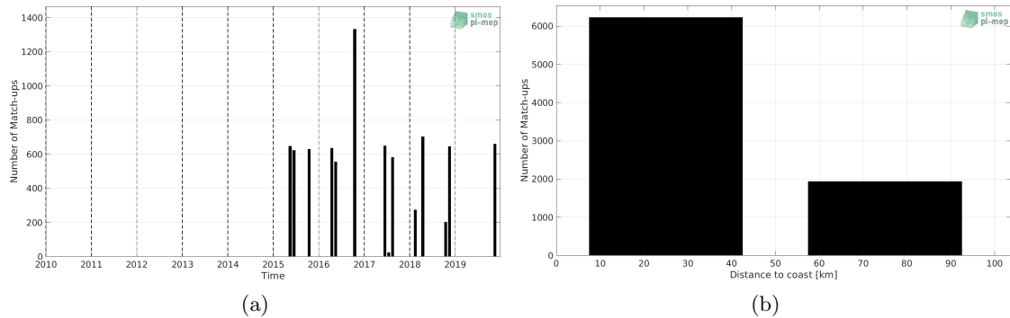
Figure 1: Number of match-ups between TSG (LEGOS-DM) and SMAP SSS L3 v5.0 - 8-Day running (JPL) SSS as a function of time (a) and as function of the distance to coast (b) over the Baltic Sea Pi-MEP region and for the full satellite product period.
