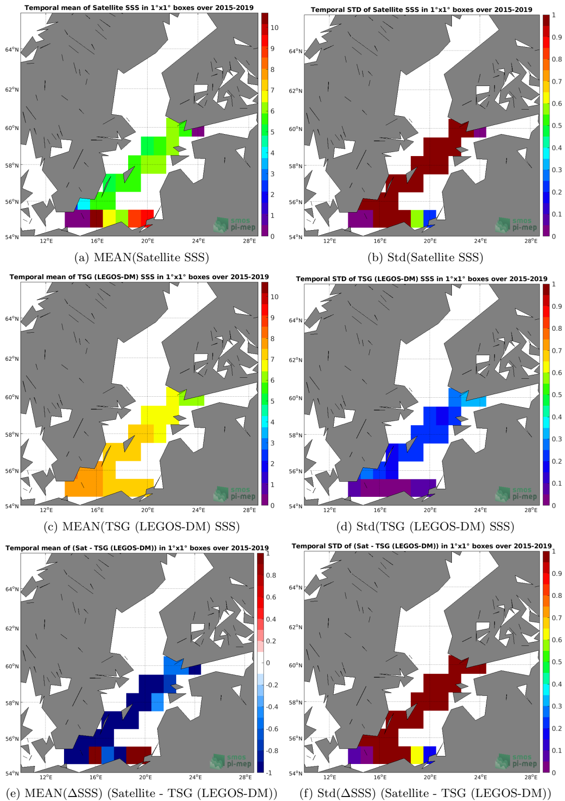
Figure 6: Temporal mean (left) and Std (right) of SSS from SMAP SSS L3 v5.0 - 8-Day running (JPL) (top), TSG (LEGOS-DM) (middle), and \Delta SSS (Satellite - TSG (LEGOS-DM)). Only match-up pairs are used to generate these maps.
