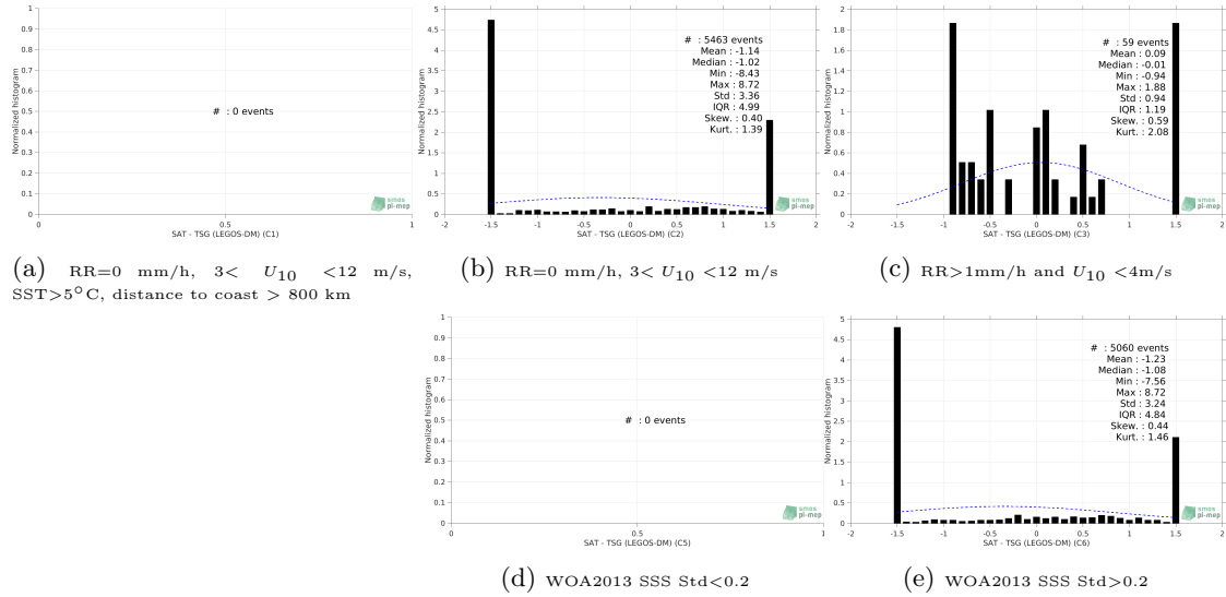
Figure 13: Normalized histogram of \Delta\text{SSS} (SMAP SSS L3 v5.0 - 8-Day running (JPL) - TSG (LEGOS-DM)) for 5 different subdatasets corresponding to: RR=0 mm/h, 3 < U_{10} < 12 m/s, SST > 5^\circ\text{C} , distance to coast > 800 km (a), RR=0 mm/h, 3 < U_{10} < 12 m/s (b), RR > 1\text{mm/h} and U_{10} < 4\text{m/s} (c), WOA2013 SSS \text{Std} < 0.2 (d), WOA2013 SSS \text{Std} > 0.2 (e).
