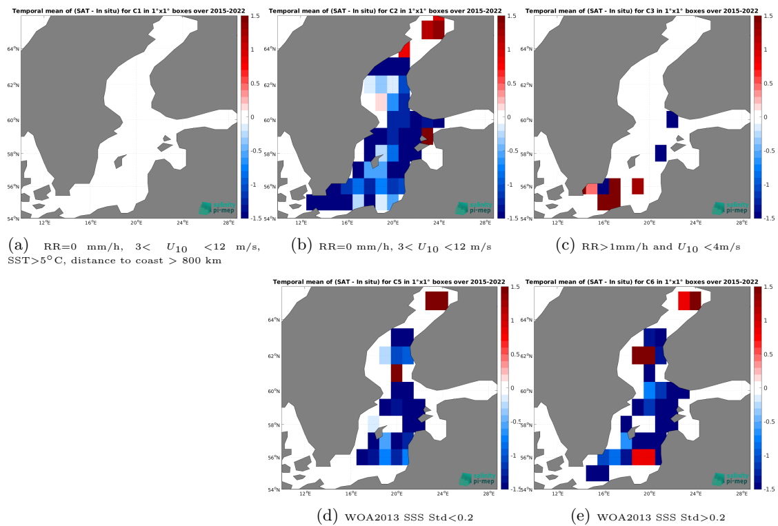
Figure 14: Temporal mean gridded over spatial boxes of size 1^\circ \times 1^\circ of \Delta\text{SSS} (SMAP SSS L3 v5.0 - 8-Day running (JPL) - ICES) for 5 different subdatasets corresponding to:RR=0 mm/h, 3 < U_{10} < 12 m/s, SST >5^\circ\text{C} , distance to coast > 800 km (a), RR=0 mm/h, 3 < U_{10} < 12 m/s (b), RR >1 mm/h and U_{10} < 4 m/s (c), WOA2013 SSS Std <0.2 (d), WOA2013 SSS Std >0.2 (e).
