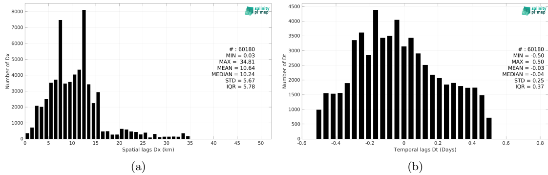
Figure 6: Histograms of the spatial (a) and temporal (b) lags between the location/time of the ICES measurement and the date of the corresponding SMAP SSS L3 v5.0 - 8-Day running (JPL) SSS pixel.
