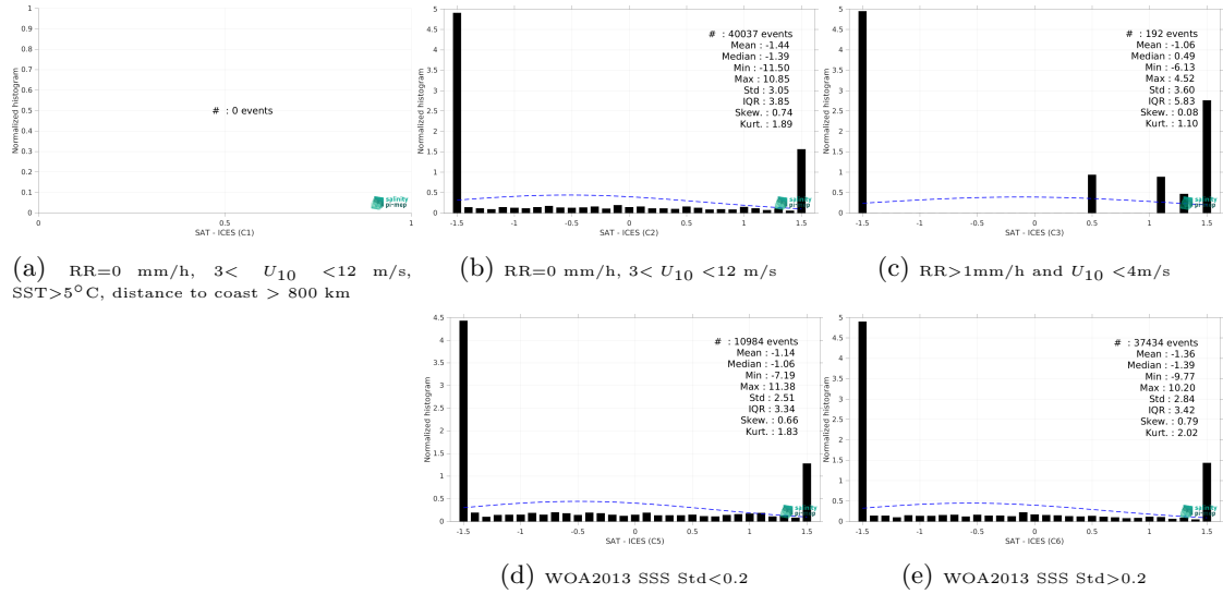
Figure 15: Normalized histogram of \Delta SSS (SMAP SSS L3 v5.0 - 8-Day running (JPL) - ICES) for 5 different subdatasets corresponding to: RR=0 mm/h, 3 < U_{10} < 12 m/s, SST > 5°C, distance to coast > 800 km (a), RR=0 mm/h, 3 < U_{10} < 12 m/s (b), RR > 1mm/h and U_{10} < 4 m/s (c), WOA2013 SSS Std < 0.2 (d), WOA2013 SSS Std > 0.2 (e).
