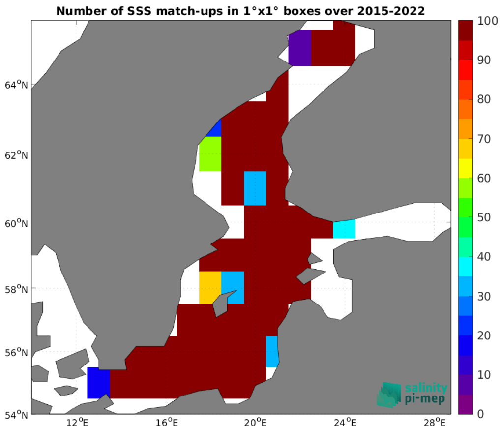
Figure 5: Number of SSS match-ups between ICES SSS and the SMAP SSS L3 v5.0 - 8-Day running (JPL) SSS product for the Baltic Sea Pi-MEP region over 1°×1° boxes and for the full satellite product period.
