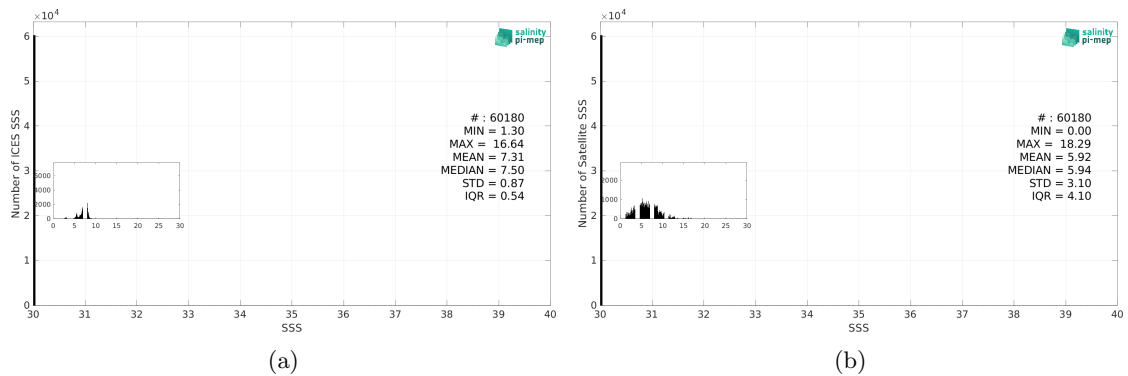
Figure 3: Histograms of SSS from ICES (a) and SMAP SSS L3 v5.0 - 8-Day running (JPL) (b) considering all match-up pairs per bins of 0.1 over the Baltic Sea Pi-MEP region and for the full satellite product period.
