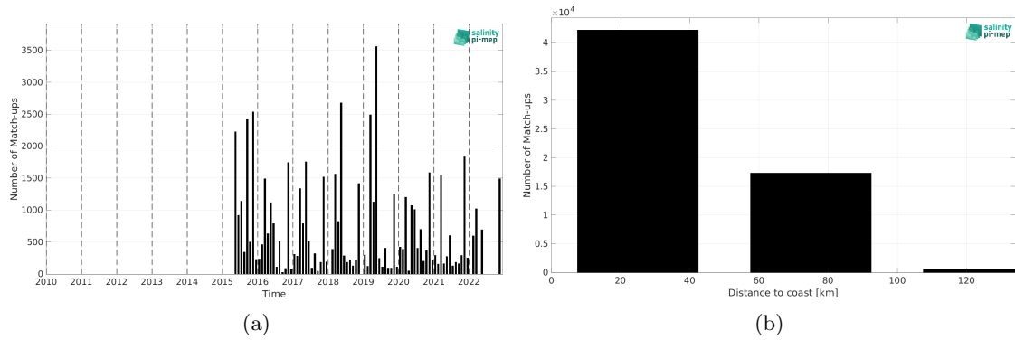
Figure 2: Number of match-ups between ICES and SMAP SSS L3 v5.0 - 8-Day running (JPL) SSS as a function of time (a) and as function of the distance to coast (b) over the Baltic Sea Pi-MEP region and for the full satellite product period.
