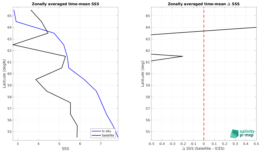
Figure 9: Left panel: Zonal mean SSS from SMAP SSS L3 v5.0 - 8-Day running (JPL) satellite product (black) and from ICES (blue). Right panel: Zonal mean of \Delta SSS (Satellite - ICES) for all the collected Pi-MEP match-up pairs estimated over the full satellite product period.
