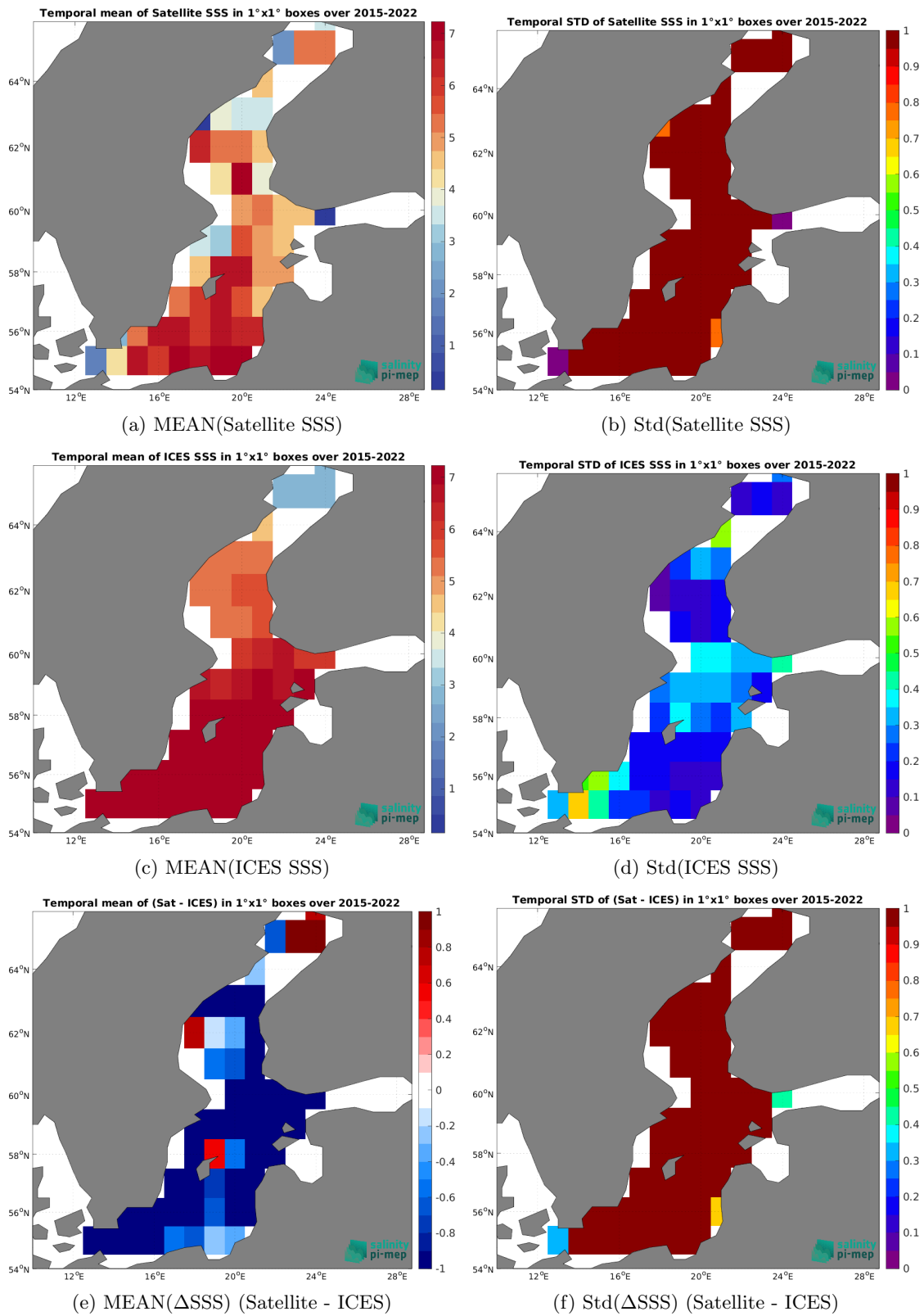
Figure 7: Temporal mean (left) and Std (right) of SSS from SMAP SSS L3 v5.0 - 8-Day running (JPL) (top), ICES (middle), and of \Delta SSS (Satellite - ICES). Only match-up pairs are used to generate these maps.
