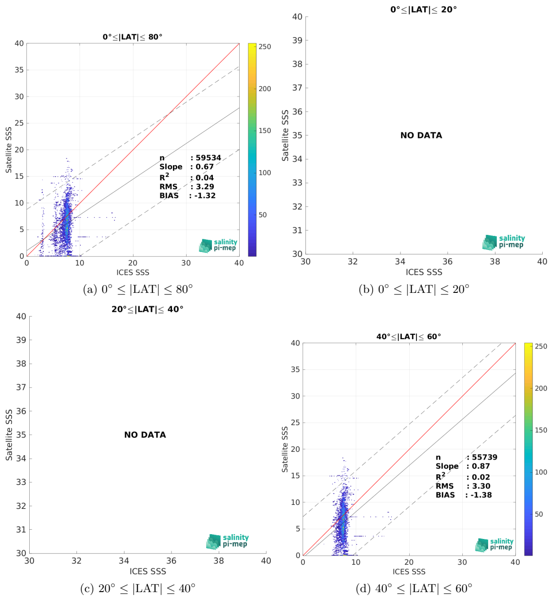
Figure 10: Contour maps of the concentration of SMAP SSS L3 v5.0 - 8-Day running (JPL) SSS (y-axis) versus ICES SSS (x-axis) at match-up pairs for different latitude bands. For each plot, the red line shows x=y . The black thin and dashed lines indicate a linear fit through the data cloud and the \pm 95\% confidence levels, respectively. The number match-up pairs n , the slope and R^2 coefficient of the linear fit, the root mean square (RMS) and the mean bias between satellite and in situ data are indicated for each latitude band in each plots.
