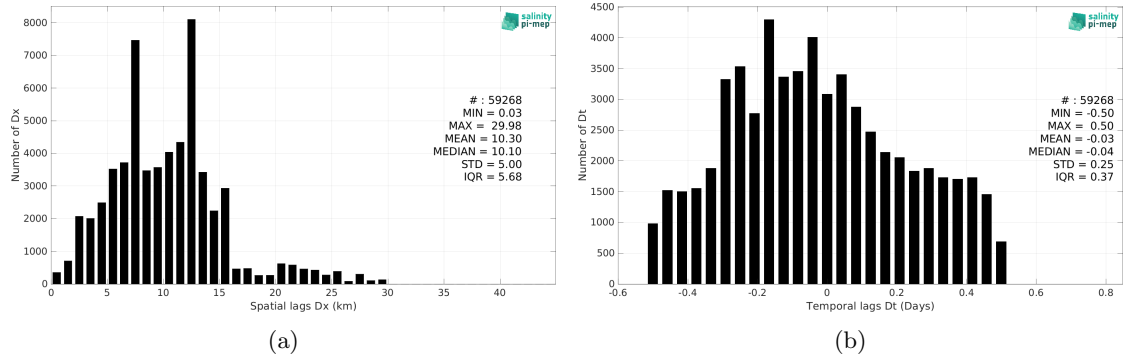
Figure 5: Histograms of the spatial (a) and temporal (b) lags between the location/time of the ICES measurement and the date of the corresponding SMAP SSS L3 v5.0 - 8-Day running (JPL) SSS pixel.
