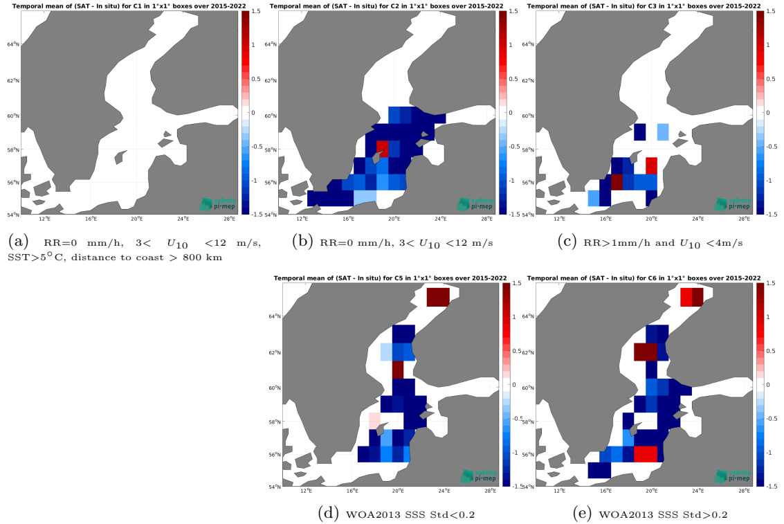
Figure 12: Temporal mean gridded over spatial boxes of size 1^{\circ}\times 1^{\circ} of \Delta\text{SSS} (SMAP SSS L3 v5.0 - 8-Day running (JPL) - ICES) for 5 different subdatasets corresponding to:RR=0 mm/h, 3 < U_{10} < 12 m/s, SST > 5^{\circ}\text{C} , distance to coast > 800 km (a), RR=0 mm/h, 3 < U_{10} < 12 m/s (b), RR > 1 mm/h and U_{10} < 4 m/s (c), WOA2013 SSS Std < 0.2 (d), WOA2013 SSS Std > 0.2 (e).
