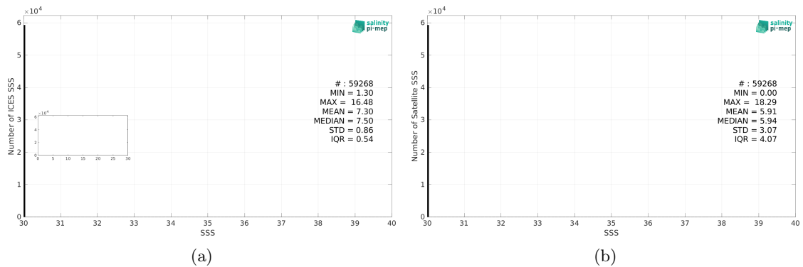
Figure 2: Histograms of SSS from ICES (a) and SMAP SSS L3 v5.0 - 8-Day running (JPL) (b) considering all match-up pairs per bins of 0.1 over the Baltic Sea Pi-MEP region and for the full satellite product period.
