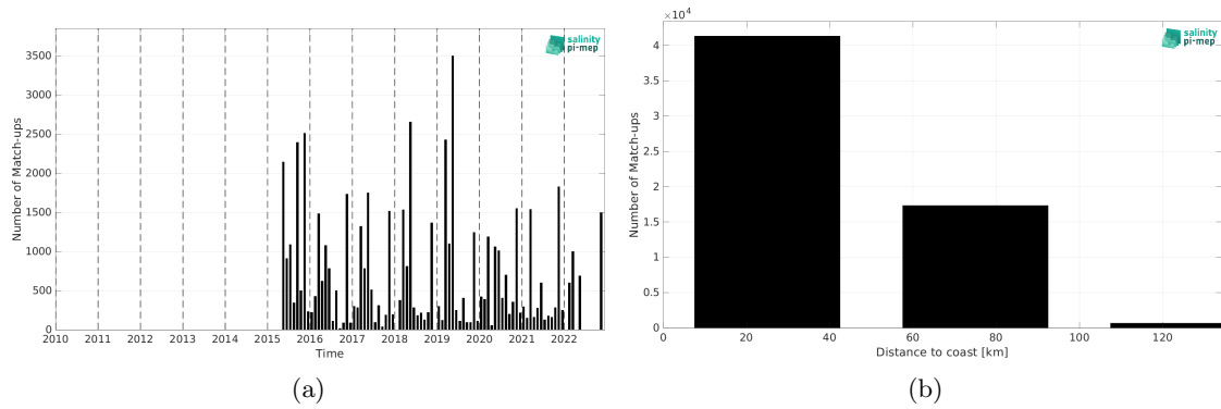
Figure 1: Number of match-ups between ICES and SMAP SSS L3 v5.0 - 8-Day running (JPL) SSS as a function of time (a) and as function of the distance to coast (b) over the Baltic Sea Pi-MEP region and for the full satellite product period.
