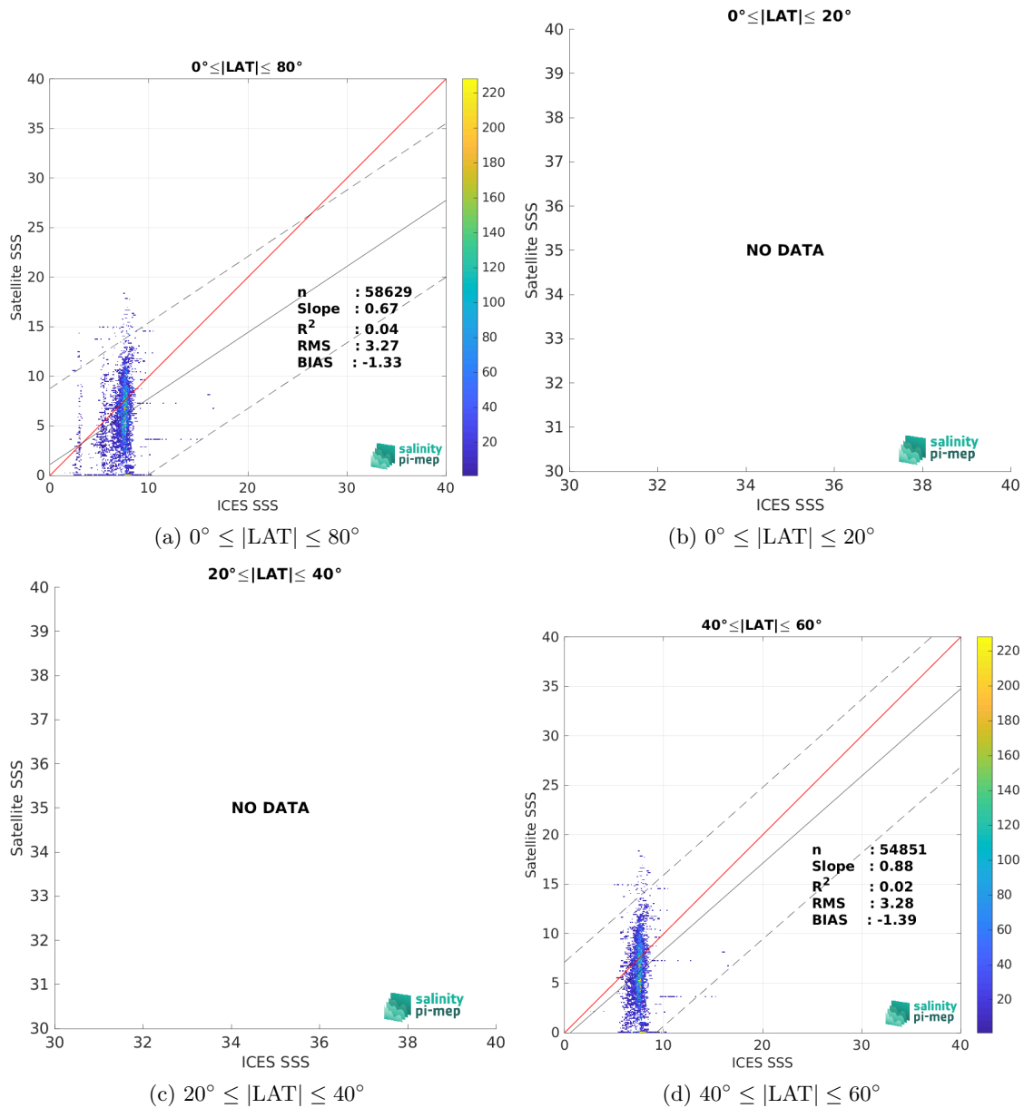
Figure 9: Contour maps of the concentration of SMAP SSS L3 v5.0 - 8-Day running (JPL) SSS (y-axis) versus ICES SSS (x-axis) at match-up pairs for different latitude bands. For each plot, the red line shows x=y . The black thin and dashed lines indicate a linear fit through the data cloud and the \pm 95\% confidence levels, respectively. The number match-up pairs n , the slope and R^2 coefficient of the linear fit, the root mean square (RMS) and the mean bias between satellite and in situ data are indicated for each latitude band in each plots.
