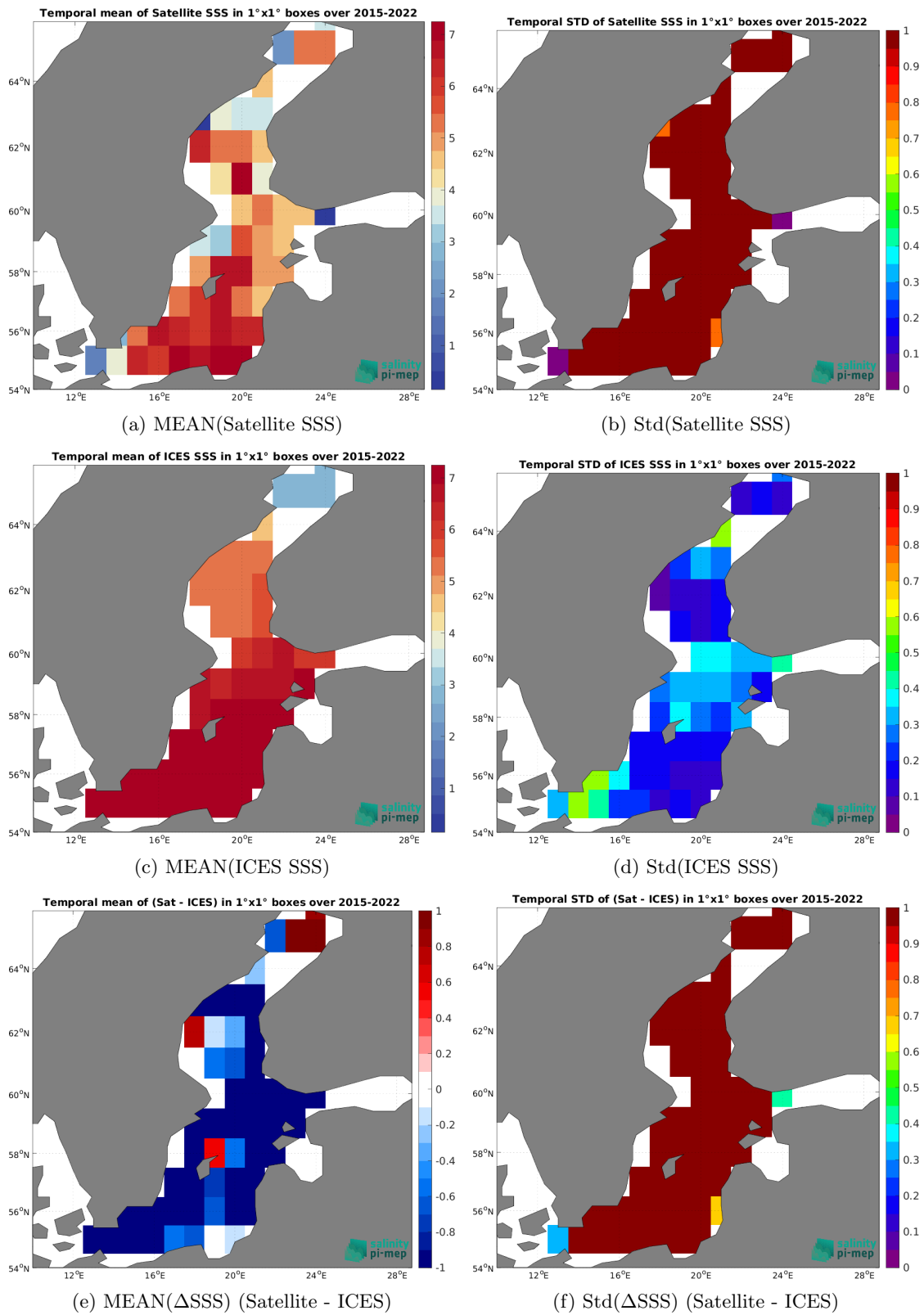
Figure 6: Temporal mean (left) and Std (right) of SSS from SMAP SSS L3 v5.0 - 8-Day running (JPL) (top), ICES (middle), and of \Delta SSS (Satellite - ICES). Only match-up pairs are used to generate these maps.
