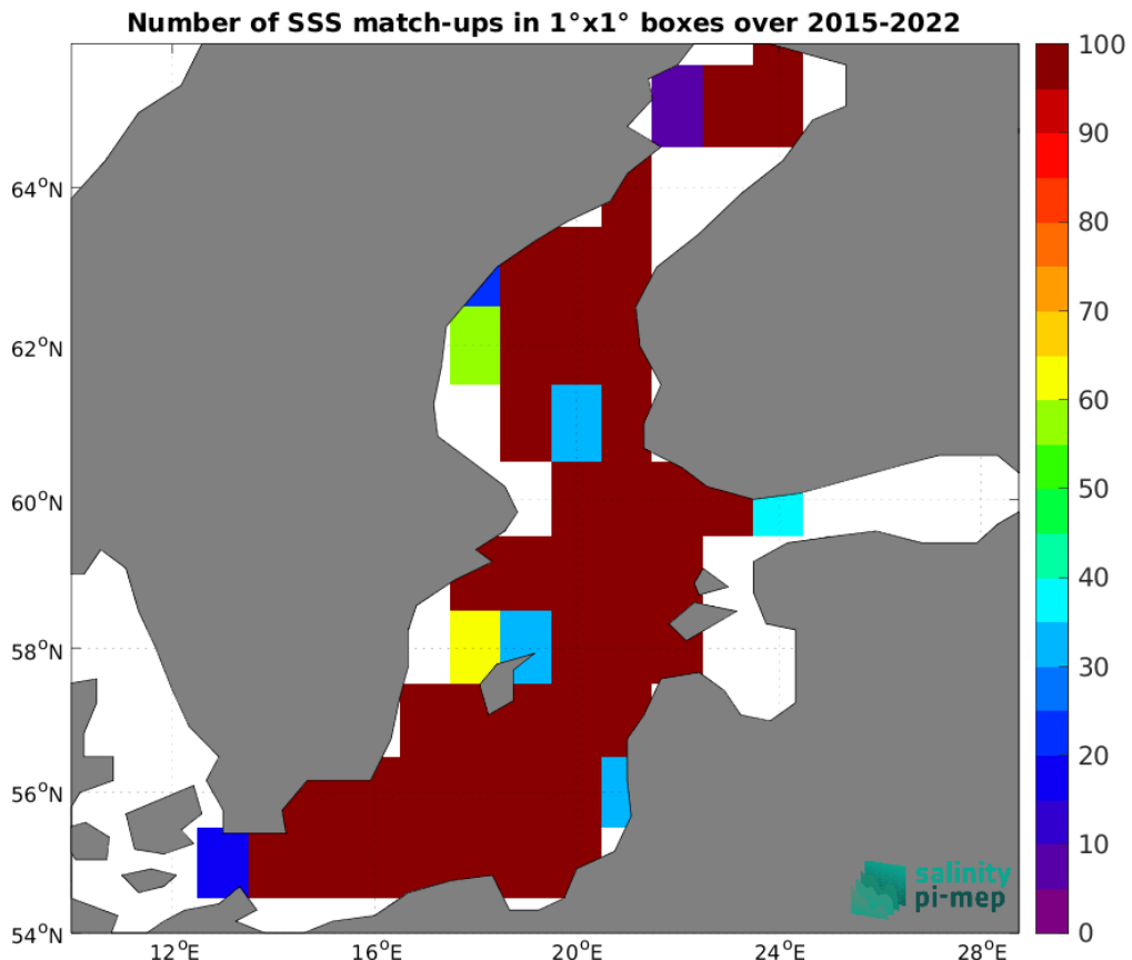
Figure 4: Number of SSS match-ups between ICES SSS and the SMAP SSS L3 v5.0 - 8-Day running (JPL) SSS product for the Baltic Sea Pi-MEP region over 1^\circ \times 1^\circ boxes and for the full satellite product period.
