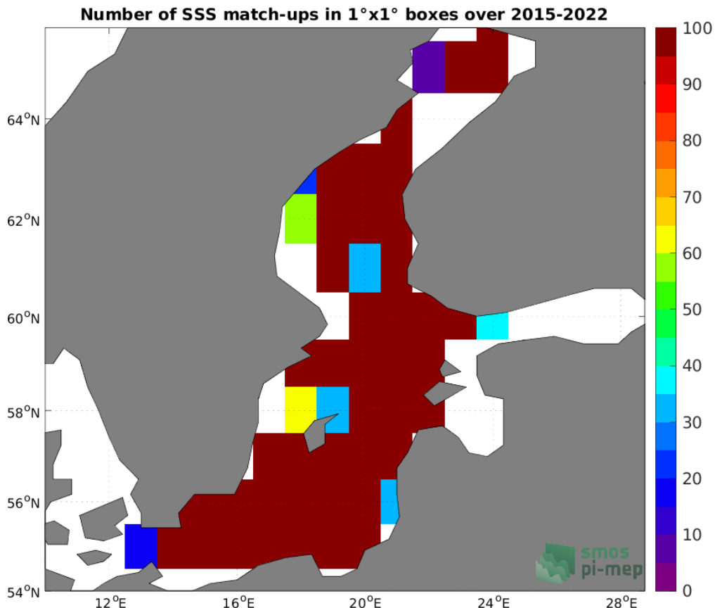
Figure 4: Number of SSS match-ups between ICES SSS and the SMAP SSS L3 v5.0 - 8-Day running (JPL) SSS product for the Baltic Sea Pi-MEP region over 1°×1° boxes and for the full satellite product period.
