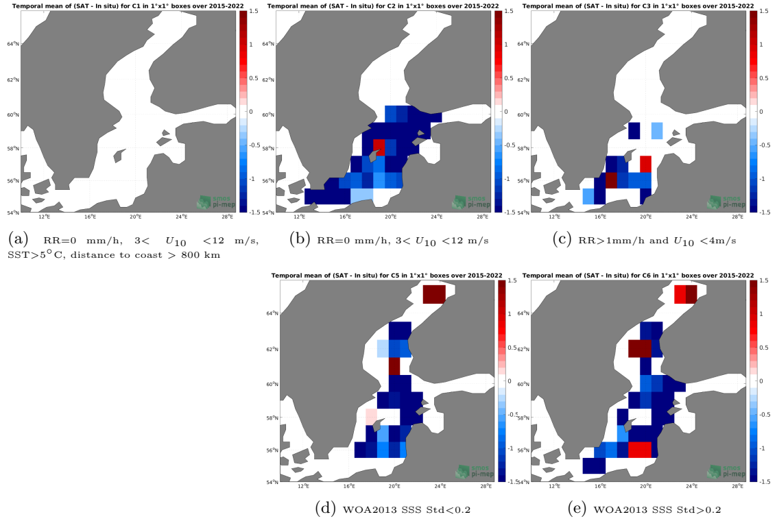
Figure 12: Temporal mean gridded over spatial boxes of size 1^{\circ}\times 1^{\circ} of \Delta\text{SSS} (SMAP SSS L3 v5.0 - 8-Day running (JPL) - ICES) for 5 different subdatasets corresponding to: \text{RR}=0 mm/h, 3 < U_{10} < 12 m/s, \text{SST} > 5^{\circ}\text{C} , distance to coast > 800 km (a), \text{RR}=0 mm/h, 3 < U_{10} < 12 m/s (b), \text{RR} > 1\text{mm/h} and U_{10} < 4\text{m/s} (c), WOA2013 SSS Std < 0.2 (d), WOA2013 SSS Std > 0.2 (e).
