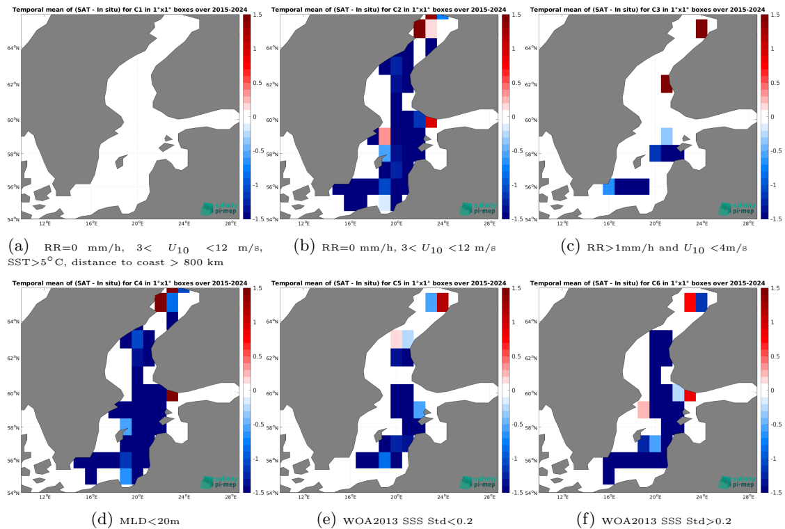
Figure 14: Temporal mean gridded over spatial boxes of size 1^\circ \times 1^\circ of \Delta\text{SSS} (SMAP SSS L3 v5.0 - 8-Day running (JPL) - Argo) for 6 different subdatasets corresponding to:RR=0 mm/h, 3 < U_{10} < 12 m/s, SST>5°C, distance to coast > 800 km (a), RR=0 mm/h, 3 < U_{10} < 12 m/s (b), RR>1mm/h and U_{10} < 4 m/s (c),MLD<20m (d),WOA2013 SSS Std<0.2 (e),WOA2013 SSS Std>0.2 (f).
