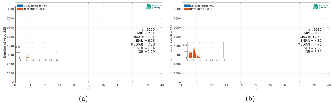
Figure 3: Histograms of SSS from Argo (a) and SMAP SSS L3 v5.0 - 8-Day running (JPL) (b) considering all match-up pairs per bins of 0.1 over the Baltic Sea Pi-MEP region and for the full satellite product period.
