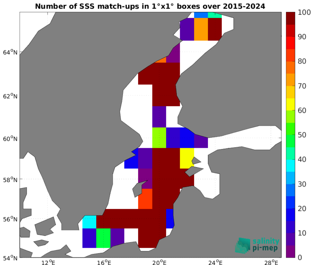
Figure 5: Number of SSS match-ups between Argo SSS and the SMAP SSS L3 v5.0 - 8-Day running (JPL) SSS product for the Baltic Sea Pi-MEP region over 1^\circ \times 1^\circ boxes and for the full satellite product period.
