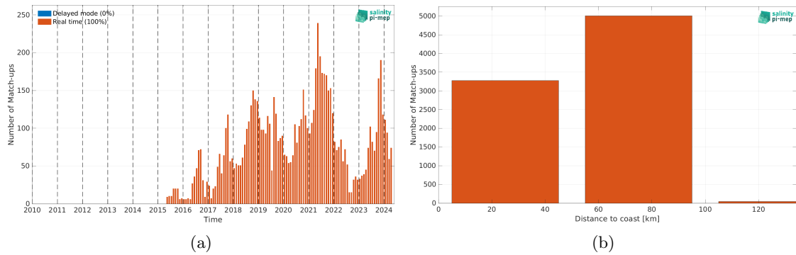
Figure 2: Number of match-ups between Argo and SMAP SSS L3 v5.0 - 8-Day running (JPL) SSS as a function of time (a) and as function of the distance to coast (b) over the Baltic Sea Pi-MEP region and for the full satellite product period.
