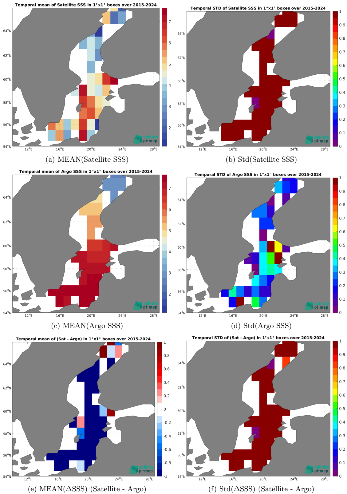
Figure 7: Temporal mean (left) and Std (right) of SSS from SMAP SSS L3 v5.0 - 8-Day running (JPL) (top), Argo (middle), and of \Delta SSS (Satellite - Argo). Only match-up pairs are used to generate these maps.
