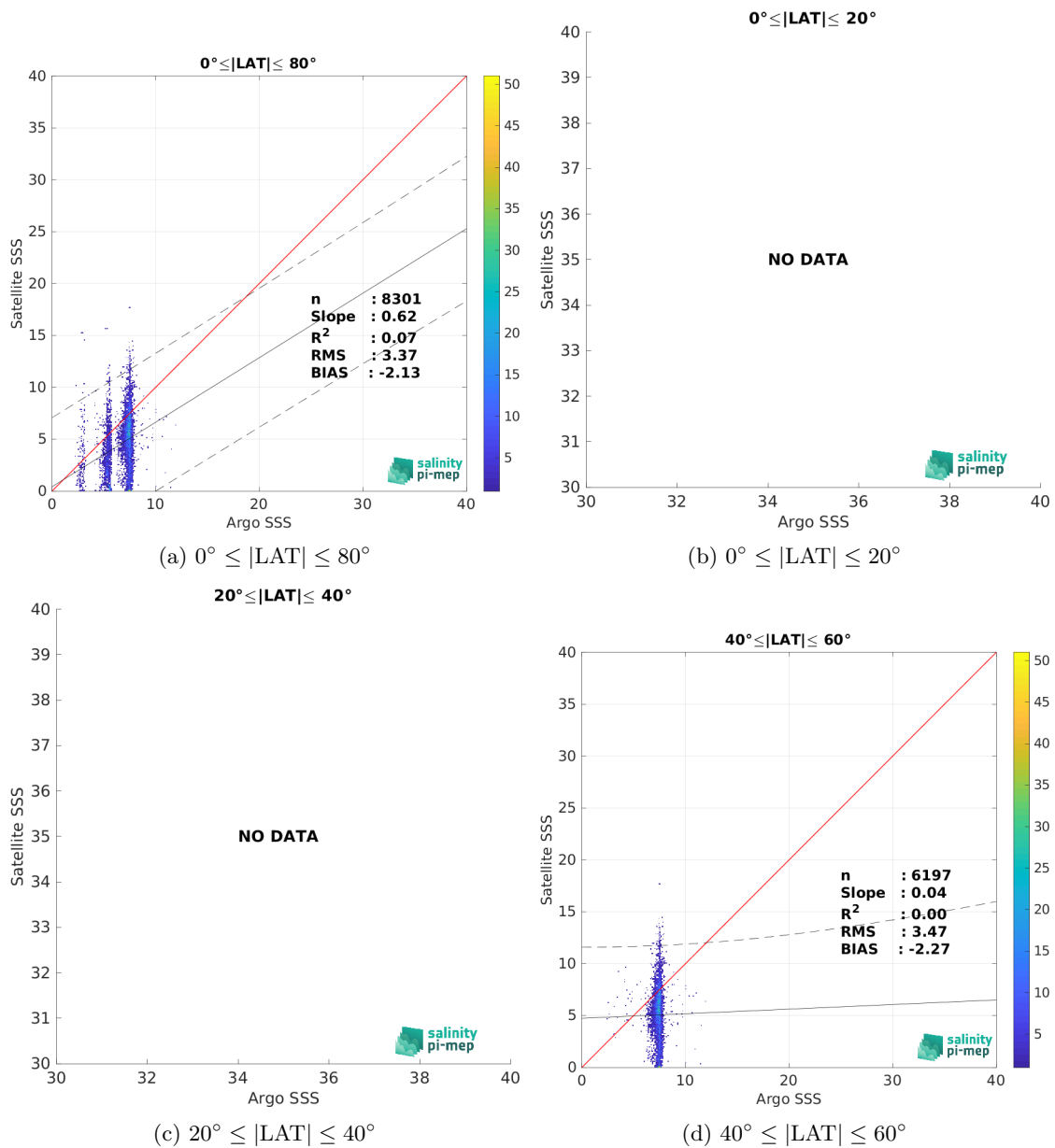
Figure 10: Contour maps of the concentration of SMAP SSS L3 v5.0 - 8-Day running (JPL) SSS (y-axis) versus Argo SSS (x-axis) at match-up pairs for different latitude bands. For each plot, the red line shows x=y . The black thin and dashed lines indicate a linear fit through the data cloud and the \pm 95\% confidence levels, respectively. The number match-up pairs n , the slope and R^2 coefficient of the linear fit, the root mean square (RMS) and the mean bias between satellite and in situ data are indicated for each latitude band in each plot.
