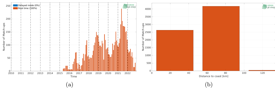
Figure 1: Number of match-ups between Argo and SMAP SSS L3 v5.0 - 8-Day running (JPL) SSS as a function of time (a) and as function of the distance to coast (b) over the Baltic Sea Pi-MEP region and for the full satellite product period.
