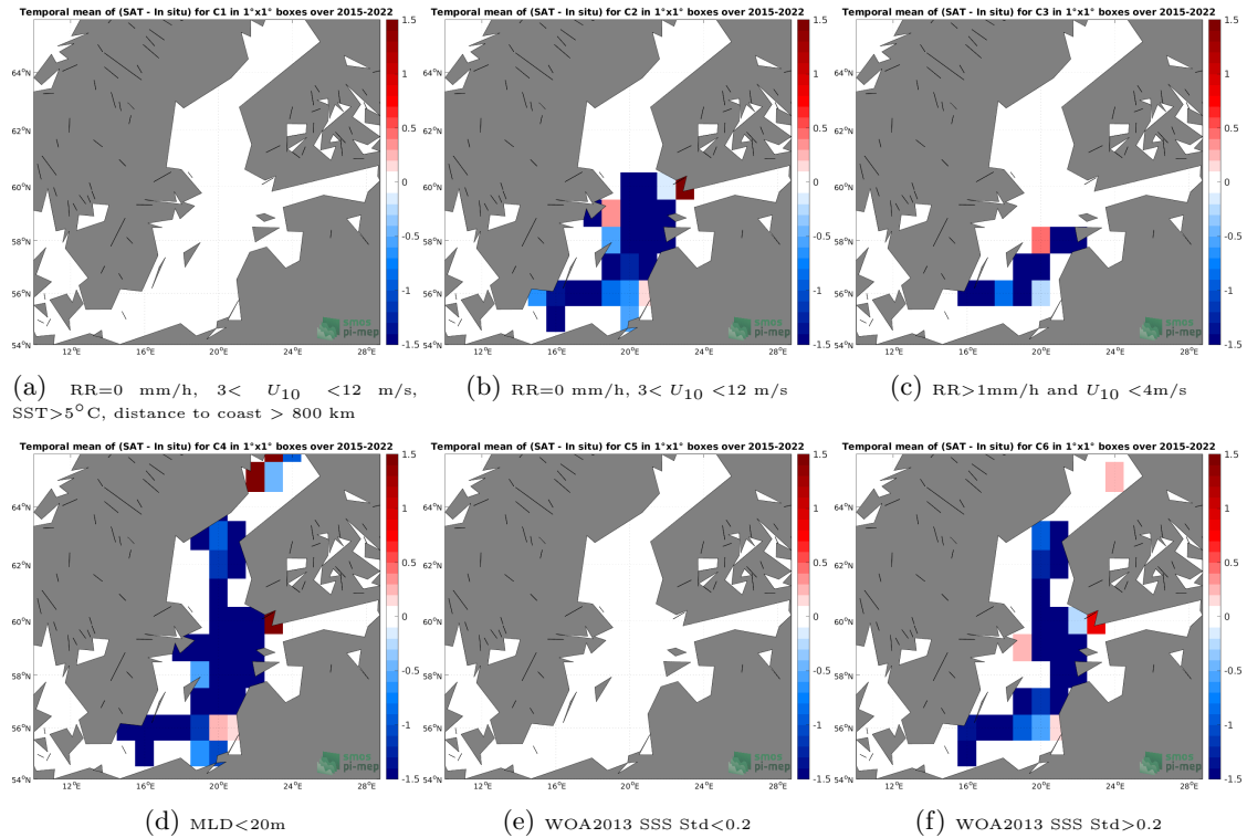
Figure 12: Temporal mean gridded over spatial boxes of size 1^{\circ}\times 1^{\circ} of \Delta\text{SSS} (SMAP SSS L3 v5.0 - 8-Day running (JPL) - Argo) for 6 different subdatasets corresponding to:RR=0 mm/h, 3 < U_{10} < 12 m/s, SST >5^{\circ}\text{C} , distance to coast > 800 km (a), RR=0 mm/h, 3 < U_{10} < 12 m/s (b), RR >1 mm/h and U_{10} < 4 m/s (c),MLD <20 m (d),WOA2013 SSS Std <0.2 (e),WOA2013 SSS Std >0.2 (f).
