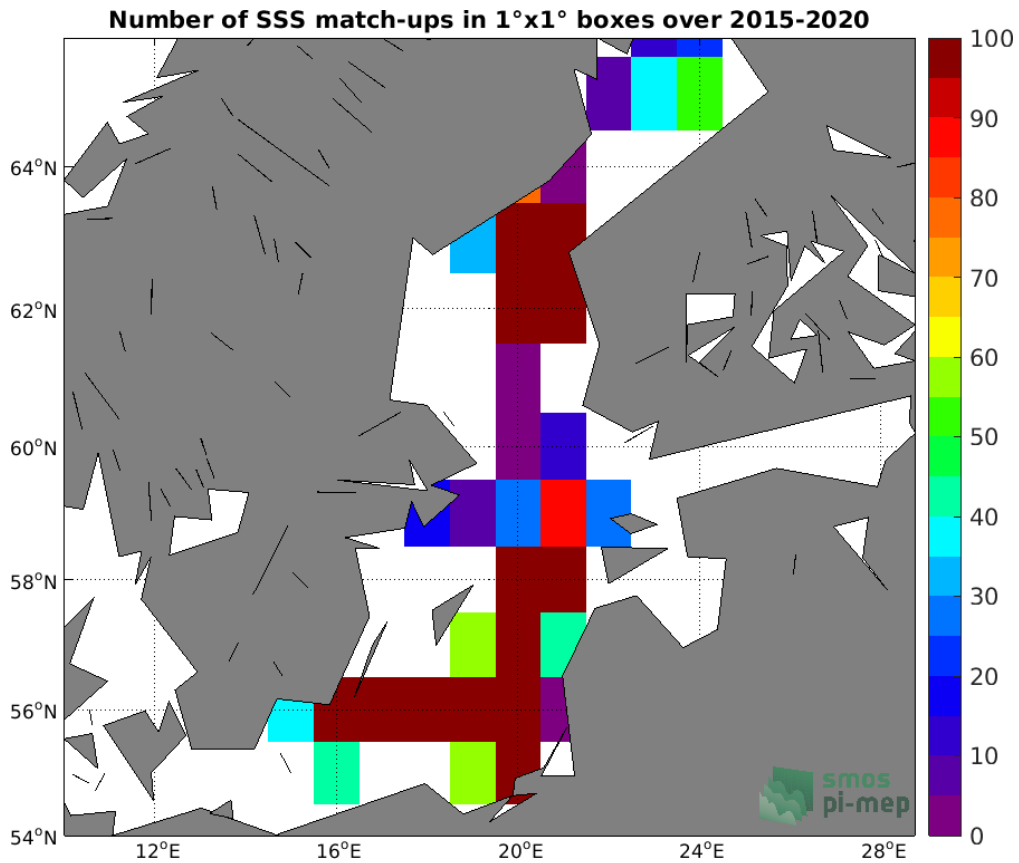
Figure 4: Number of SSS match-ups between Argo SSS and the SMAP SSS L3 v5.0 - 8-Day running (JPL) SSS product for the Baltic Sea Pi-MEP region over 1°x1° boxes and for the full satellite product period.
