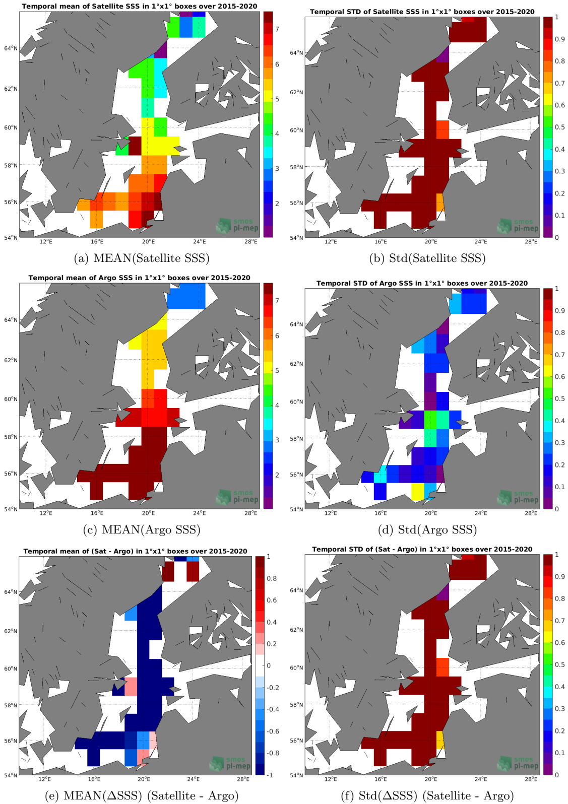
Figure 6: Temporal mean (left) and Std (right) of SSS from SMAP SSS L3 v5.0 - 8-Day running (JPL) (top), Argo (middle), and of \Delta SSS (Satellite - Argo) (bottom). Only match-up pairs are used to generate these maps.
