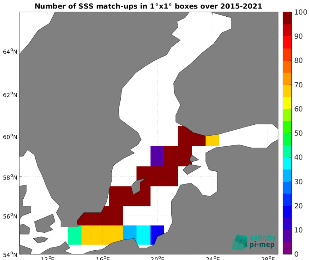
Figure 4: Number of SSS match-ups between TSG (LEGOS-DM) SSS and the SMAP SSS L3 v5.0 - Monthly (JPL) SSS product for the Baltic Sea Pi-MEP region over 1^\circ \times 1^\circ boxes and for the full satellite product period.
