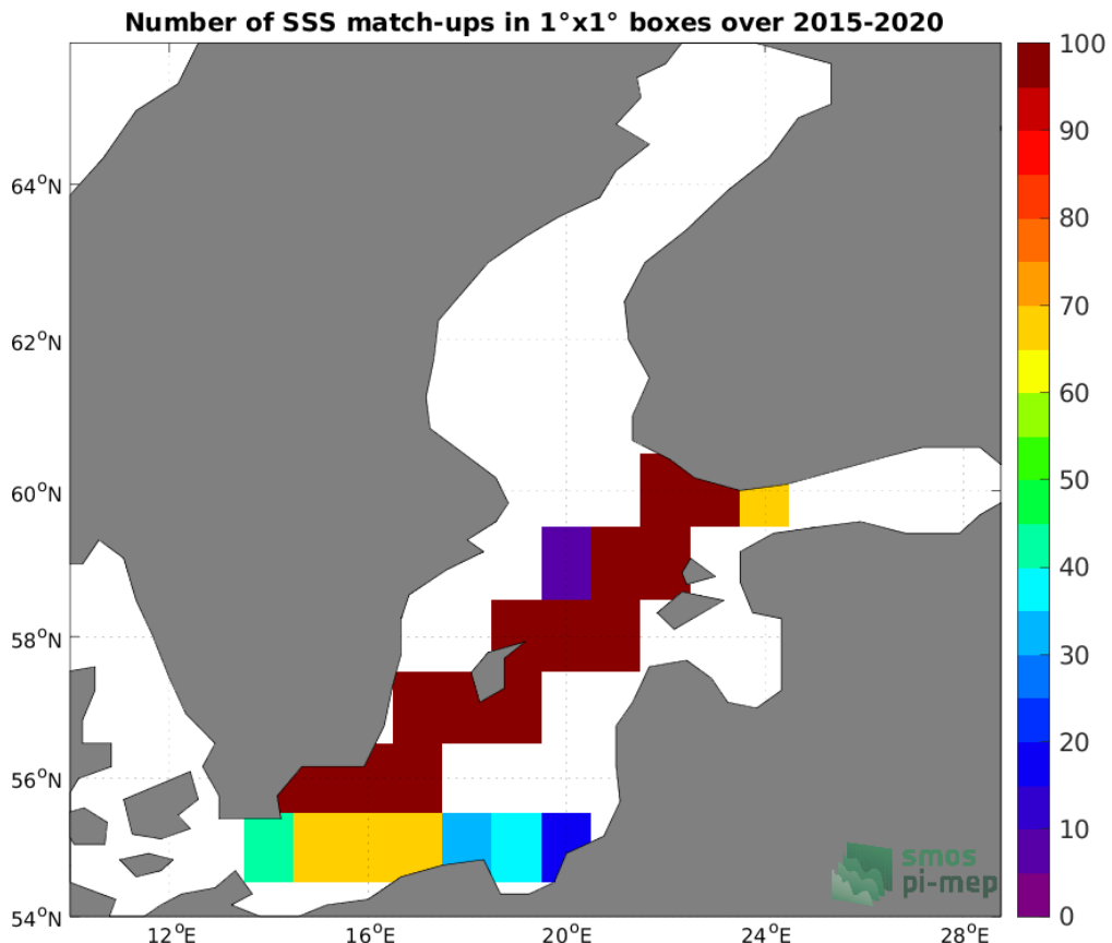
Figure 4: Number of SSS match-ups between TSG (LEGOS-DM) SSS and the SMAP SSS L3 v5.0 - Monthly (JPL) SSS product for the Baltic Sea Pi-MEP region over 1°×1° boxes and for the full satellite product period.
