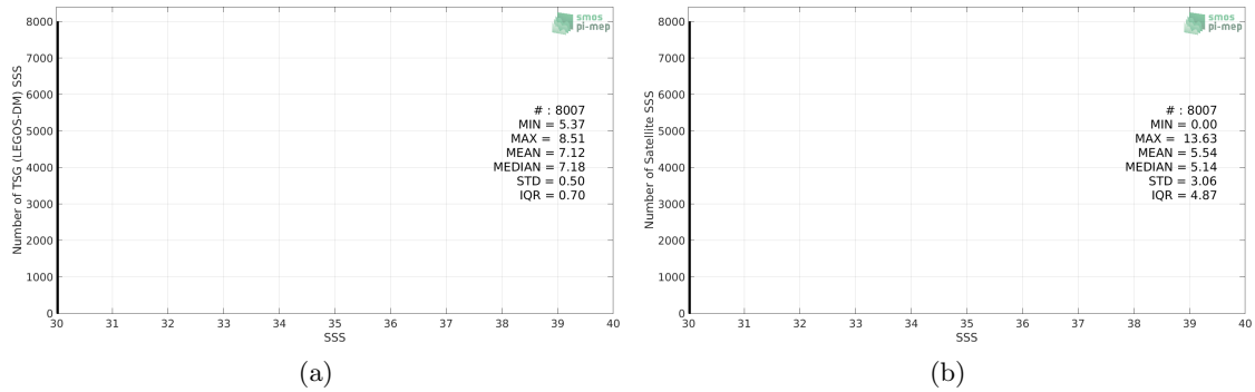
Figure 2: Histograms of SSS from TSG (LEGOS-DM) (a) and SMAP SSS L3 v5.0 - Monthly (JPL) (b) considering all match-up pairs per bins of 0.1 over the Baltic Sea Pi-MEP region and for the full satellite product period.
