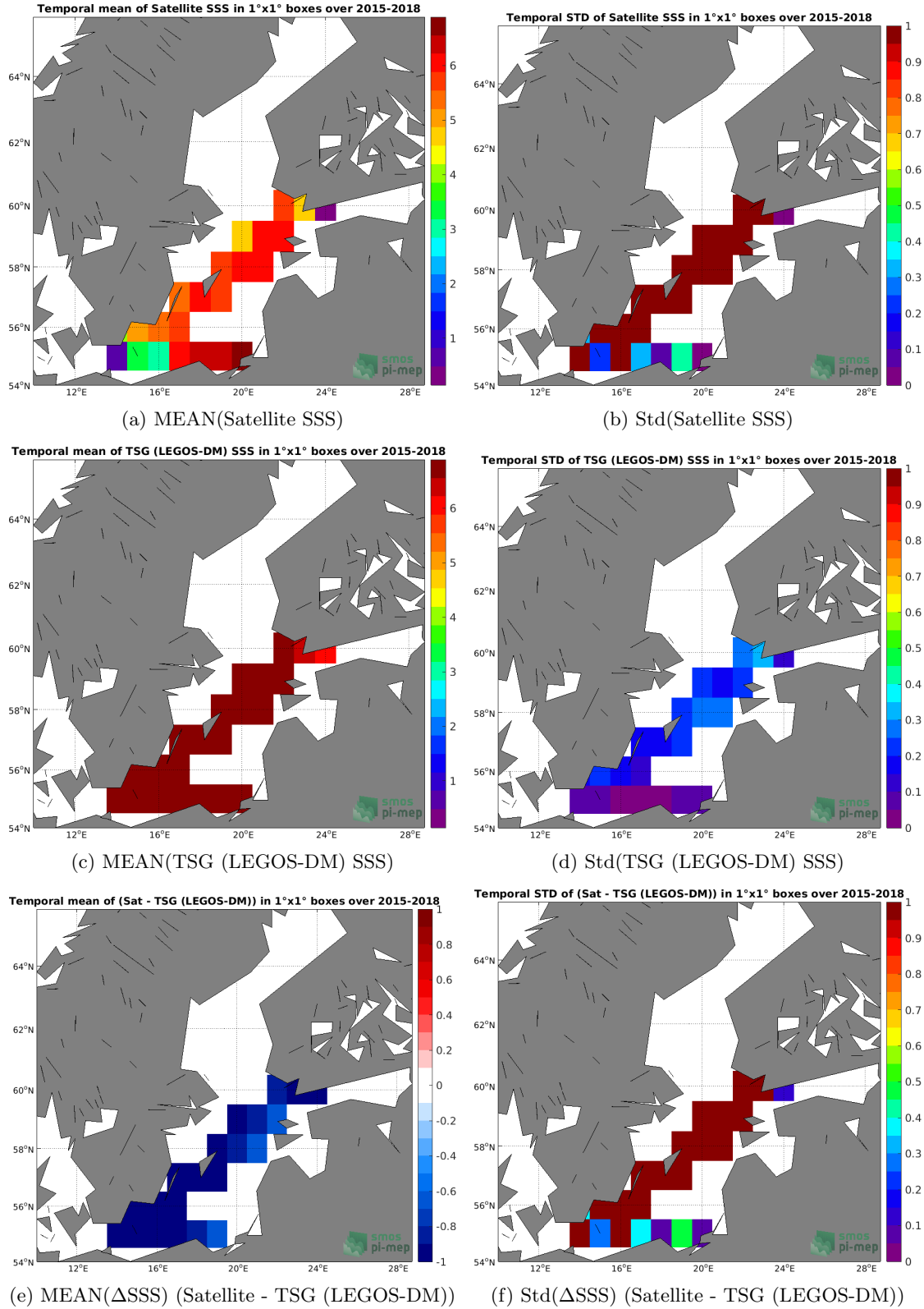
Figure 6: Temporal mean (left) and Std (right) of SSS from SMAP SSS L3 v5.0 - Monthly (JPL) (top), TSG (LEGOS-DM) (middle), and \Delta SSS (Satellite - TSG (LEGOS-DM)). Only match-up pairs are used to generate these maps.
