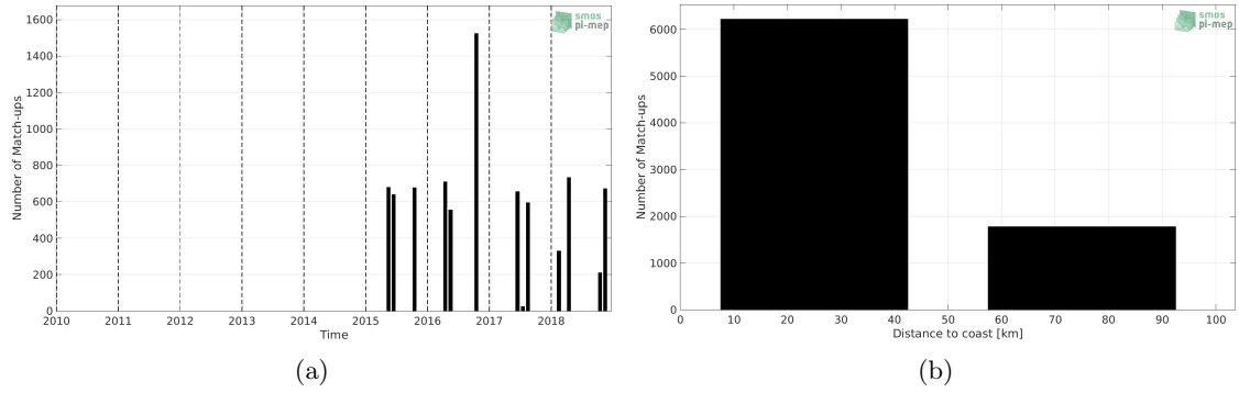
Figure 1: Number of match-ups between TSG (LEGOS-DM) and SMAP SSS L3 v5.0 - Monthly (JPL) SSS as a function of time (a) and as function of the distance to coast (b) over the Baltic Sea Pi-MEP region and for the full satellite product period.
