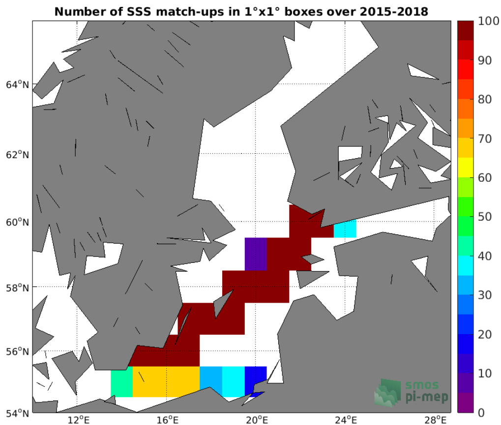
Figure 4: Number of SSS match-ups between TSG (LEGOS-DM) SSS and the SMAP SSS L3 v5.0 - Monthly (JPL) SSS product for the Baltic Sea Pi-MEP region over 1°x1° boxes and for the full satellite product period.
