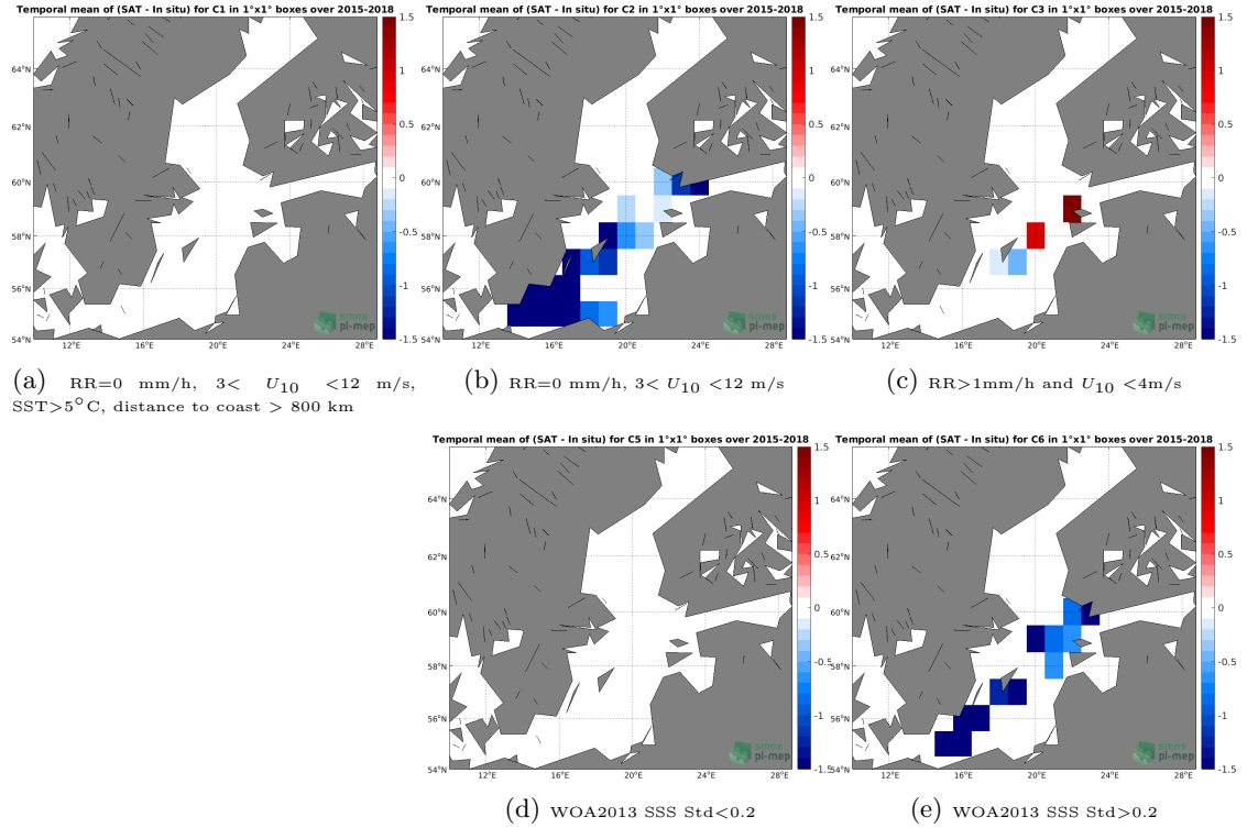
Figure 12: Temporal mean gridded over spatial boxes of size 1^{\circ}\times 1^{\circ} of \Delta\text{SSS} (SMAP SSS L3 v5.0 - Monthly (JPL) - TSG (LEGOS-DM)) for 5 different subdatasets corresponding to:RR=0 mm/h, 3 < U_{10} < 12 m/s, SST >5^{\circ}\text{C} , distance to coast > 800 km (a), RR=0 mm/h, 3 < U_{10} < 12 m/s (b), RR >1 mm/h and U_{10} < 4 m/s (c), WOA2013 SSS Std <0.2 (d), WOA2013 SSS Std >0.2 (e).
