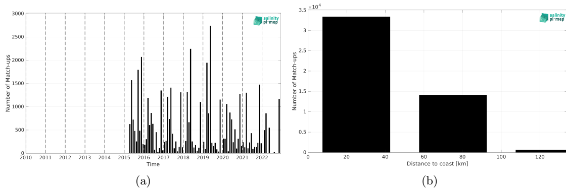
Figure 2: Number of match-ups between ICES and SMAP SSS L3 v5.0 - Monthly (JPL) SSS as a function of time (a) and as function of the distance to coast (b) over the Baltic Sea Pi-MEP region and for the full satellite product period.
