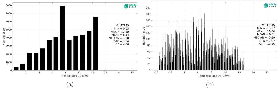
Figure 6: Histograms of the spatial (a) and temporal (b) lags between the location/time of the ICES measurement and the date of the corresponding SMAP SSS L3 v5.0 - Monthly (JPL) SSS pixel.
