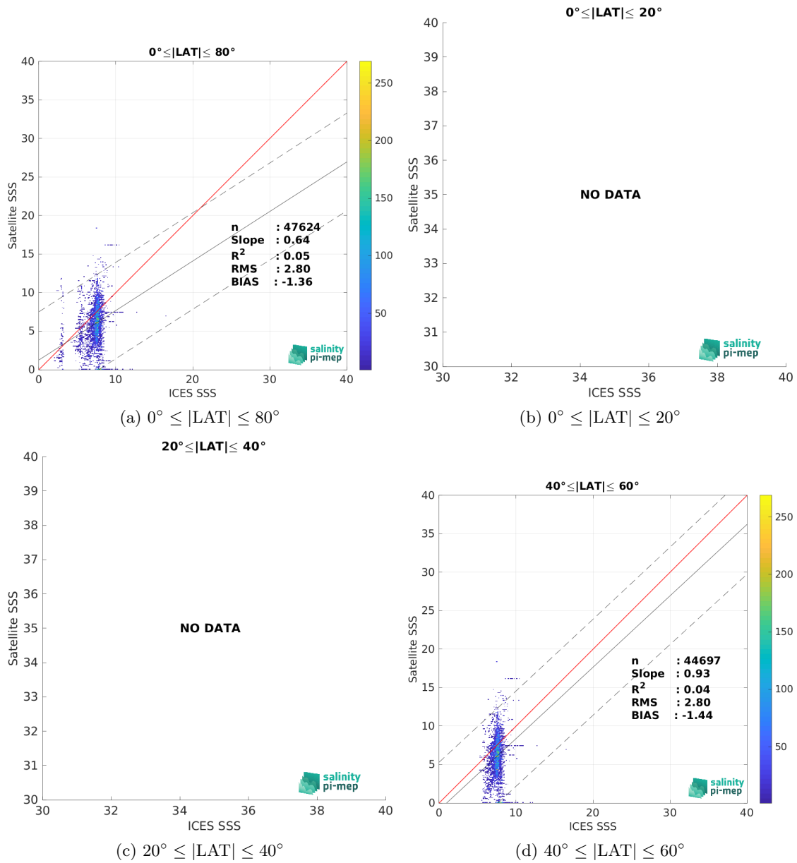
Figure 10: Contour maps of the concentration of SMAP SSS L3 v5.0 - Monthly (JPL) SSS (y-axis) versus ICES SSS (x-axis) at match-up pairs for different latitude bands. For each plot, the red line shows x=y . The black thin and dashed lines indicate a linear fit through the data cloud and the \pm 95\% confidence levels, respectively. The number match-up pairs n , the slope and R^2 coefficient of the linear fit, the root mean square (RMS) and the mean bias between satellite and in situ data are indicated for each latitude band in each plots.
