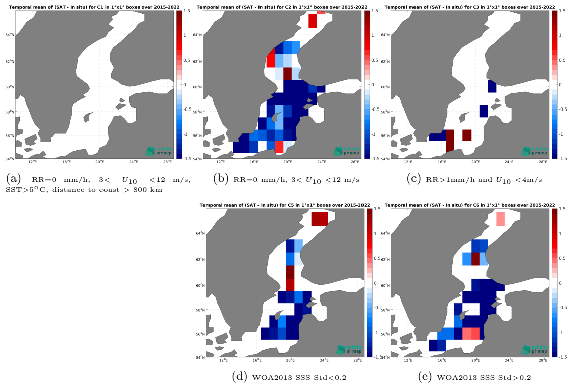
Figure 14: Temporal mean gridded over spatial boxes of size 1^\circ \times 1^\circ of \Delta SSS (SMAP SSS L3 v5.0 - Monthly (JPL) - ICES) for 5 different subdatasets corresponding to:RR=0 mm/h, 3 < U_{10} < 12 m/s, SST >5^\circ C, distance to coast > 800 km (a), RR=0 mm/h, 3 < U_{10} < 12 m/s (b), RR >1 mm/h and U_{10} < 4 m/s (c), WOA2013 SSS Std <0.2 (d), WOA2013 SSS Std >0.2 (e).
