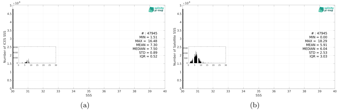
Figure 3: Histograms of SSS from ICES (a) and SMAP SSS L3 v5.0 - Monthly (JPL) (b) considering all match-up pairs per bins of 0.1 over the Baltic Sea Pi-MEP region and for the full satellite product period.
