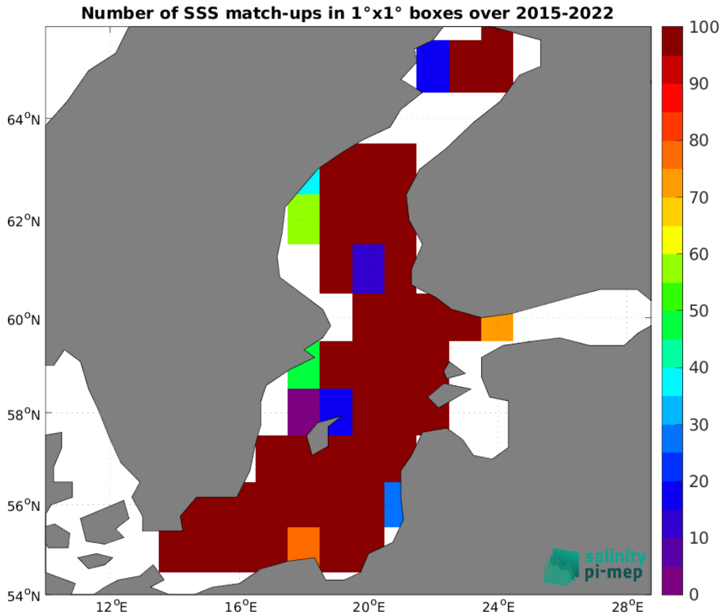
Figure 5: Number of SSS match-ups between ICES SSS and the SMAP SSS L3 v5.0 - Monthly (JPL) SSS product for the Baltic Sea Pi-MEP region over 1^\circ \times 1^\circ boxes and for the full satellite product period.
