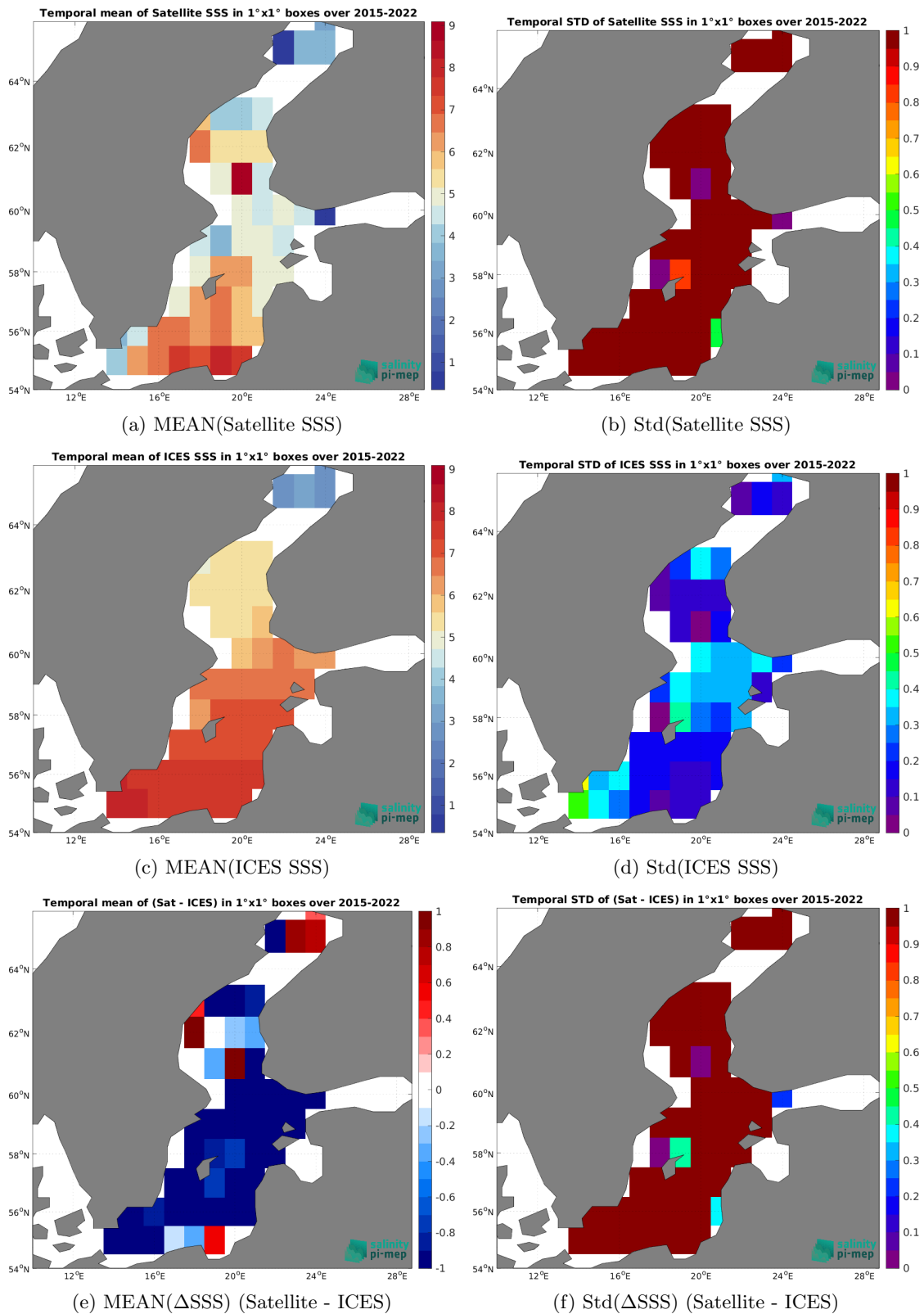
Figure 7: Temporal mean (left) and Std (right) of SSS from SMAP SSS L3 v5.0 - Monthly (JPL) (top), ICES (middle), and of \Delta\text{SSS} (Satellite - ICES). Only match-up pairs are used to generate these maps.
